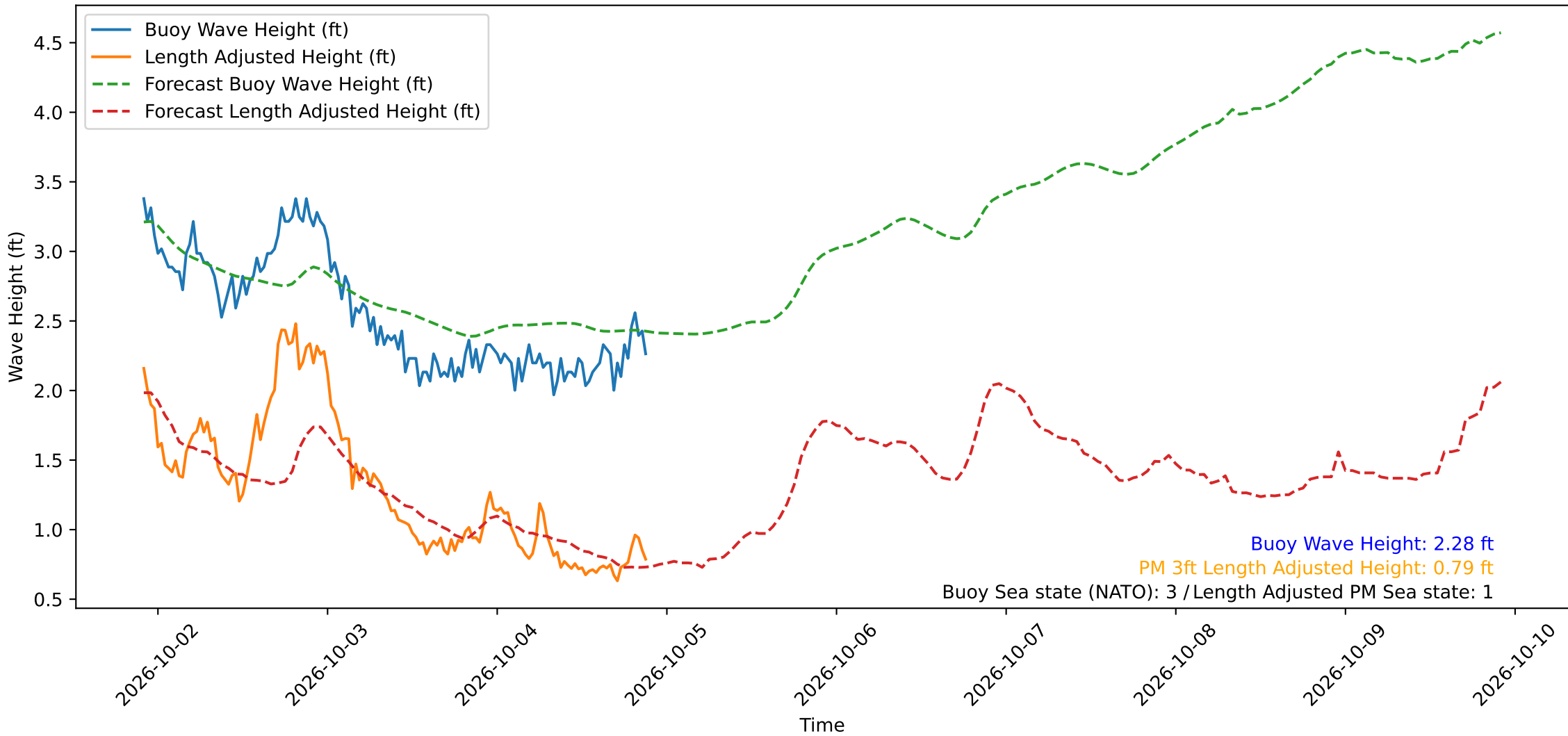
Wave Heights over Time for Green Beach at 2026-10-04 21:41:12
