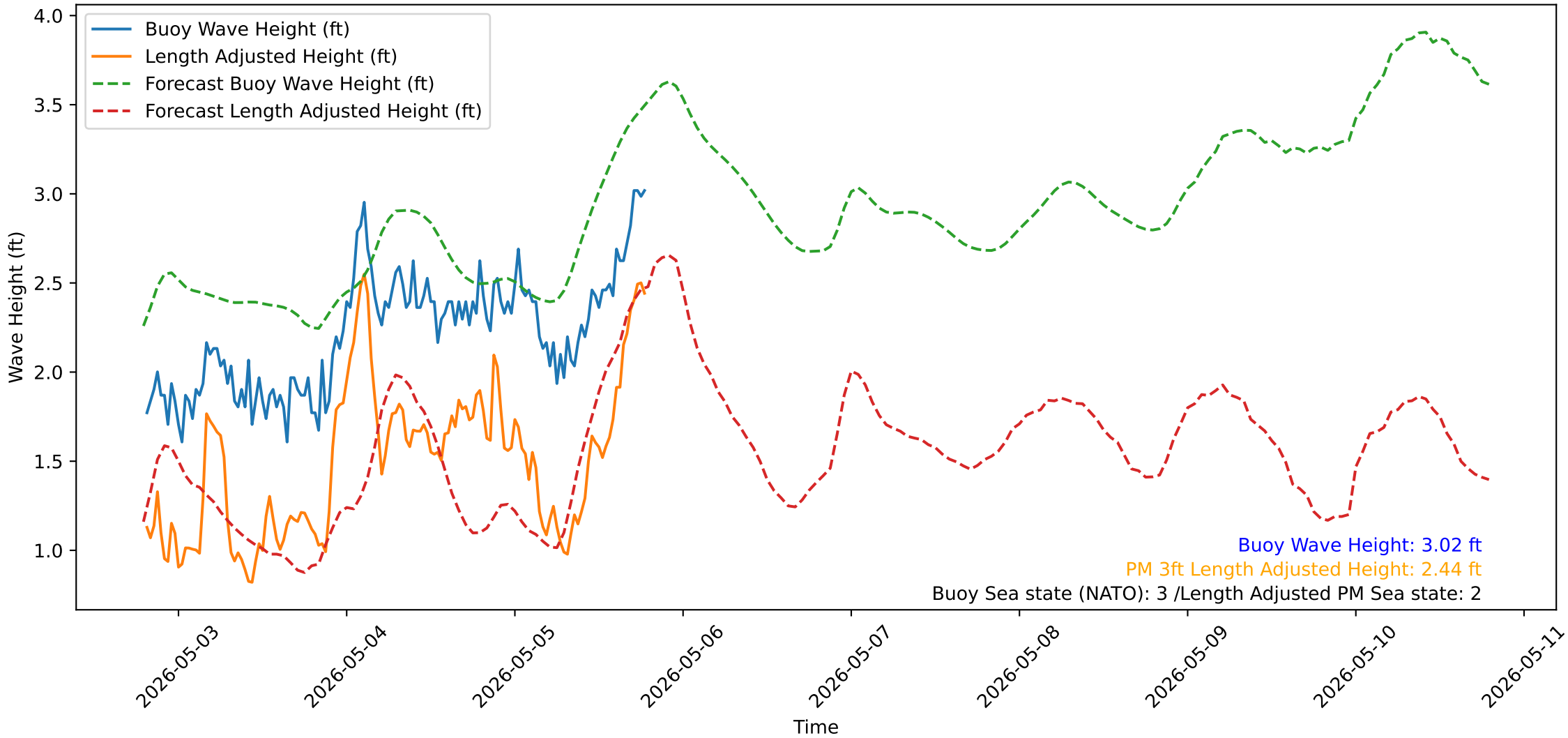
Wave Heights over Time for Red Beach at 2026-05-05 19:20:51
