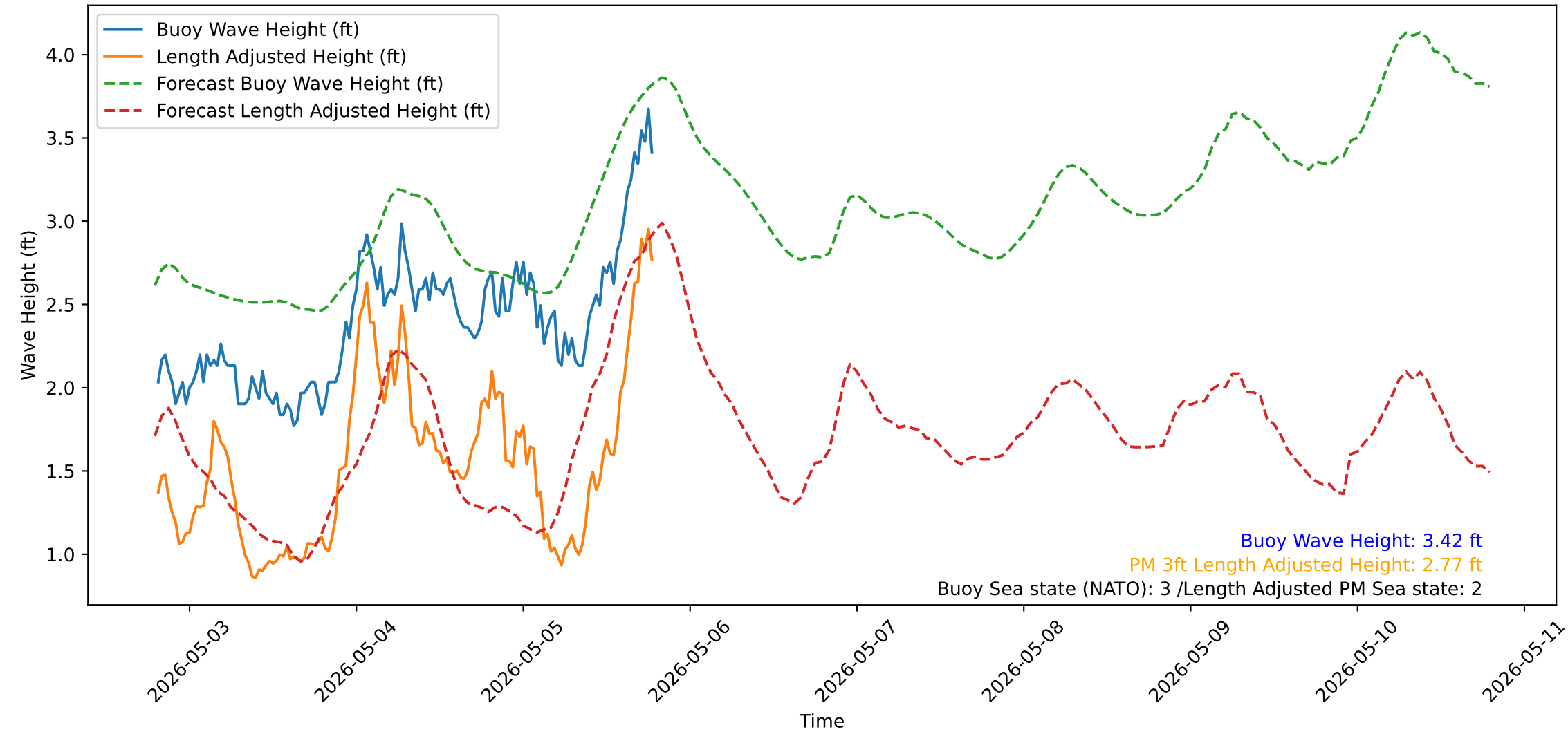
Wave Heights over Time for Green Beach at 2026-05-05 19:21:13
