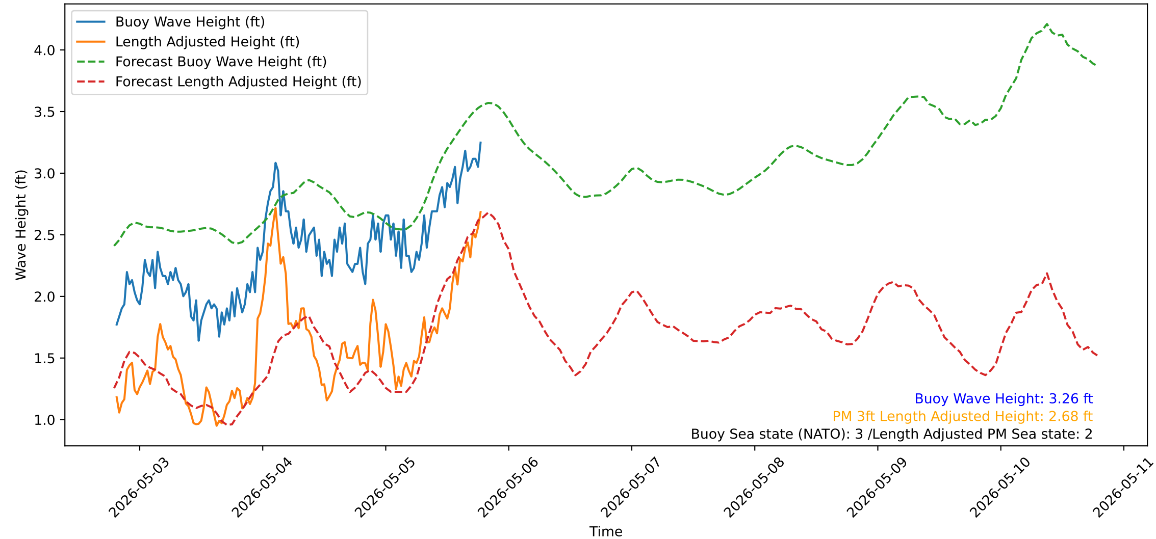
Wave Heights over Time for Oceanside Harbor at 2026-05-05 19:20:31
