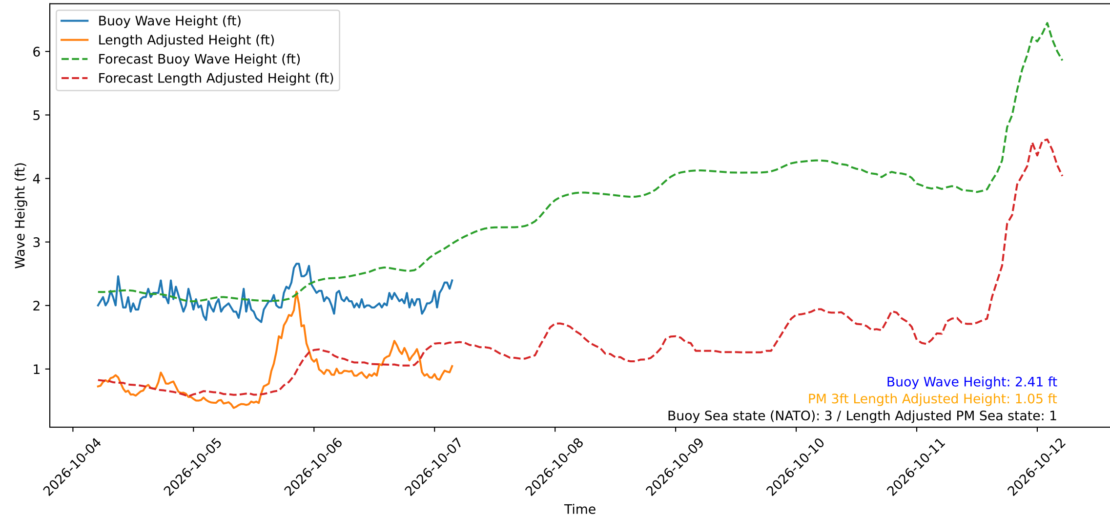
Wave Heights over Time for Red Beach at 2026-10-07 04:30:50
