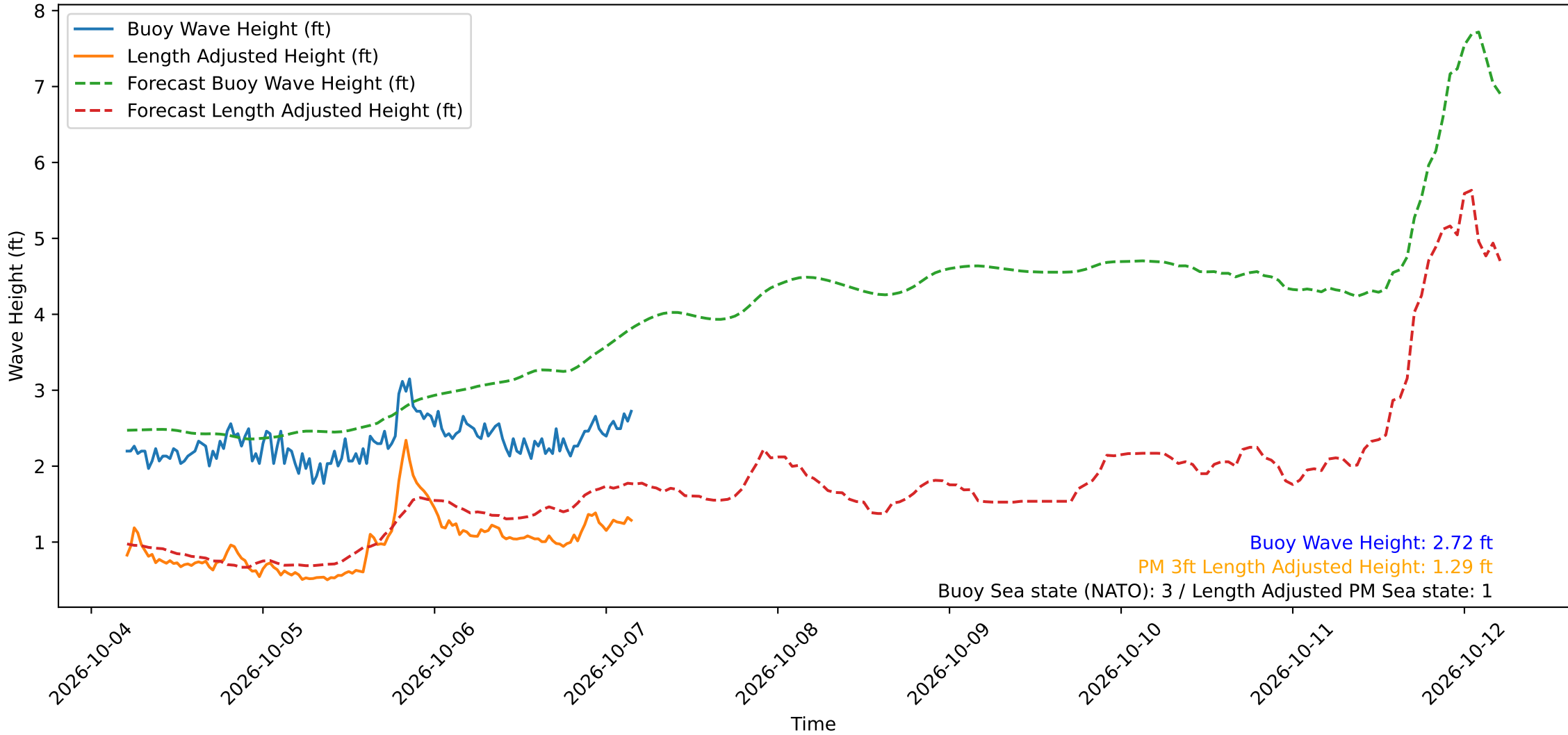
Wave Heights over Time for Green Beach at 2026-10-07 04:31:12
