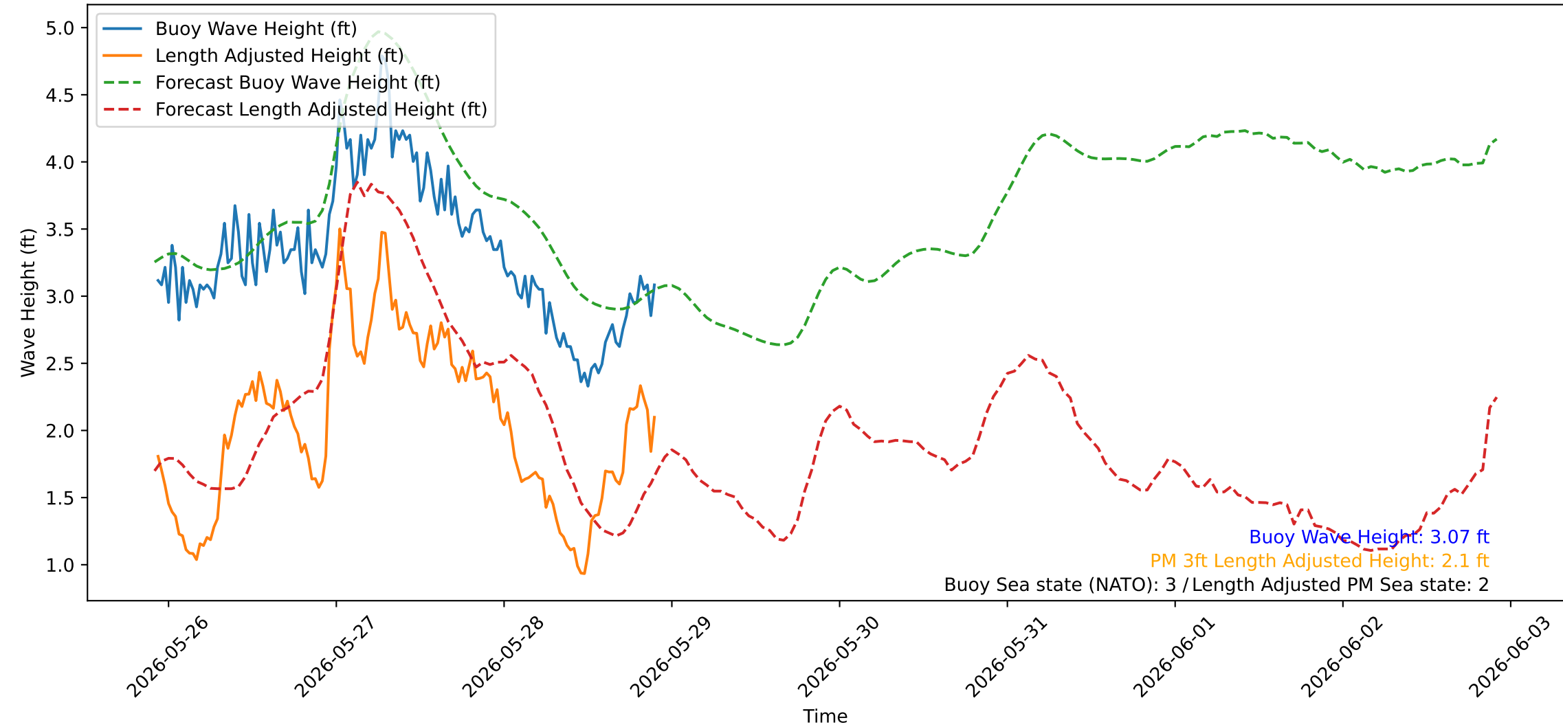
Wave Heights over Time for Red Beach at 2026-05-28 22:10:38
