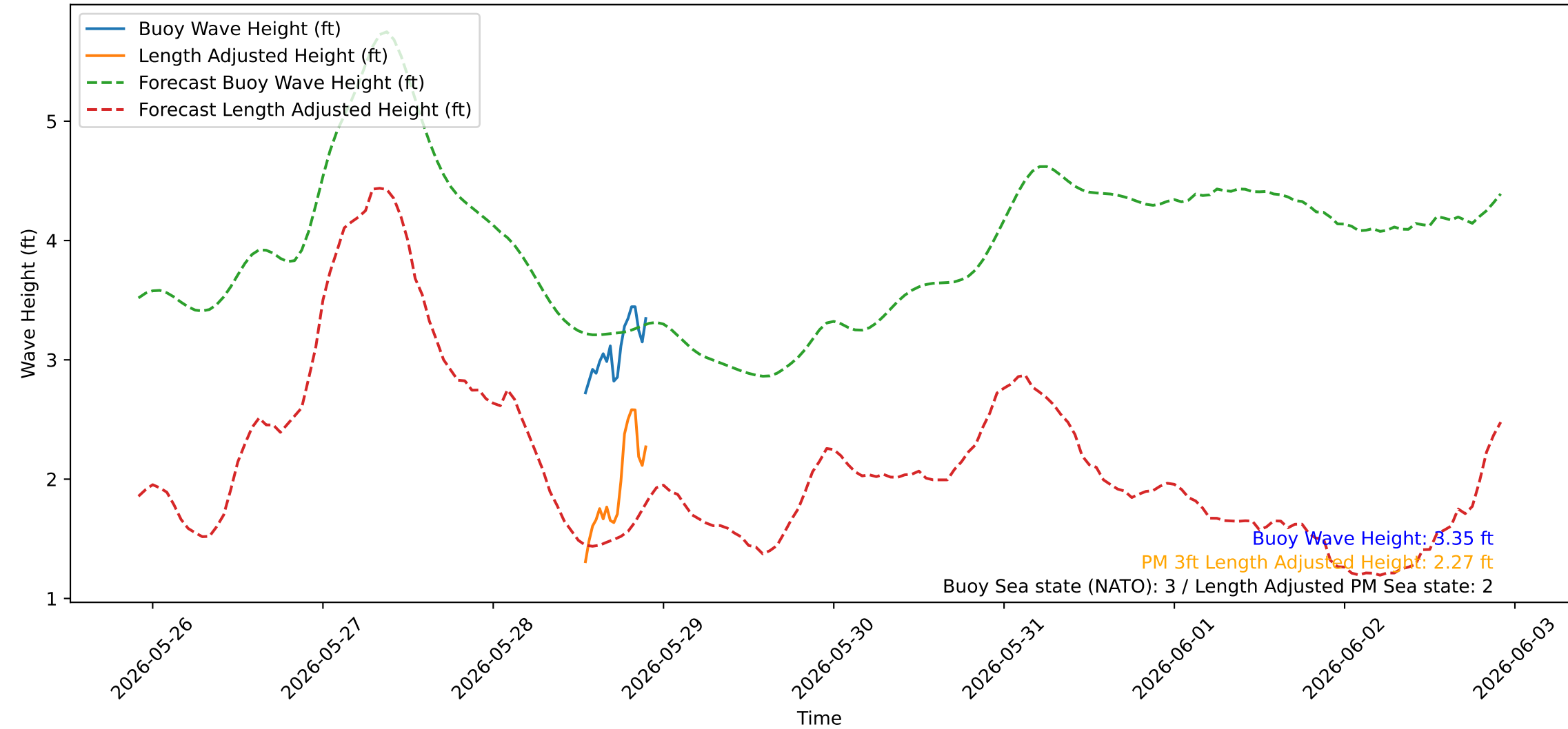
Wave Heights over Time for Oceanside Harbor at 2026-05-28 22:10:19
