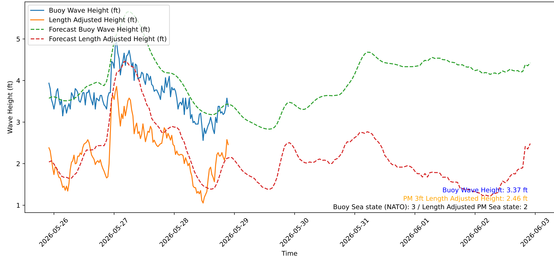
Wave Heights over Time for Green Beach at 2026-05-28 22:11:01
