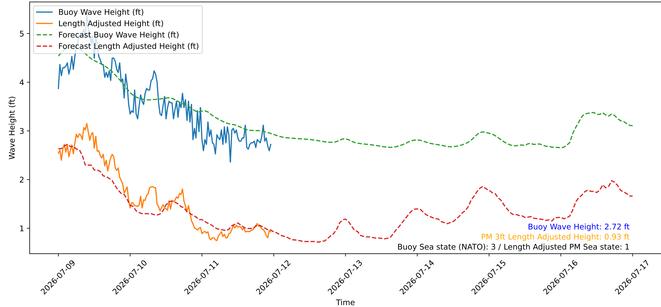
Wave Heights over Time for Oceanside Harbor at 2026-07-11 23:50:26
