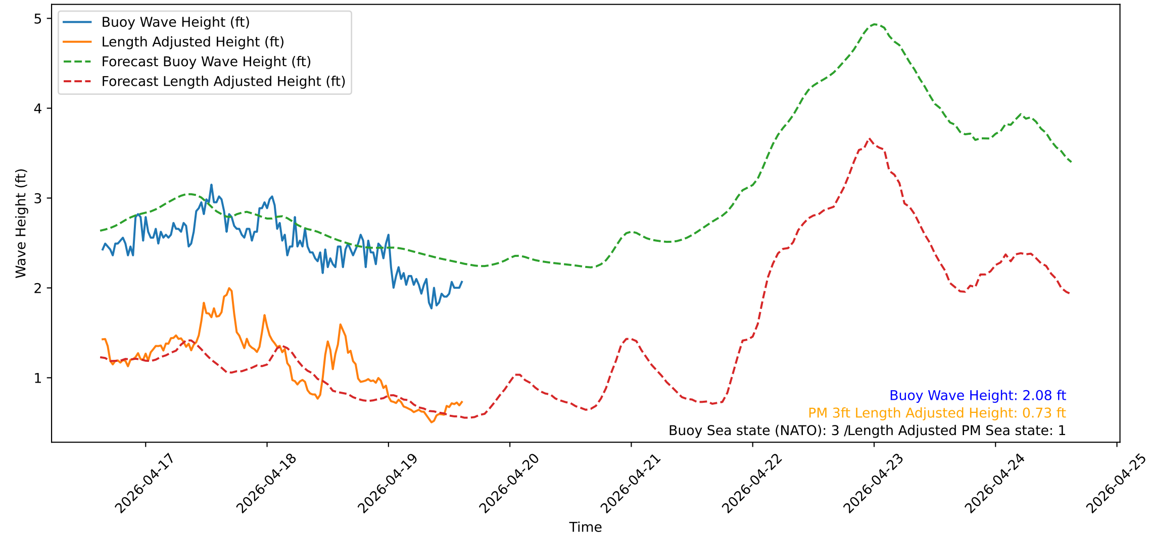
Wave Heights over Time for Red Beach at 2026-04-19 15:20:51
