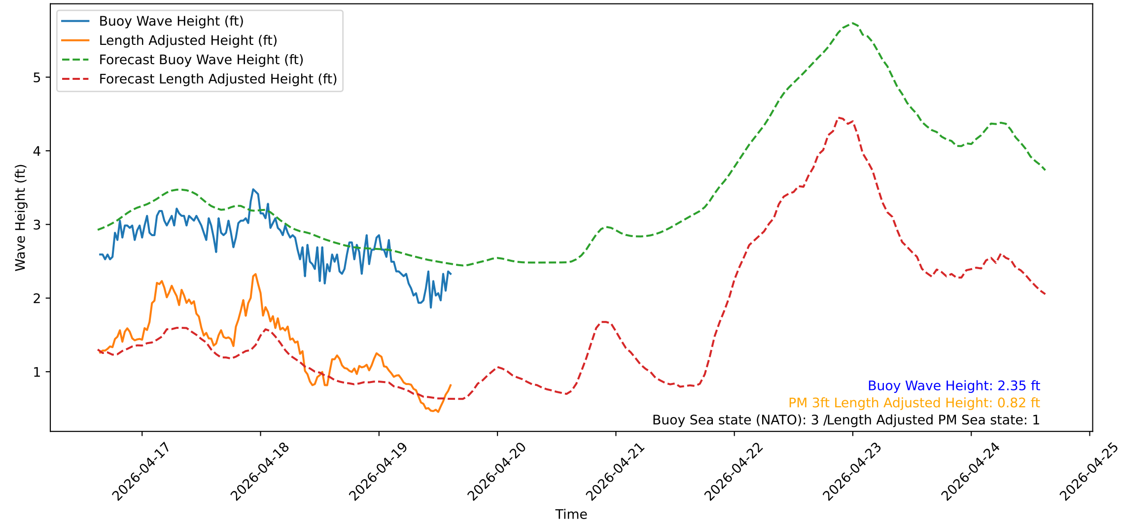
Wave Heights over Time for Green Beach at 2026-04-19 15:21:13
