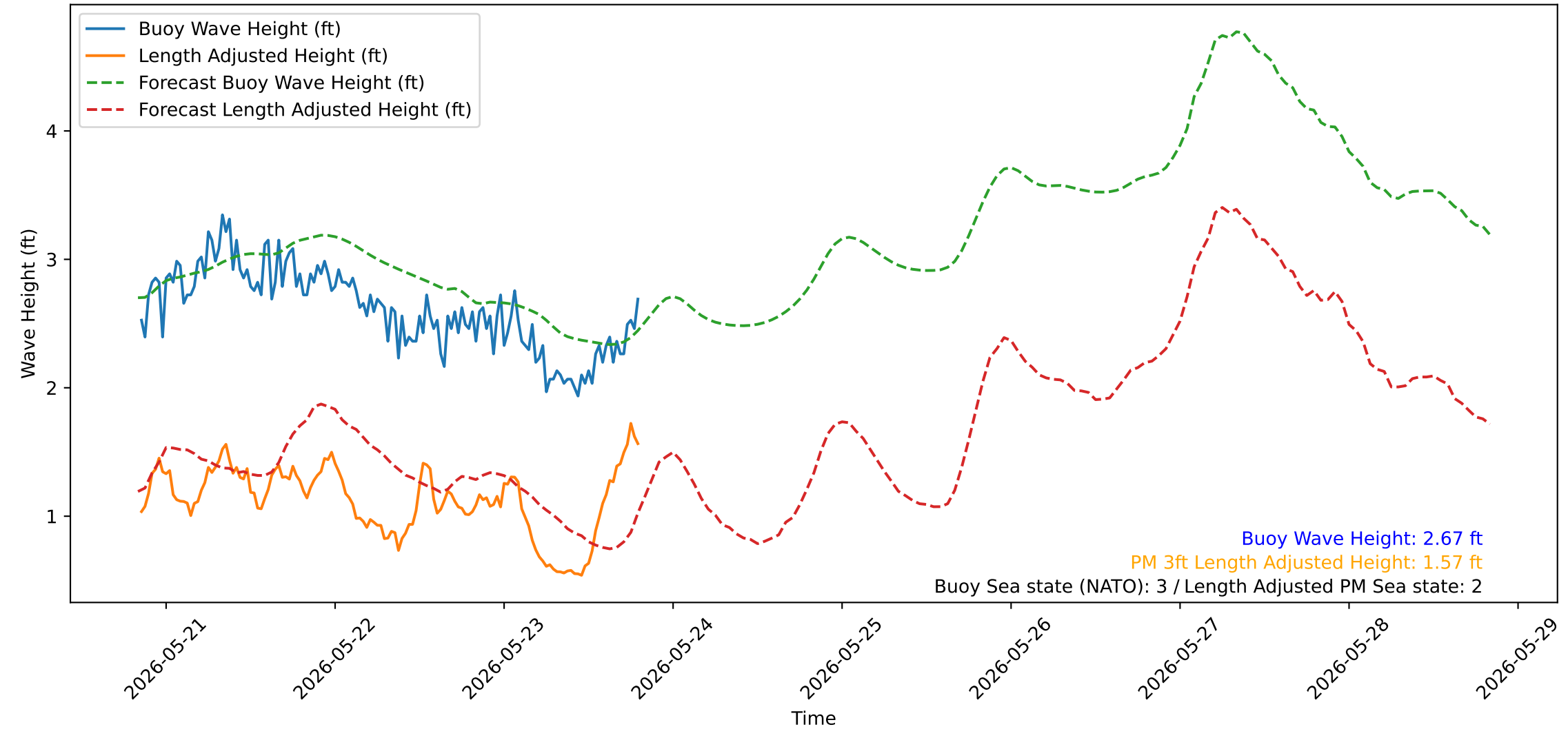
Wave Heights over Time for Red Beach at 2026-05-23 20:00:51
