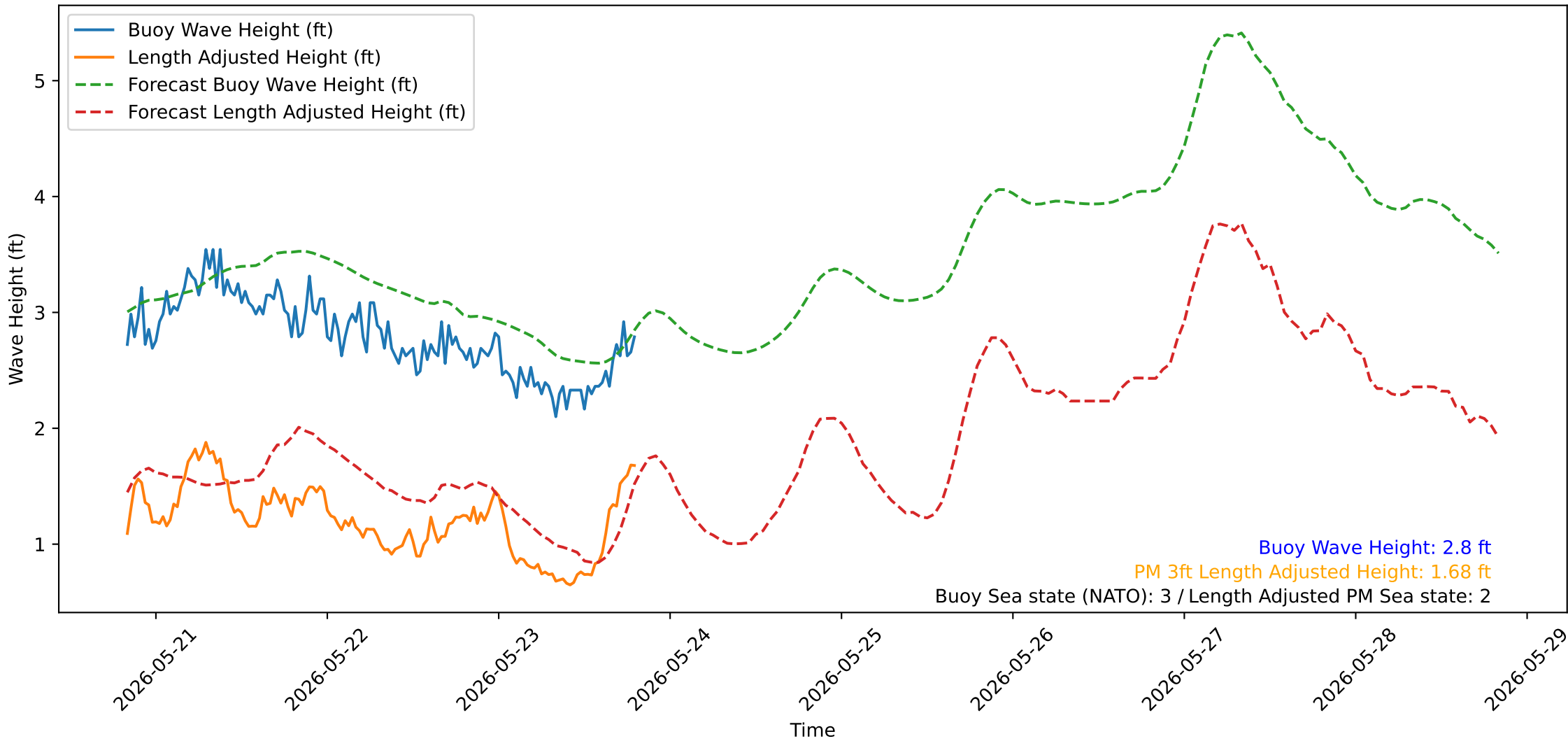
Wave Heights over Time for Green Beach at 2026-05-23 20:01:14
