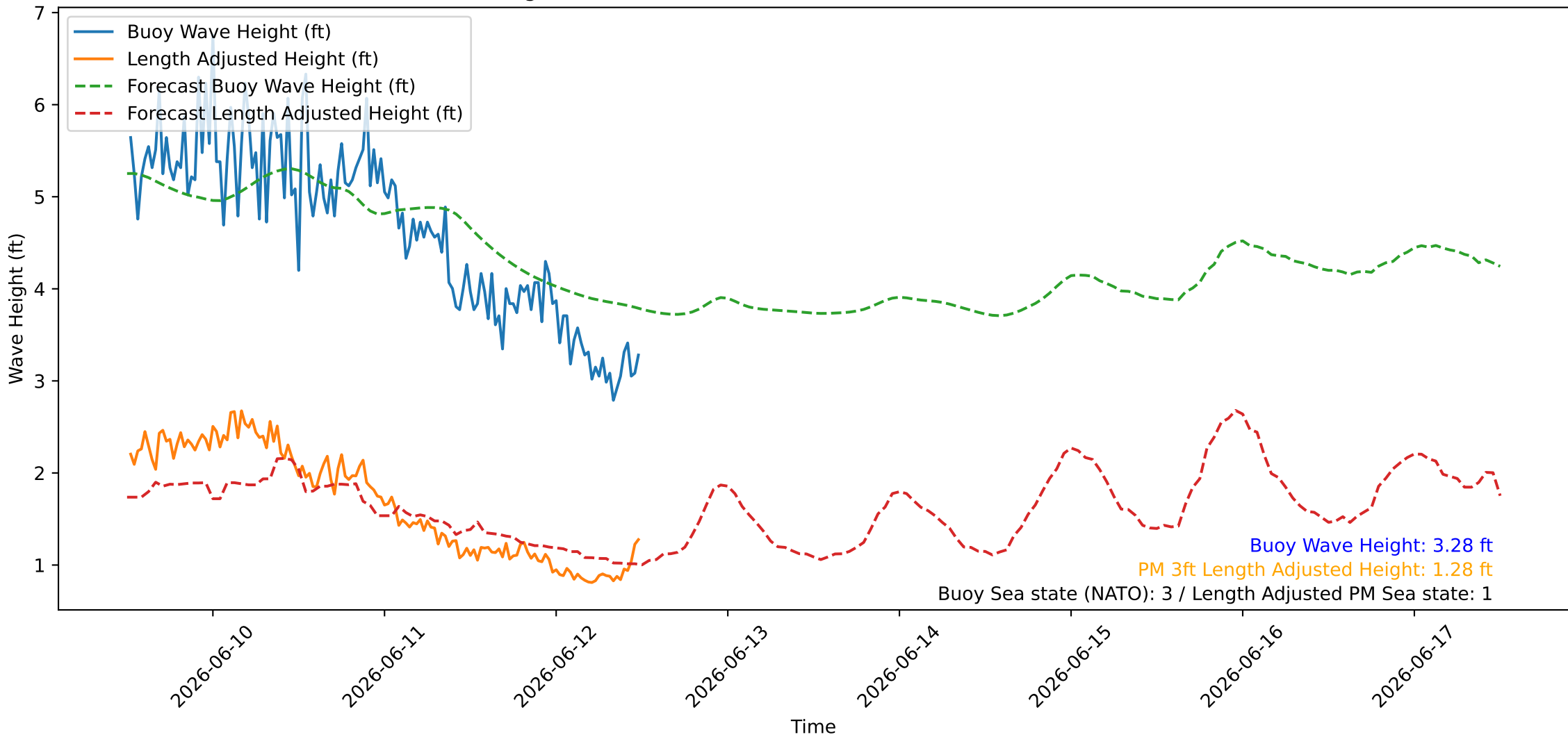
Wave Heights over Time for Oceanside Harbor at 2026-06-12 12:20:26
