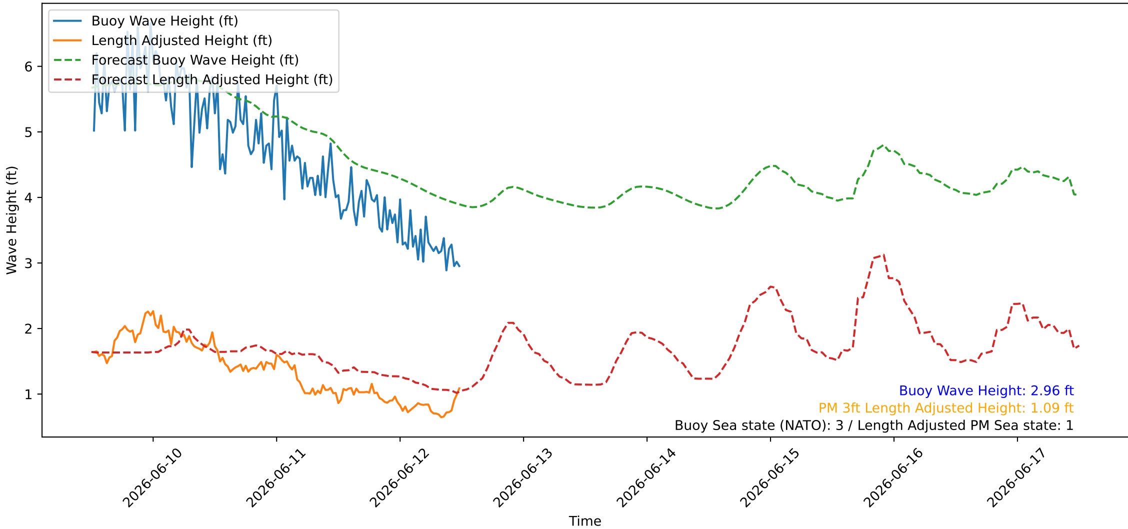
Wave Heights over Time for Green Beach at 2026-06-12 12:21:10
