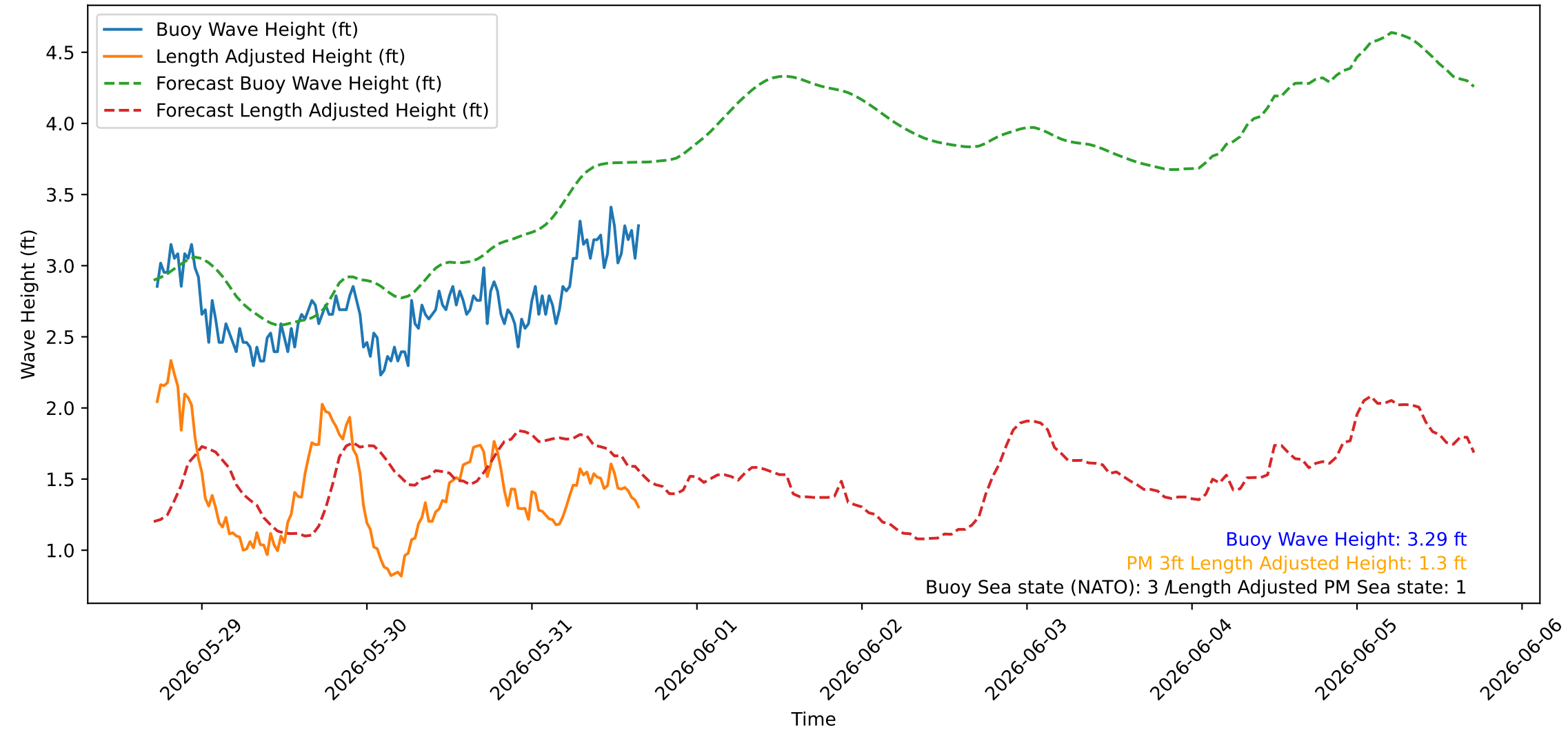
Wave Heights over Time for Red Beach at 2026-05-31 17:00:45
