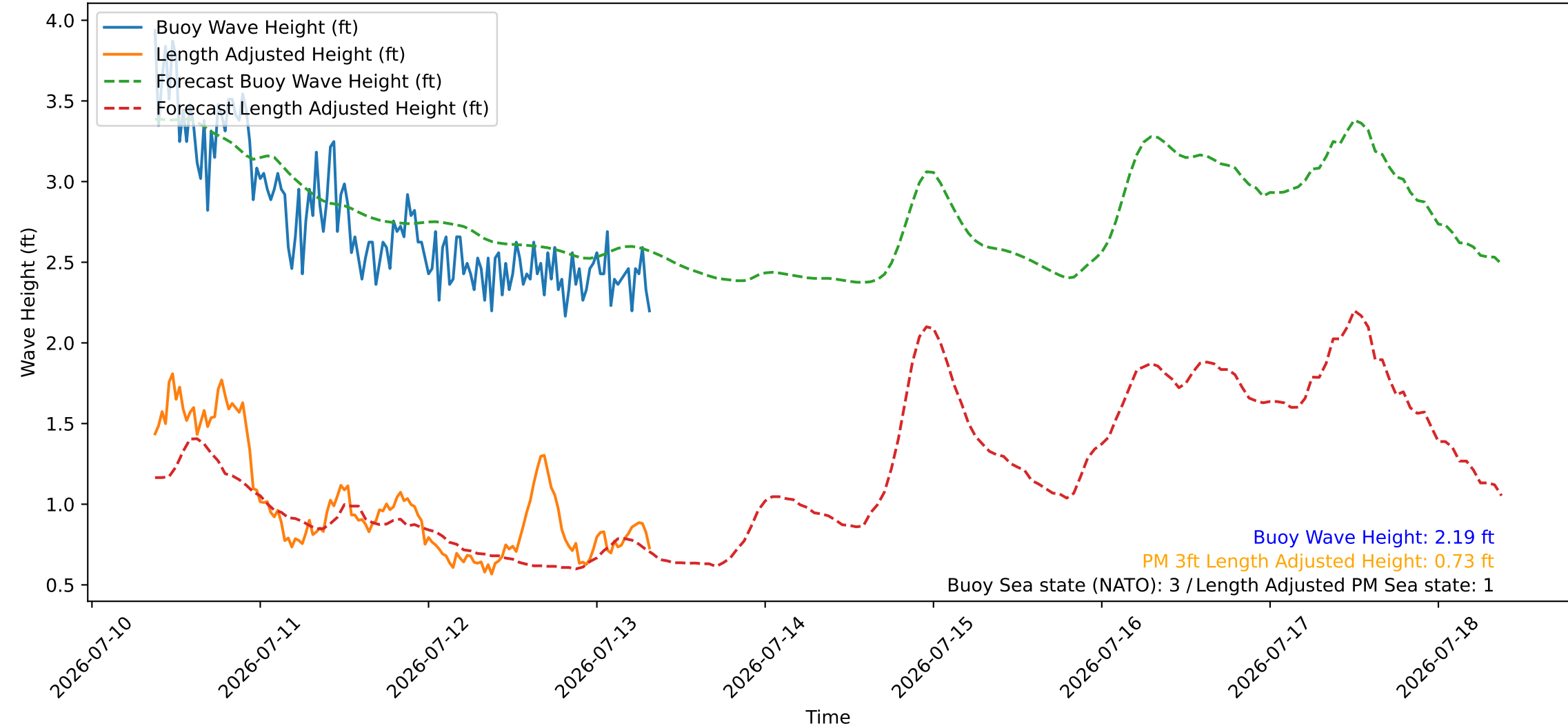
Wave Heights over Time for Red Beach at 2026-07-13 08:40:46
