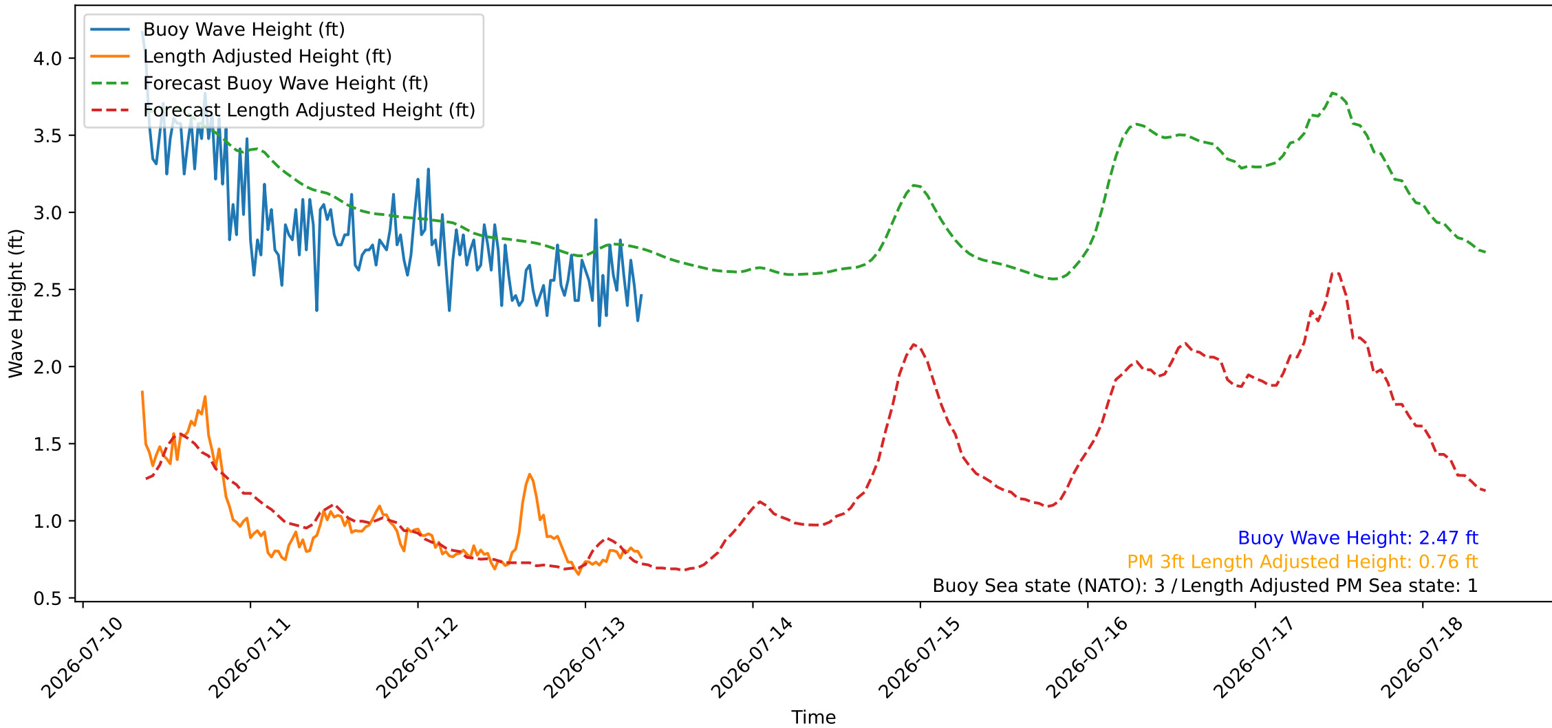
Wave Heights over Time for Oceanside Harbor at 2026-07-13 08:40:26
