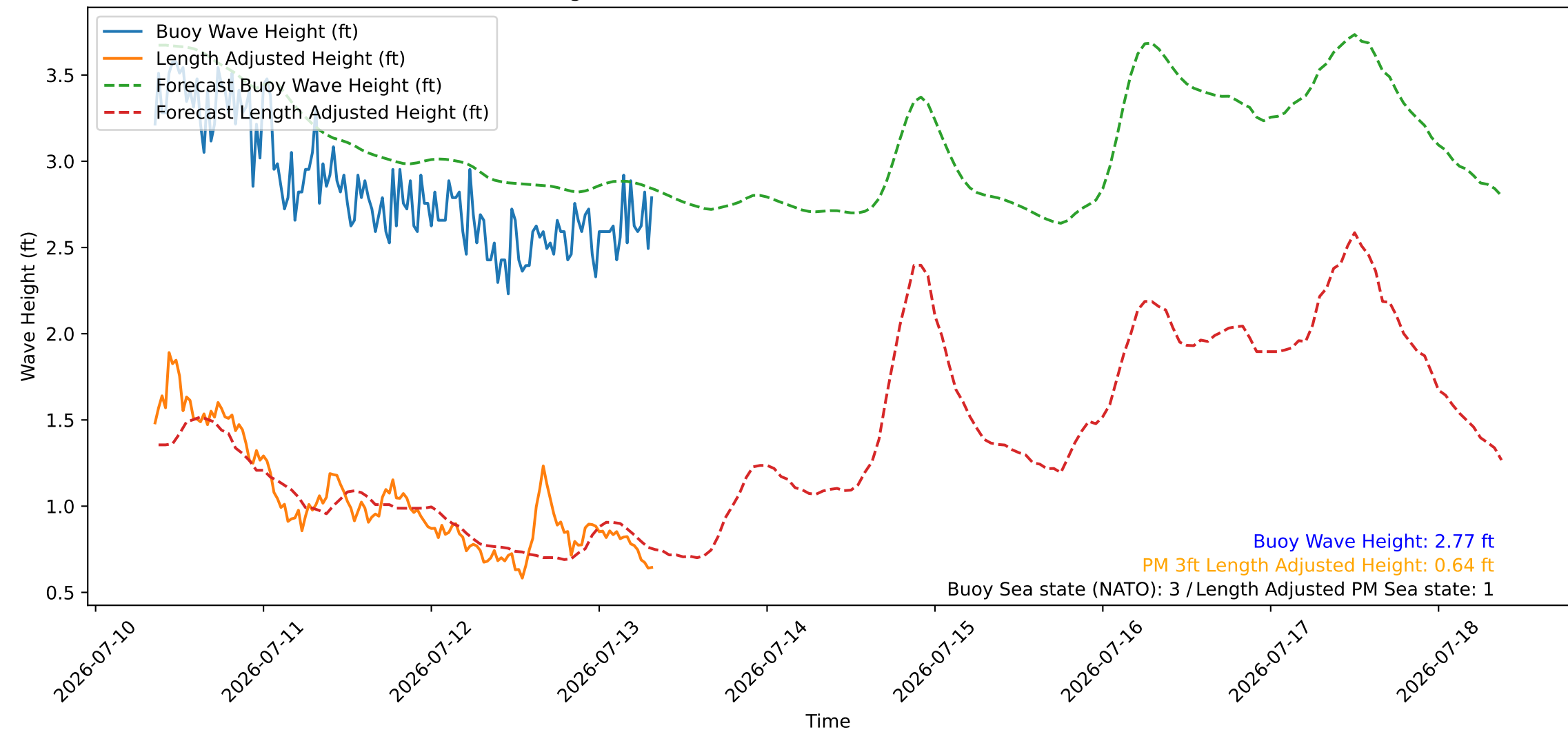
Wave Heights over Time for Green Beach at 2026-07-13 08:41:08
