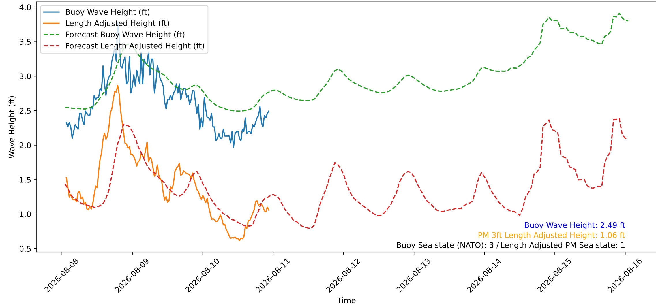
Wave Heights over Time for Green Beach at 2026-08-11 01:21:09
