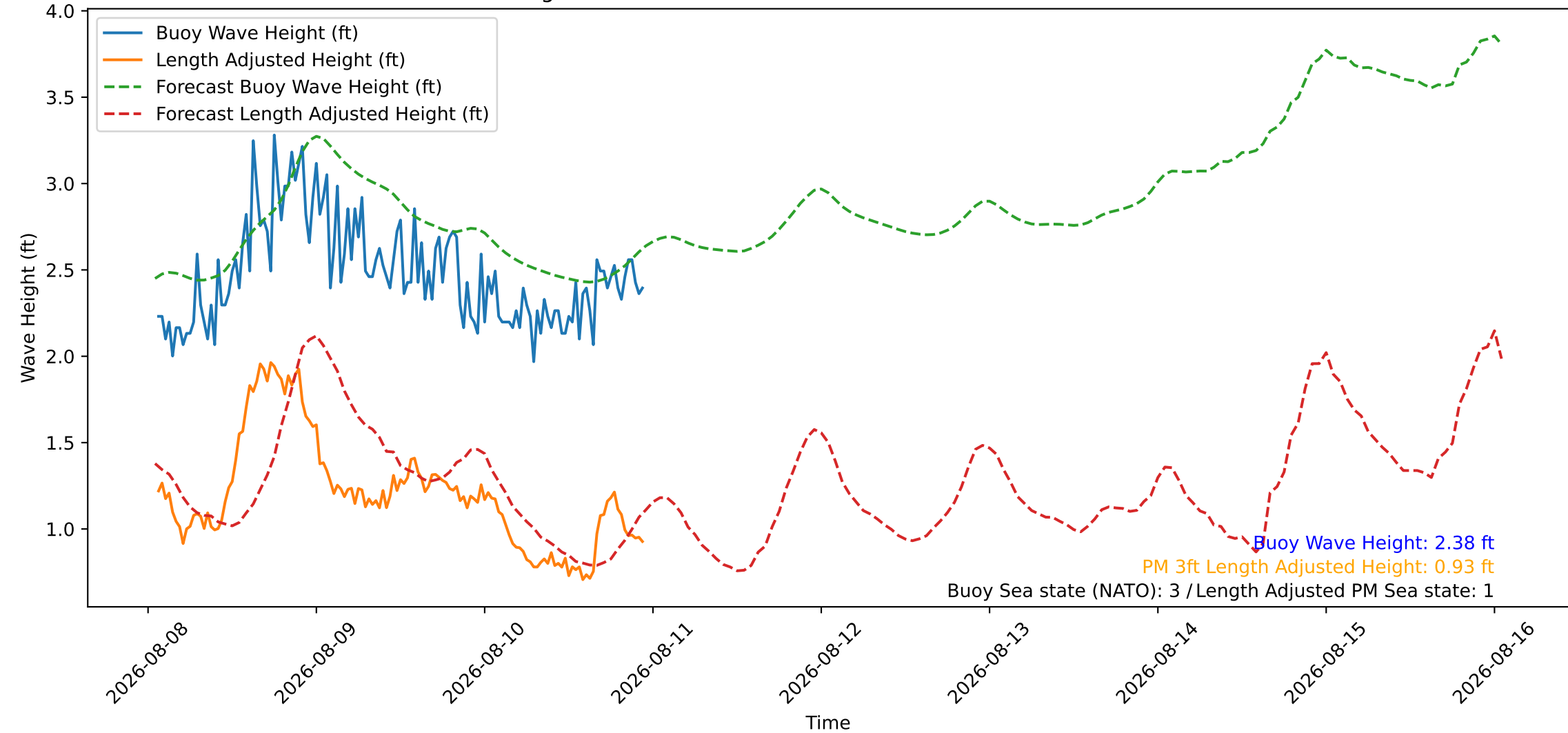
Wave Heights over Time for Oceanside Harbor at 2026-08-11 01:20:26
