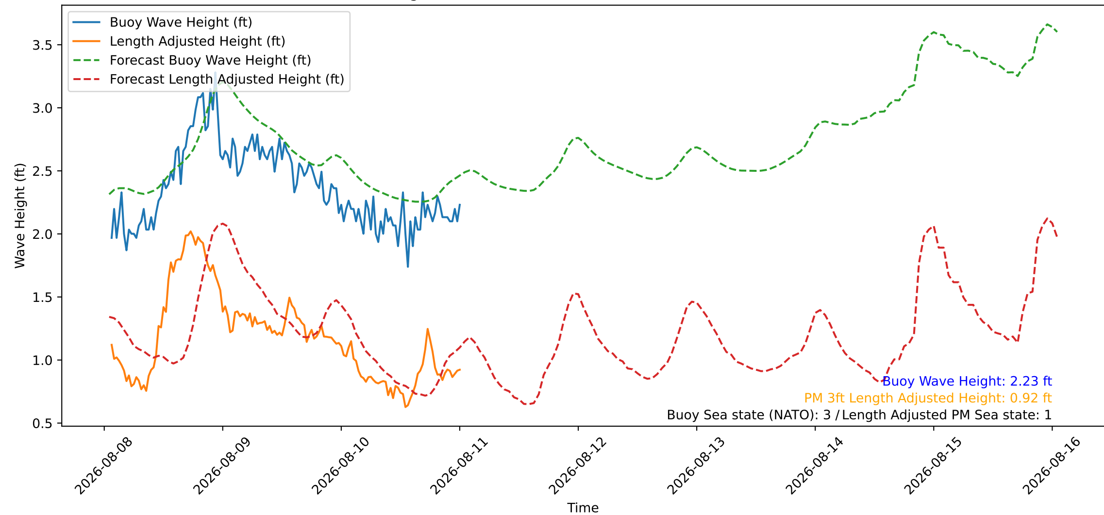
Wave Heights over Time for Red Beach at 2026-08-11 01:20:46
