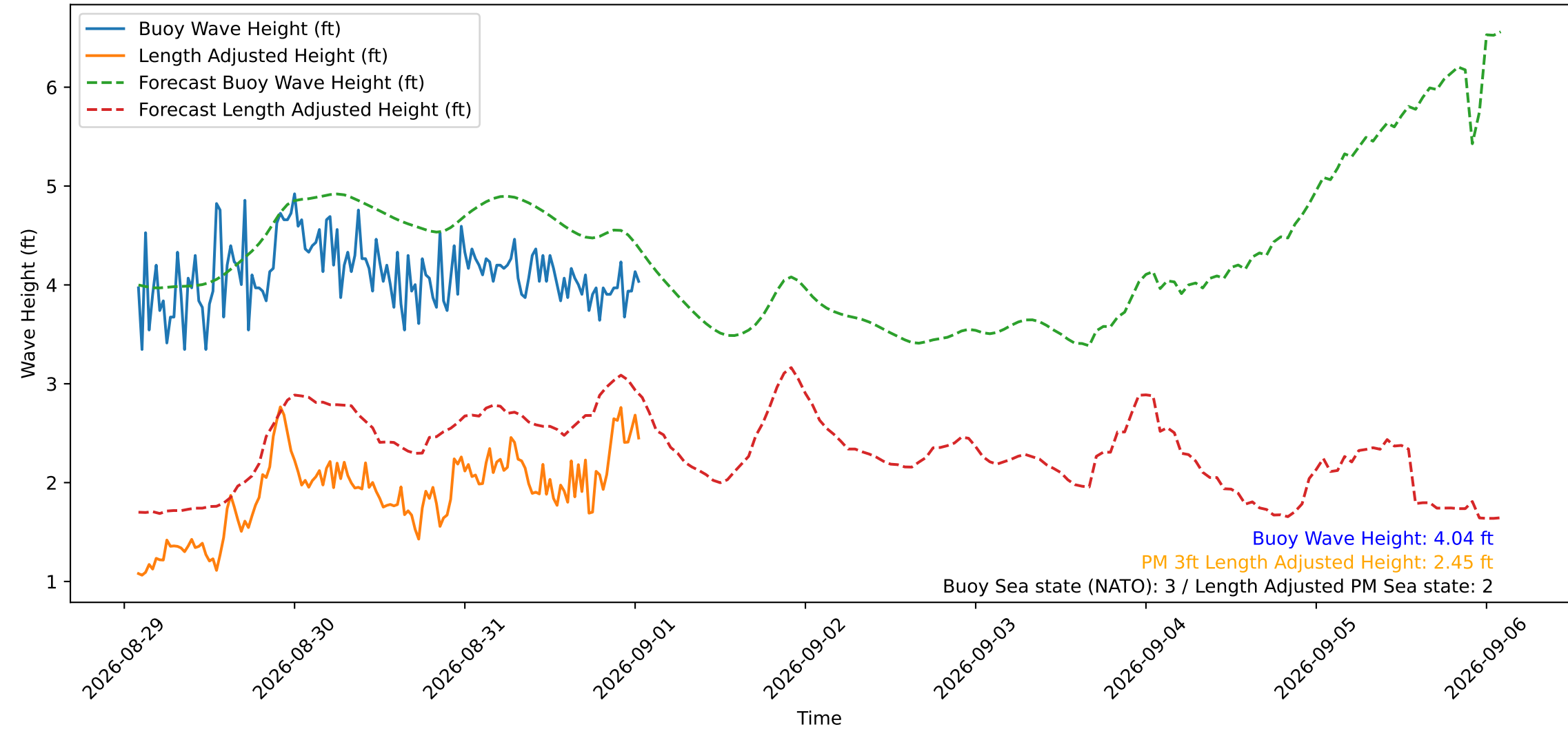
Wave Heights over Time for Green Beach at 2026-09-01 01:51:14
