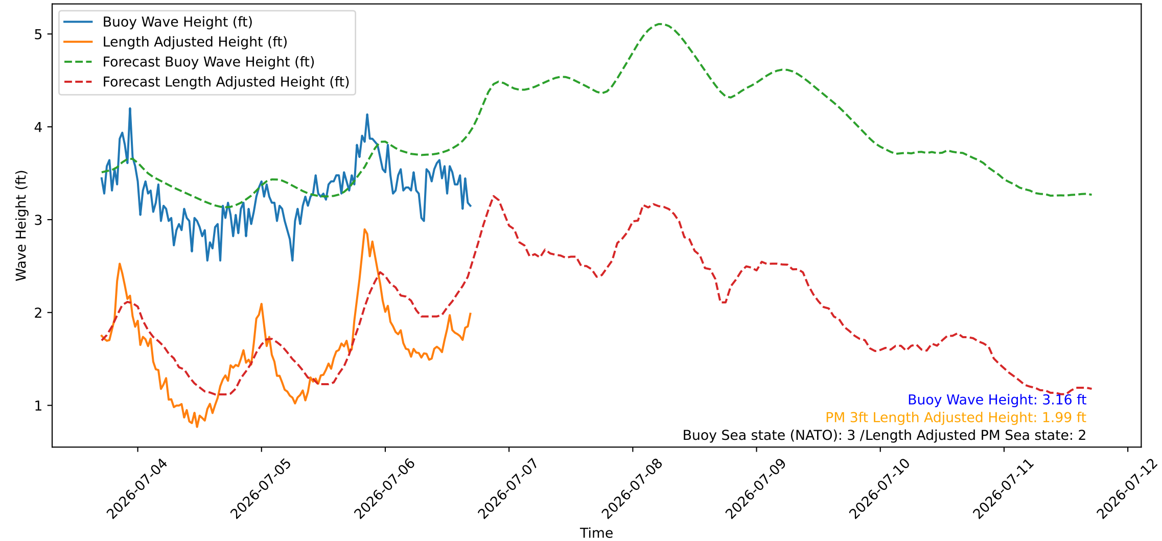
Wave Heights over Time for Green Beach at 2026-07-06 17:11:08
