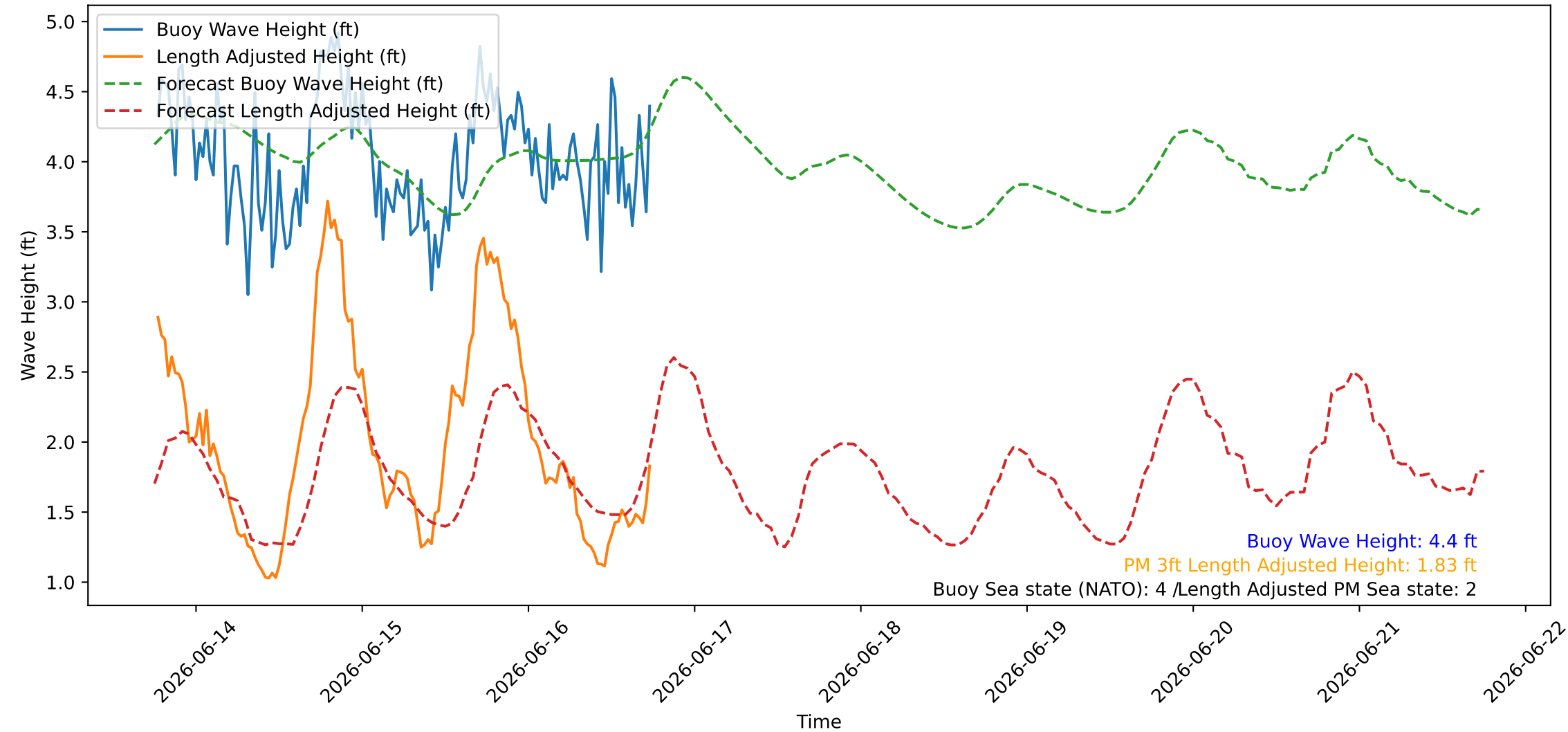
Wave Heights over Time for Green Beach at 2026-06-16 18:21:11
