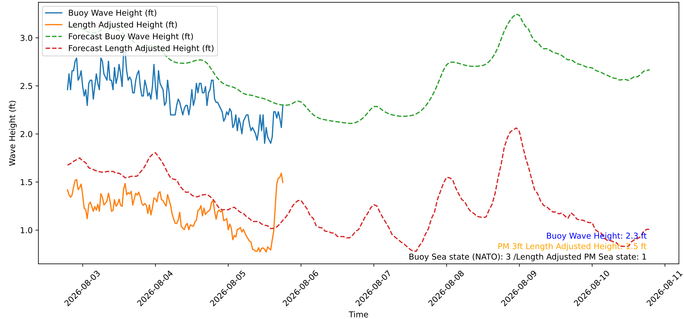
Wave Heights over Time for Oceanside Harbor at 2026-08-05 18:50:25
