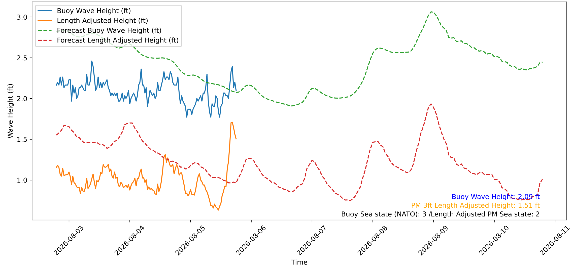
Wave Heights over Time for Red Beach at 2026-08-05 18:50:46
