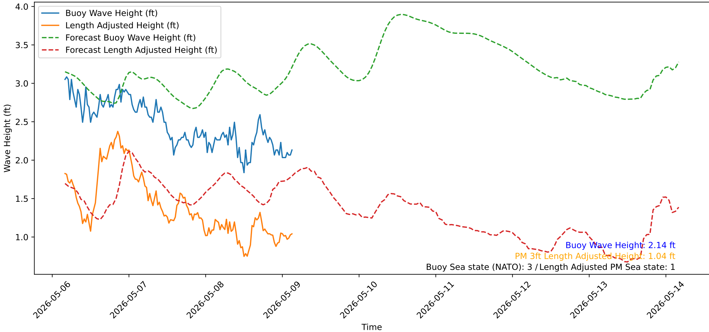
Wave Heights over Time for Green Beach at 2026-05-09 04:01:13
