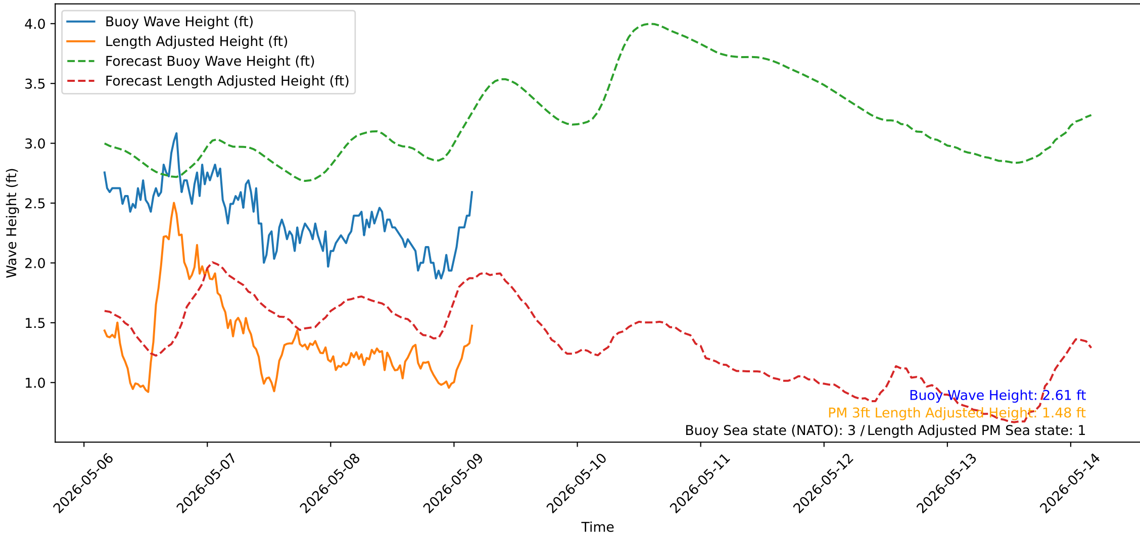
Wave Heights over Time for Oceanside Harbor at 2026-05-09 04:00:31
