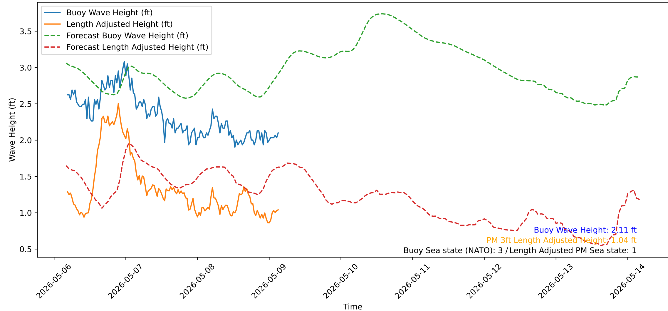
Wave Heights over Time for Red Beach at 2026-05-09 04:00:50
