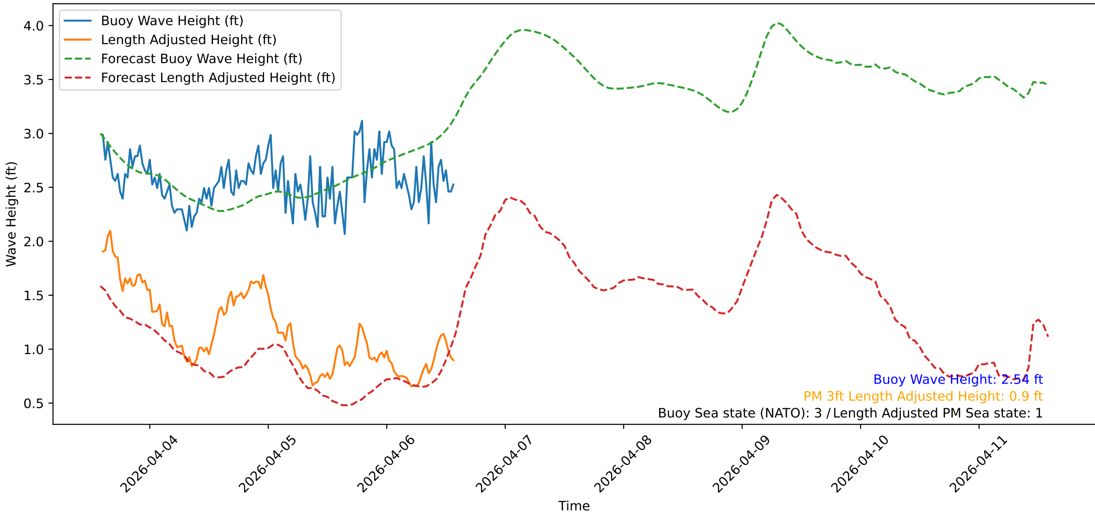
Wave Heights over Time for Oceanside Harbor at 2026-04-06 14:20:32
