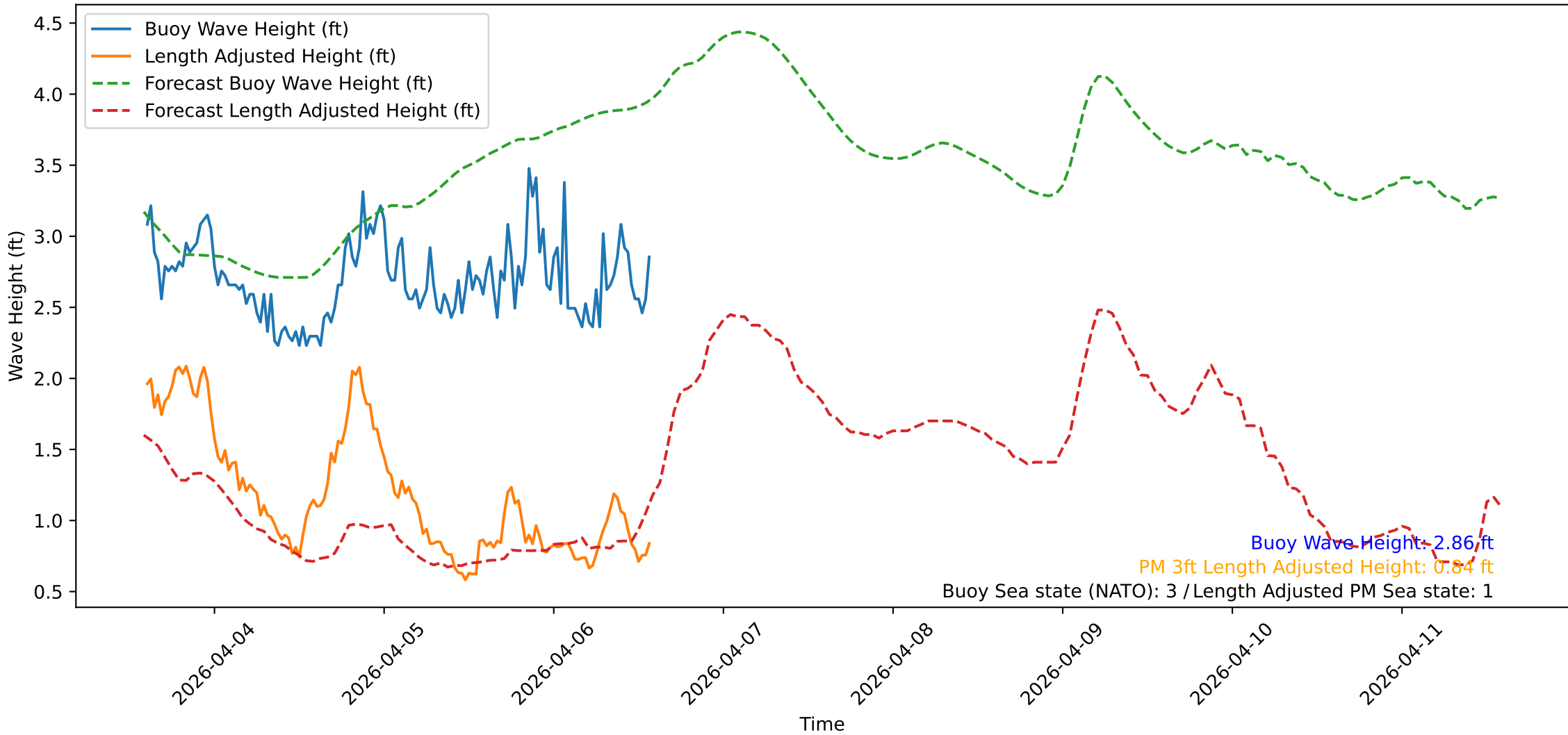
Wave Heights over Time for Green Beach at 2026-04-06 14:21:11
