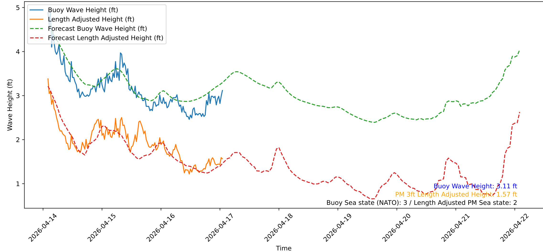
Wave Heights over Time for Green Beach at 2026-04-17 01:51:22
