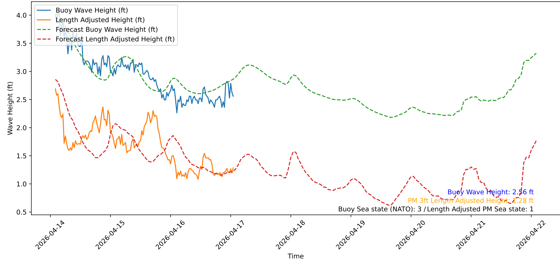
Wave Heights over Time for Red Beach at 2026-04-17 01:50:59
