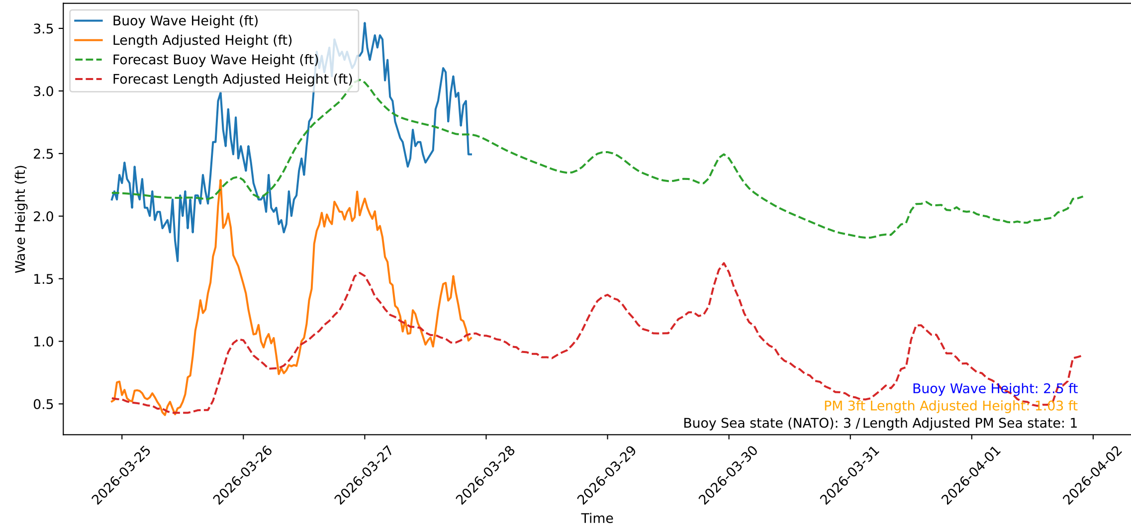
Wave Heights over Time for Green Beach at 2026-03-27 21:51:08
