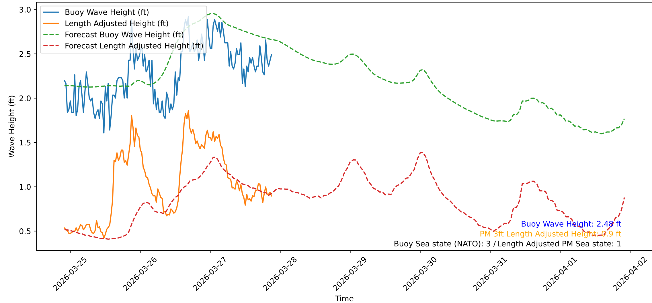
Wave Heights over Time for Oceanside Harbor at 2026-03-27 21:50:30
