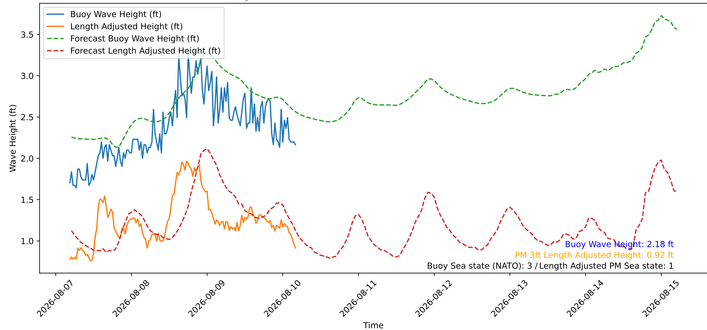
Wave Heights over Time for Oceanside Harbor at 2026-08-10 04:40:26
