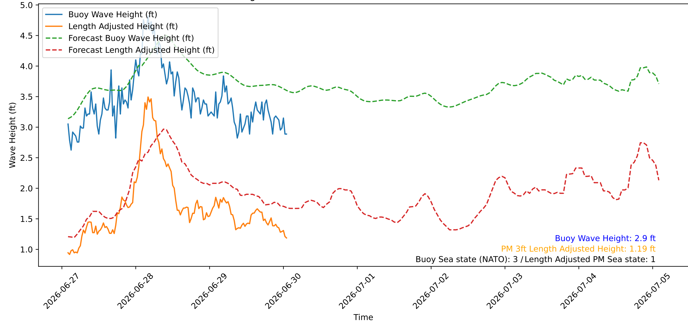
Wave Heights over Time for Green Beach at 2026-06-30 01:51:08
