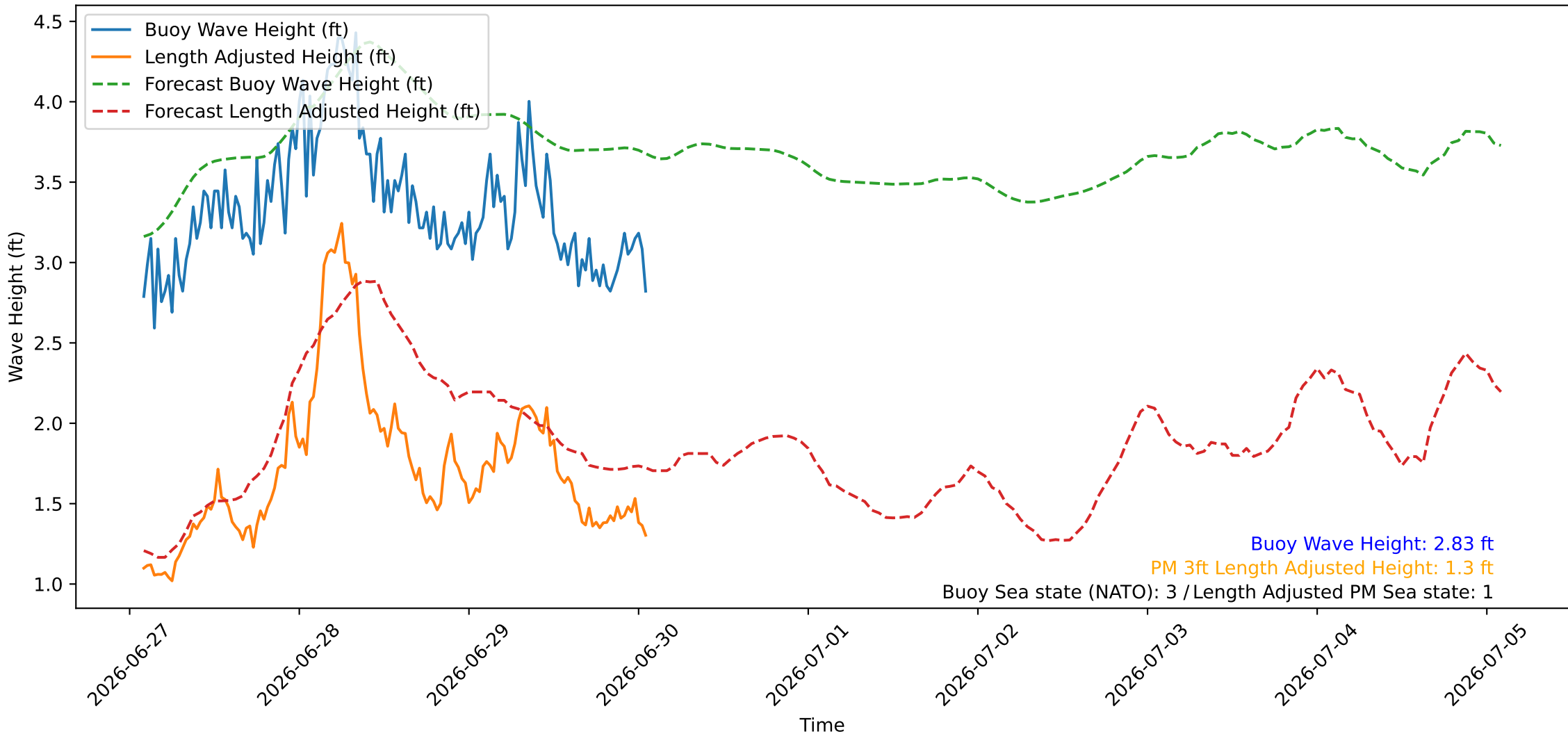
Wave Heights over Time for Oceanside Harbor at 2026-06-30 01:50:26
