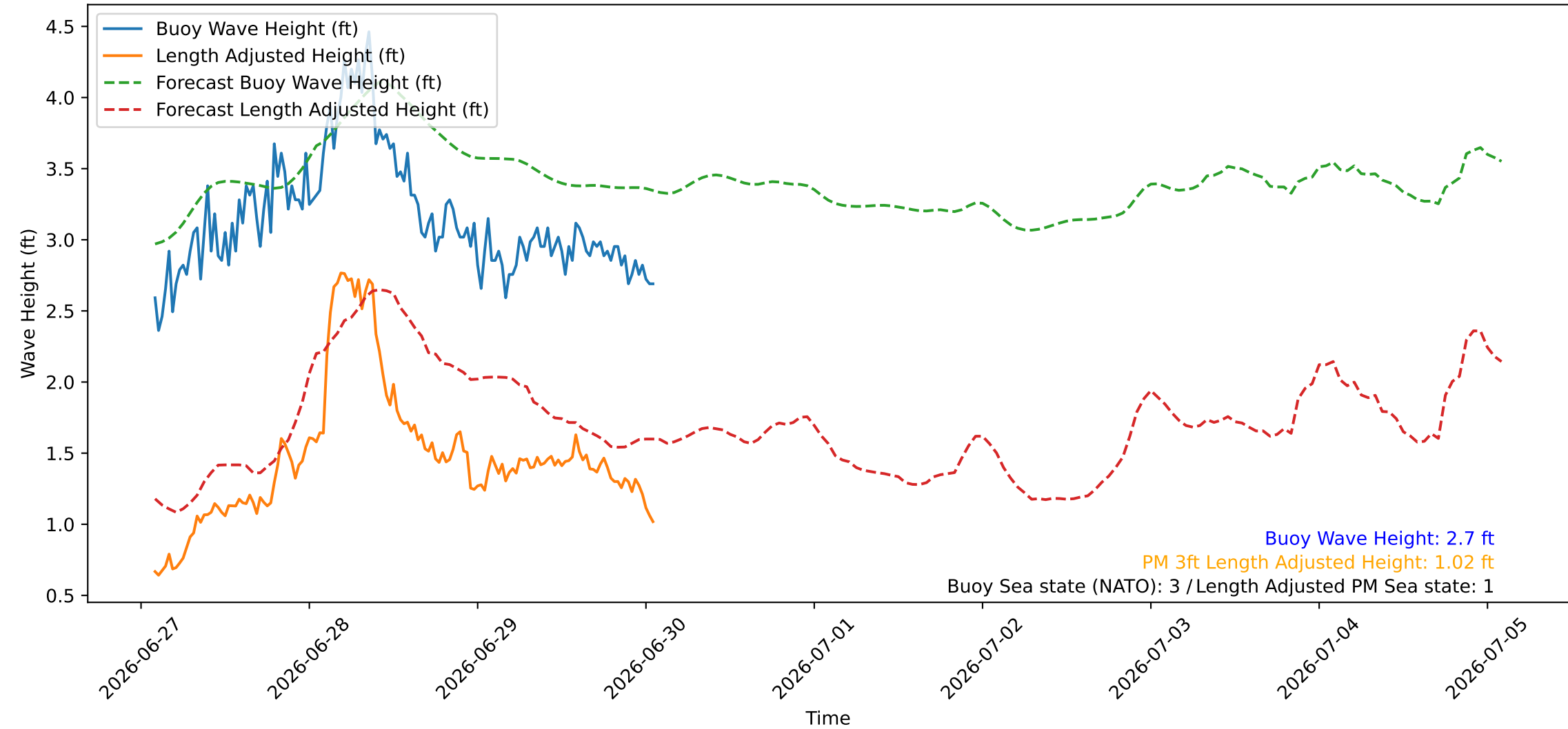
Wave Heights over Time for Red Beach at 2026-06-30 01:50:45
