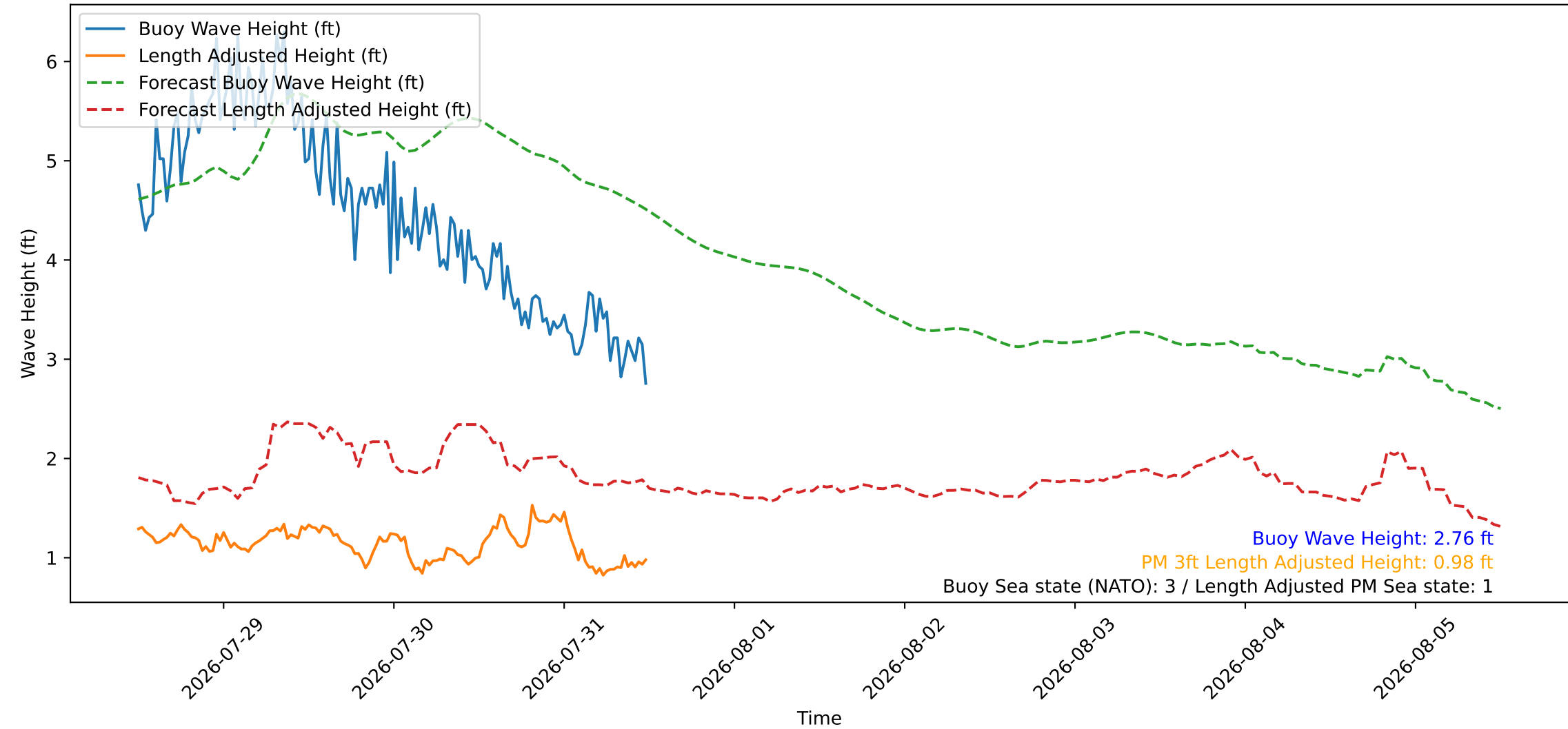
Wave Heights over Time for Green Beach at 2026-07-31 12:11:08
