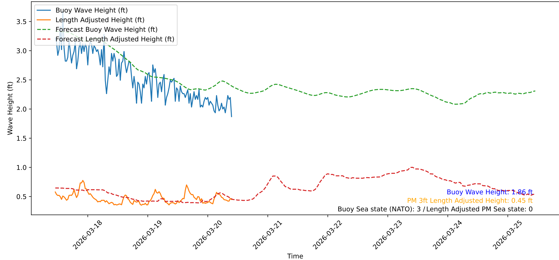
Wave Heights over Time for Red Beach at 2026-03-20 10:50:47
