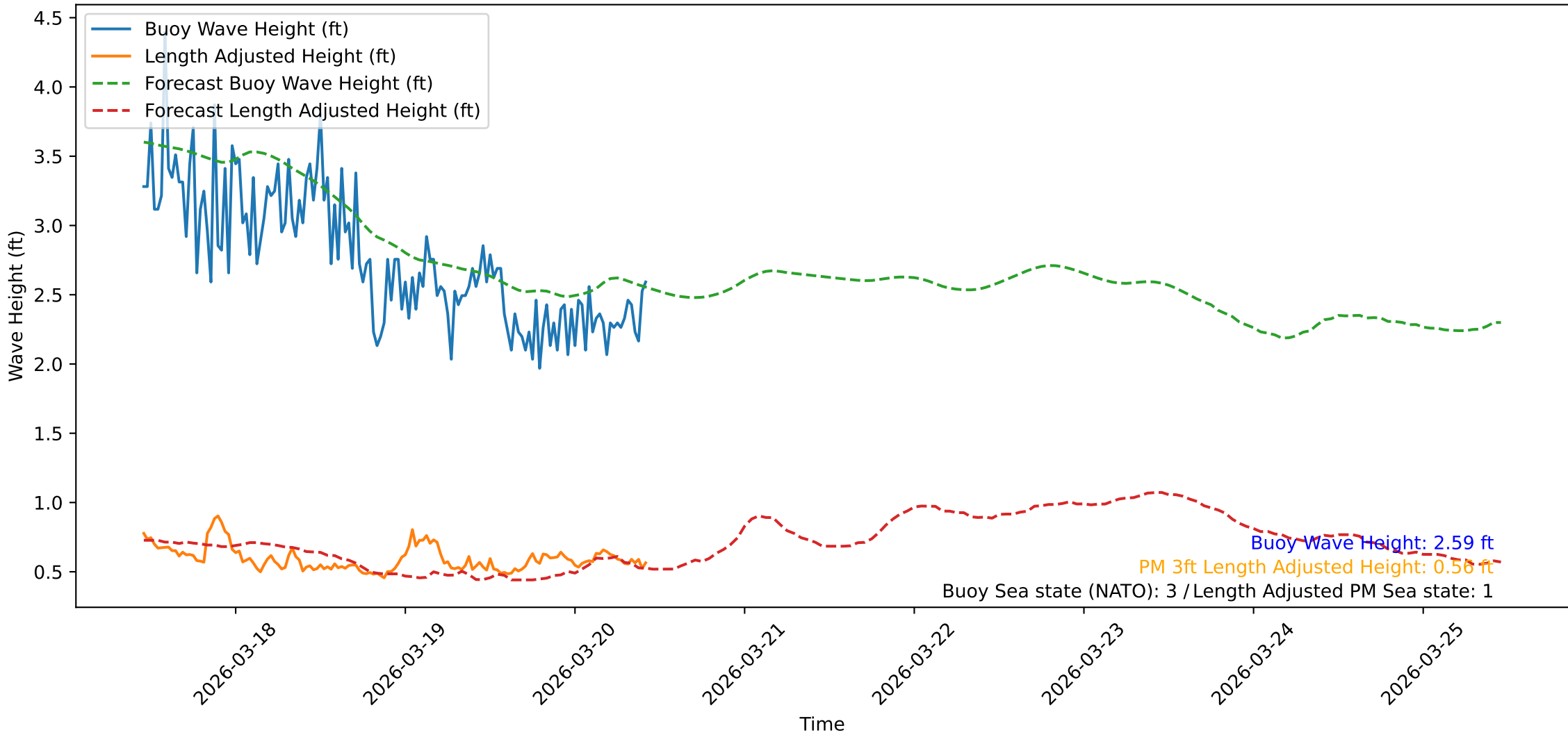
Wave Heights over Time for Oceanside Harbor at 2026-03-20 10:50:31
