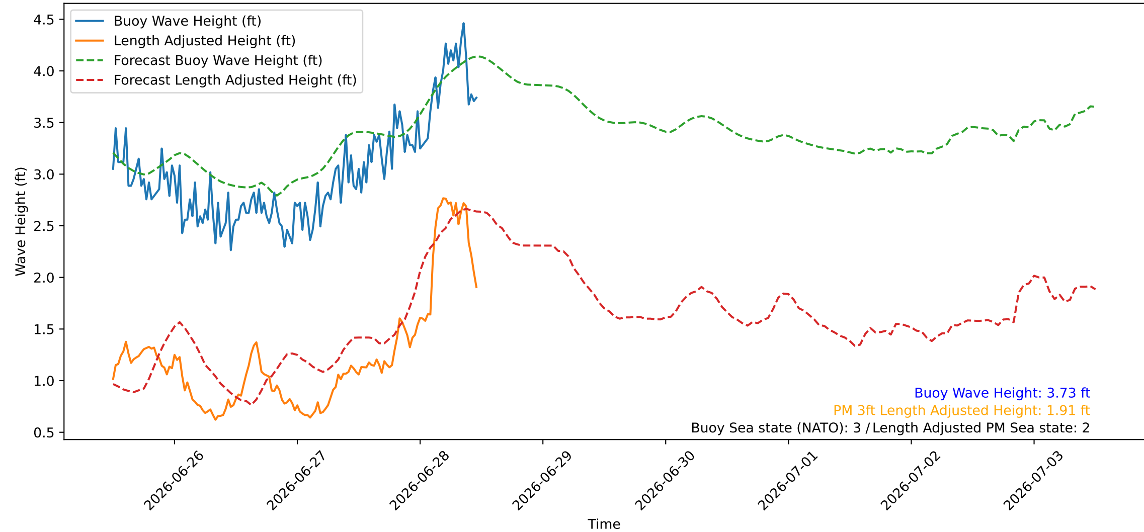
Wave Heights over Time for Red Beach at 2026-06-28 11:40:44
