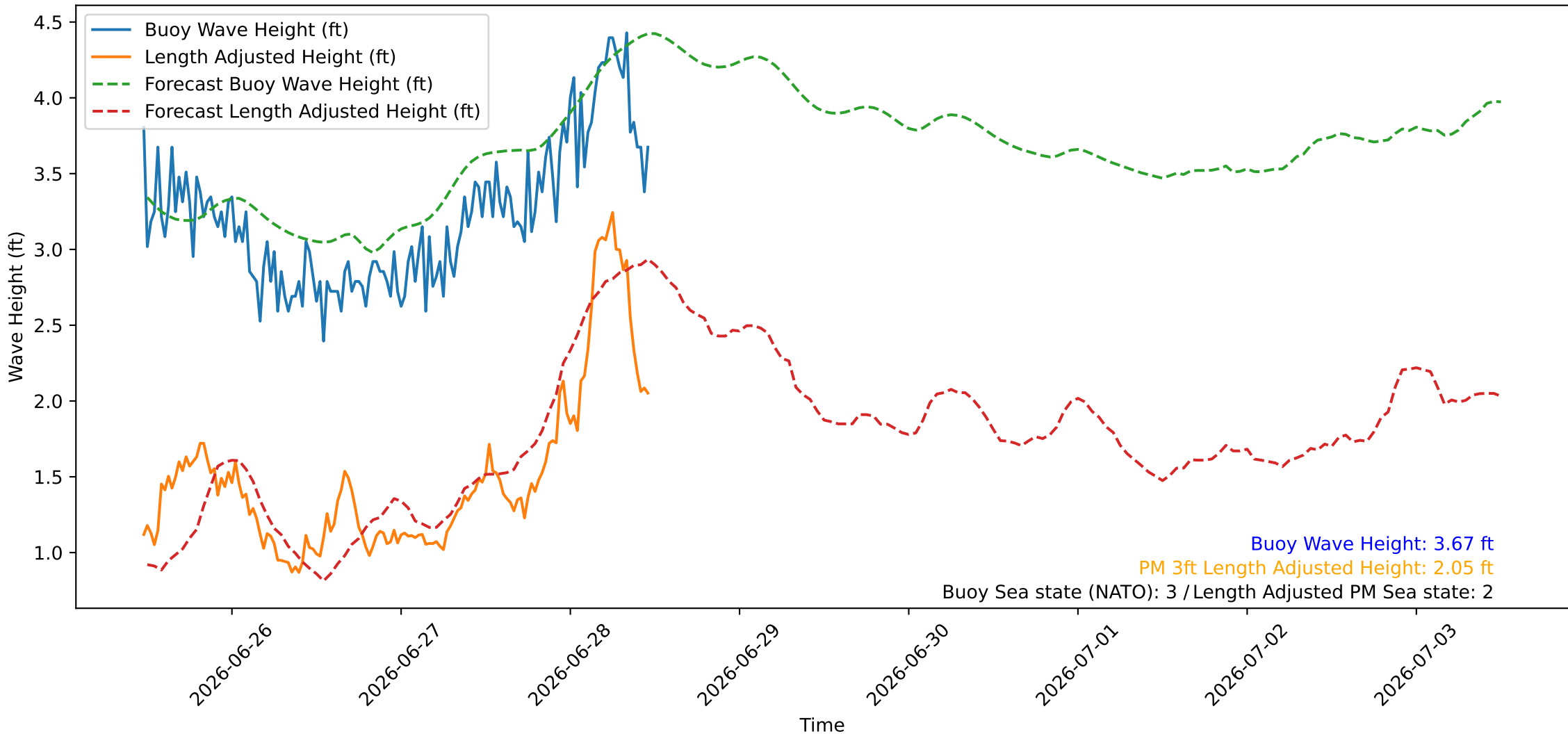
Wave Heights over Time for Oceanside Harbor at 2026-06-28 11:40:25
