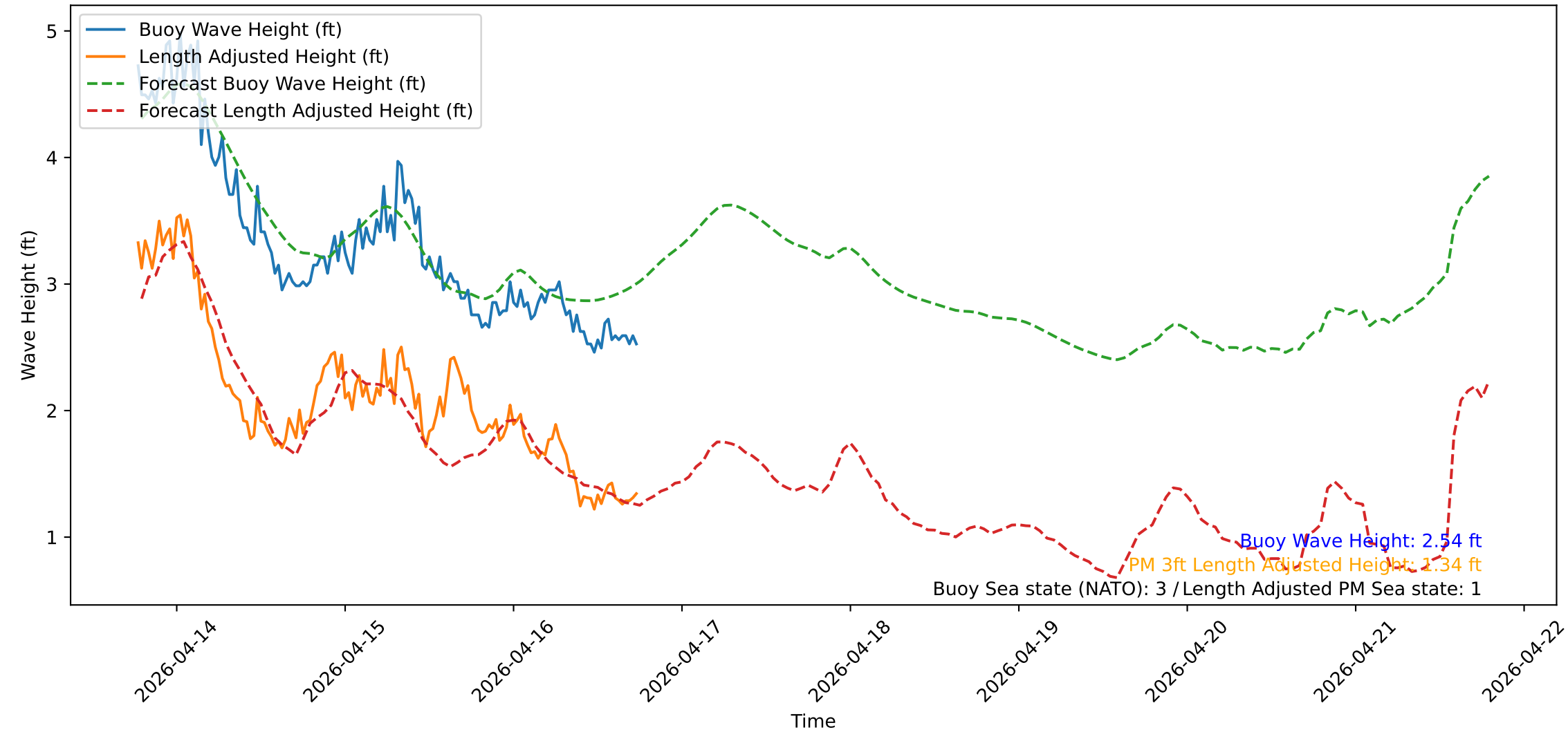
Wave Heights over Time for Green Beach at 2026-04-16 18:31:14
