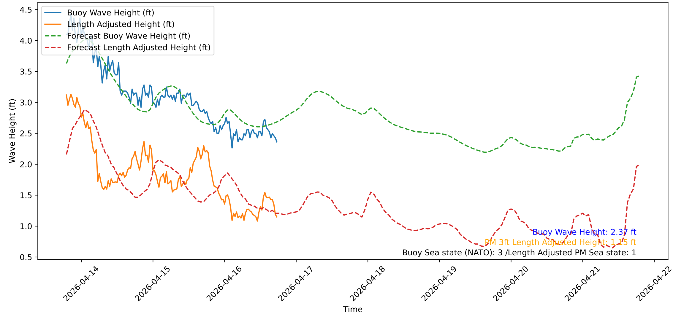
Wave Heights over Time for Red Beach at 2026-04-16 18:30:51
