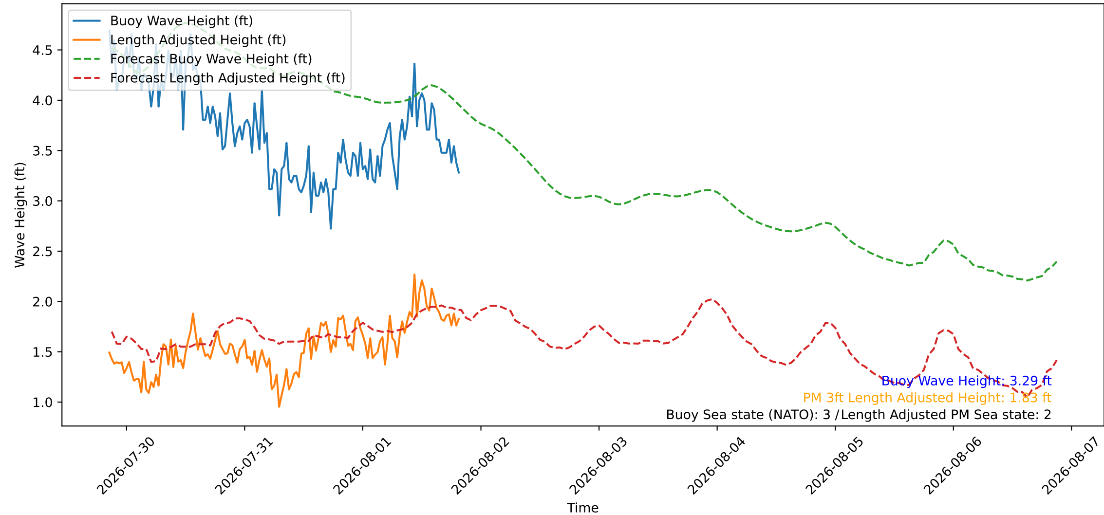
Wave Heights over Time for Oceanside Harbor at 2026-08-01 20:30:26
