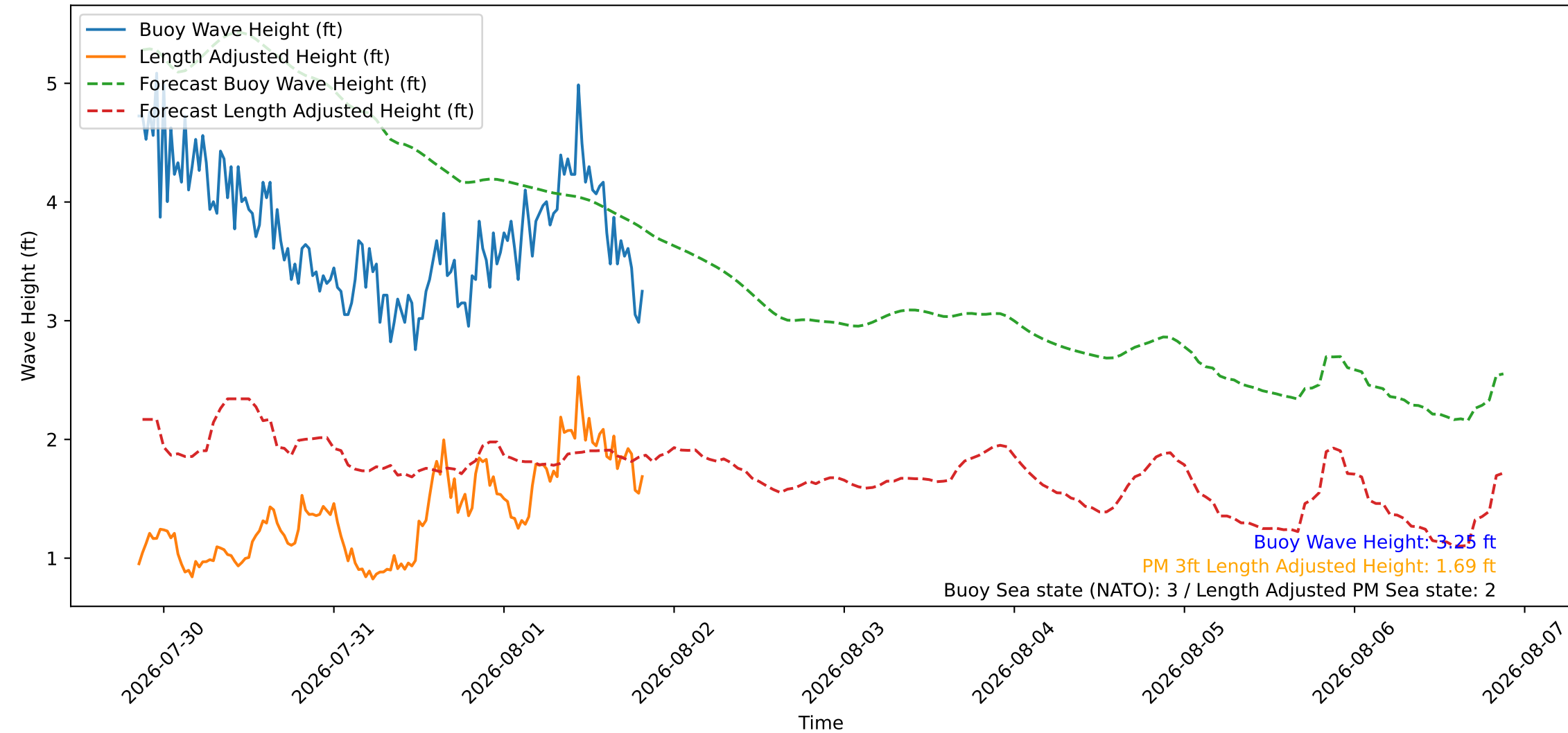
Wave Heights over Time for Green Beach at 2026-08-01 20:31:09
