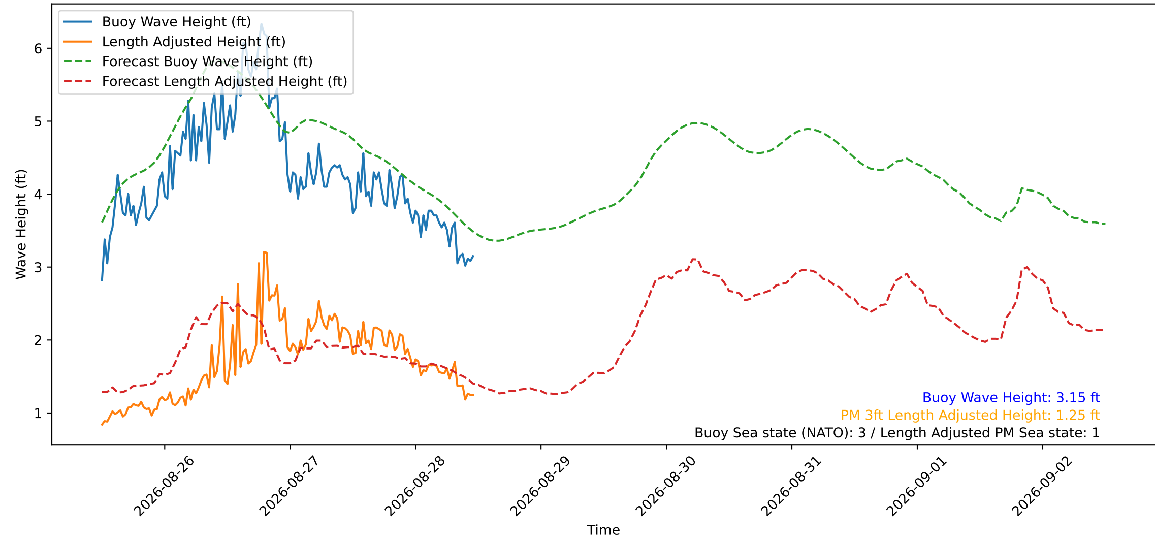
Wave Heights over Time for Green Beach at 2026-08-28 11:41:12
