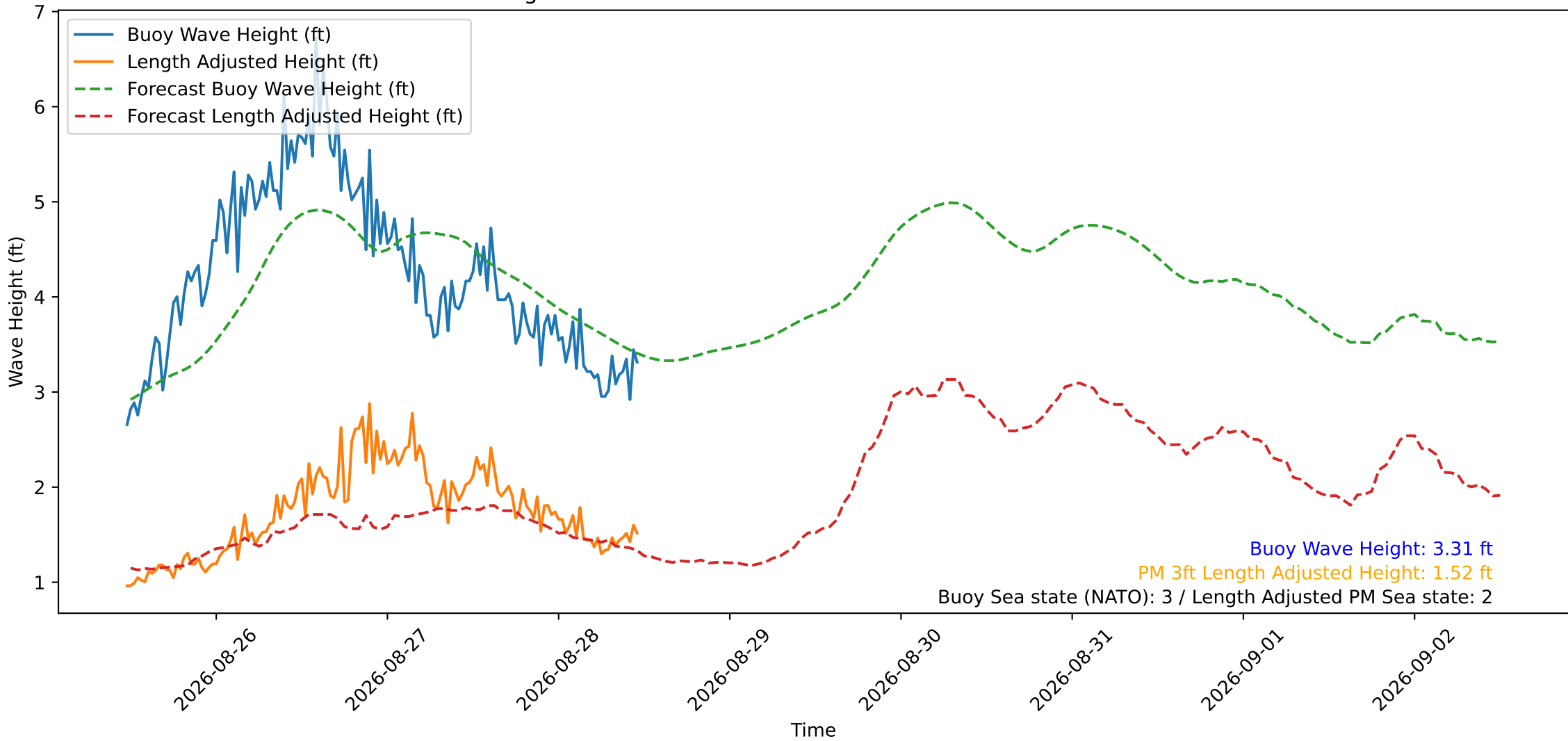
Wave Heights over Time for Oceanside Harbor at 2026-08-28 11:40:29
