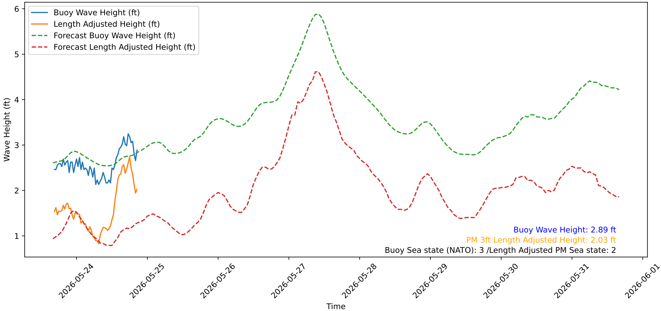
Wave Heights over Time for Oceanside Harbor at 2026-05-26 16:20:27
