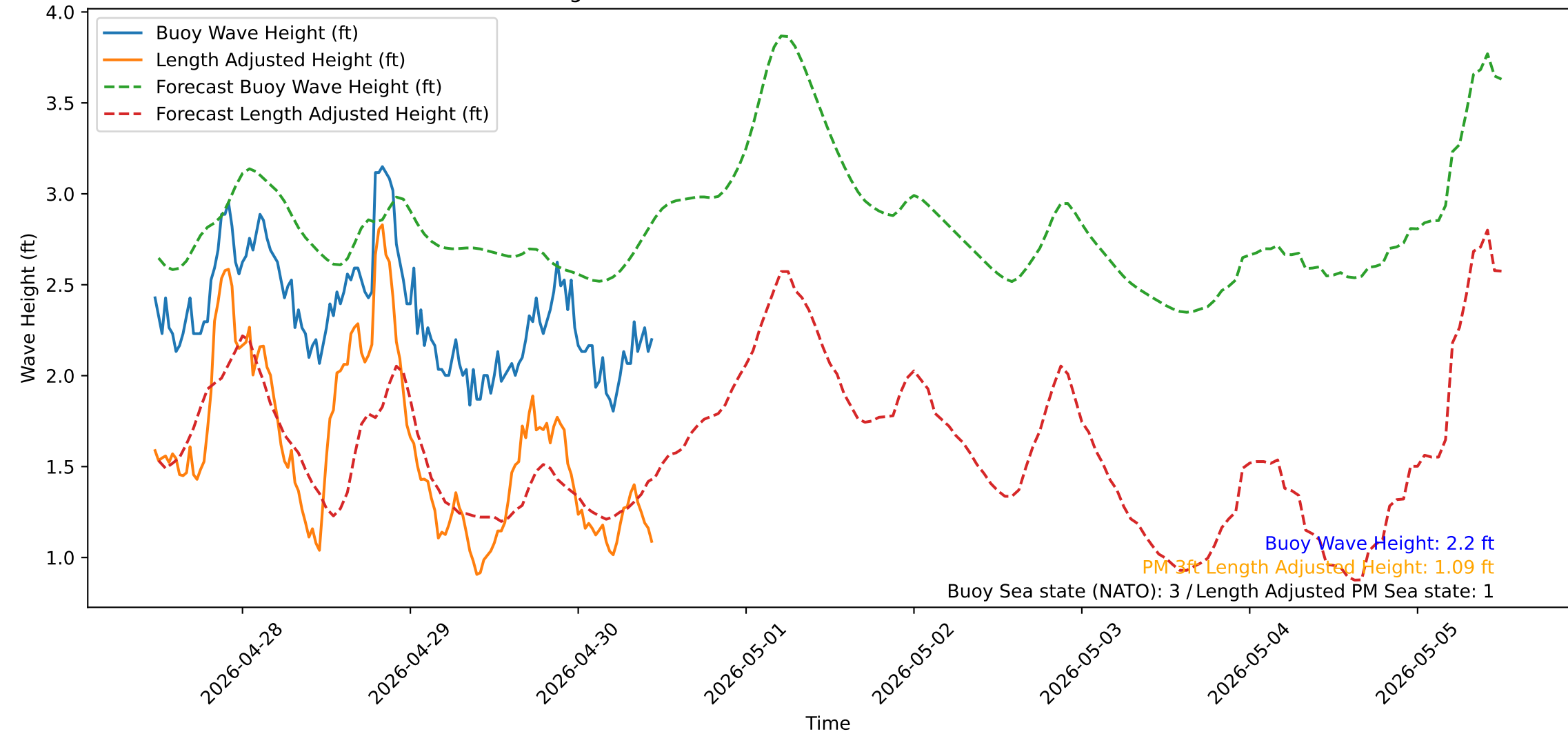
Wave Heights over Time for Green Beach at 2026-04-30 11:31:13
