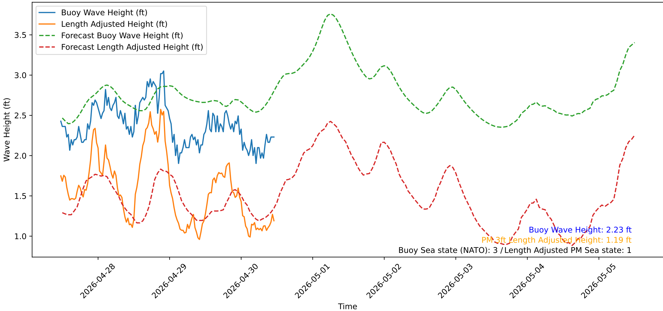
Wave Heights over Time for Oceanside Harbor at 2026-04-30 11:30:31
