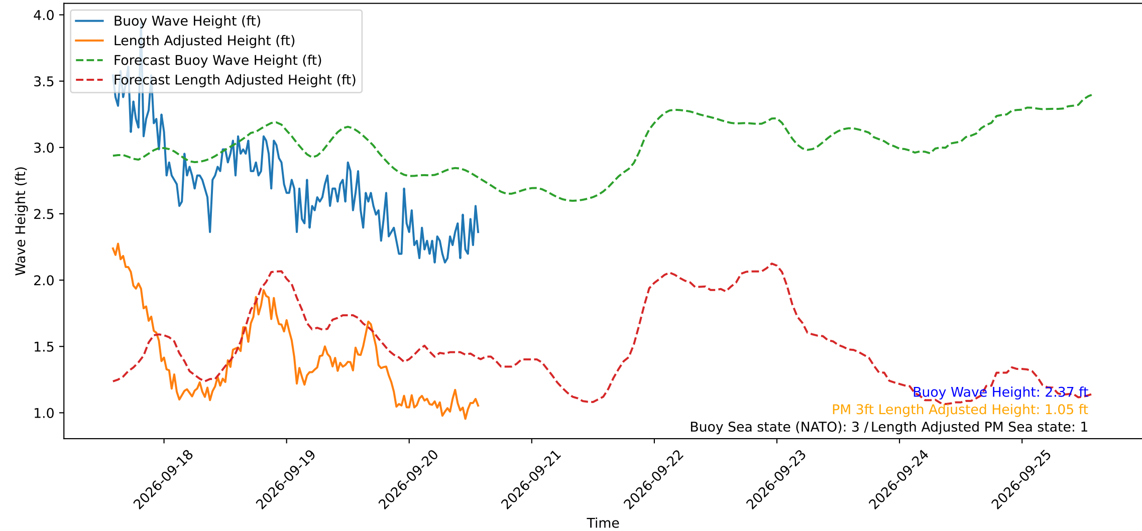
Wave Heights over Time for Oceanside Harbor at 2026-09-20 14:00:29
