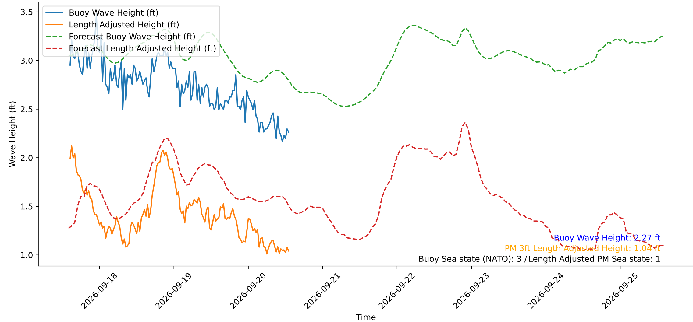
Wave Heights over Time for Green Beach at 2026-09-20 14:01:11
