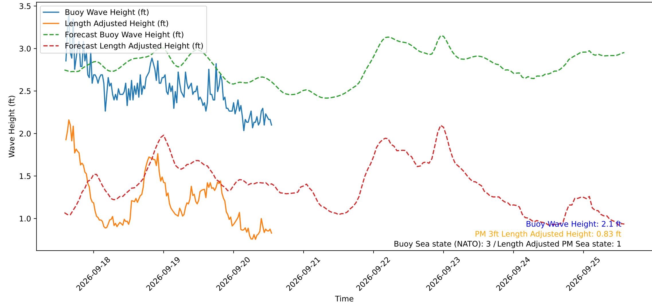
Wave Heights over Time for Red Beach at 2026-09-20 14:00:49
