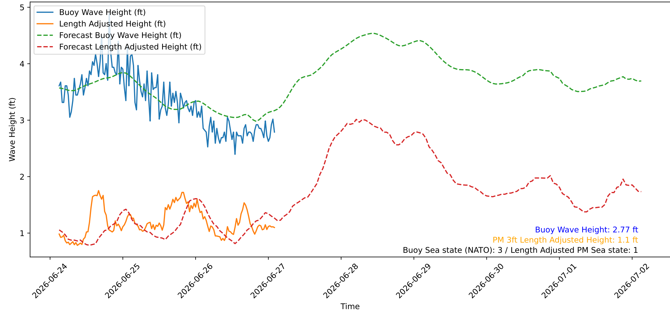
Wave Heights over Time for Oceanside Harbor at 2026-06-27 03:00:26
