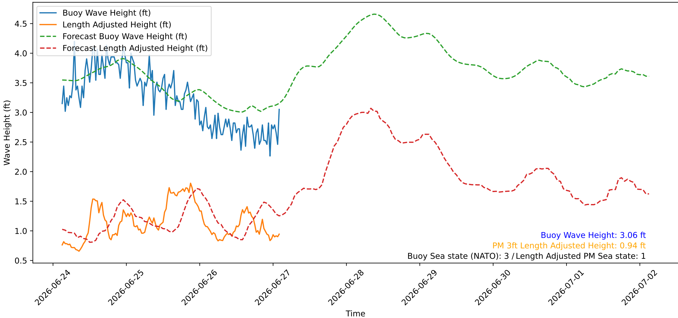
Wave Heights over Time for Green Beach at 2026-06-27 03:01:08
