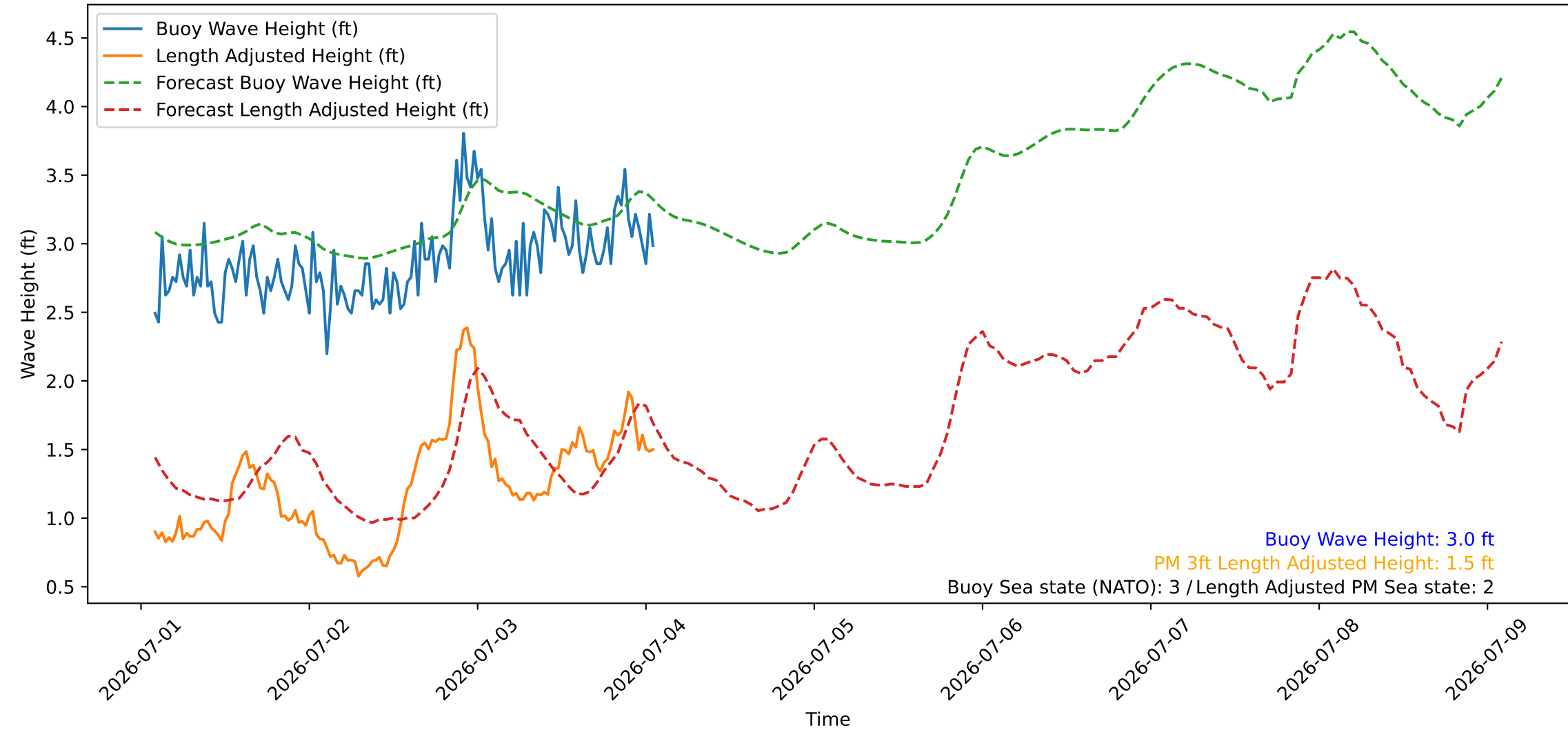
Wave Heights over Time for Red Beach at 2026-07-04 01:50:47
