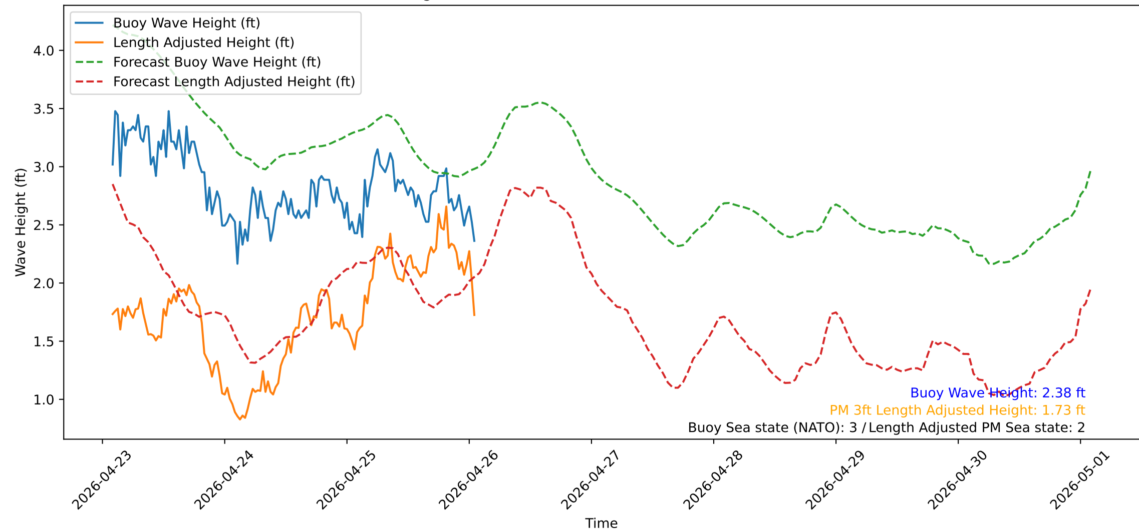
Wave Heights over Time for Red Beach at 2026-04-26 01:50:52
