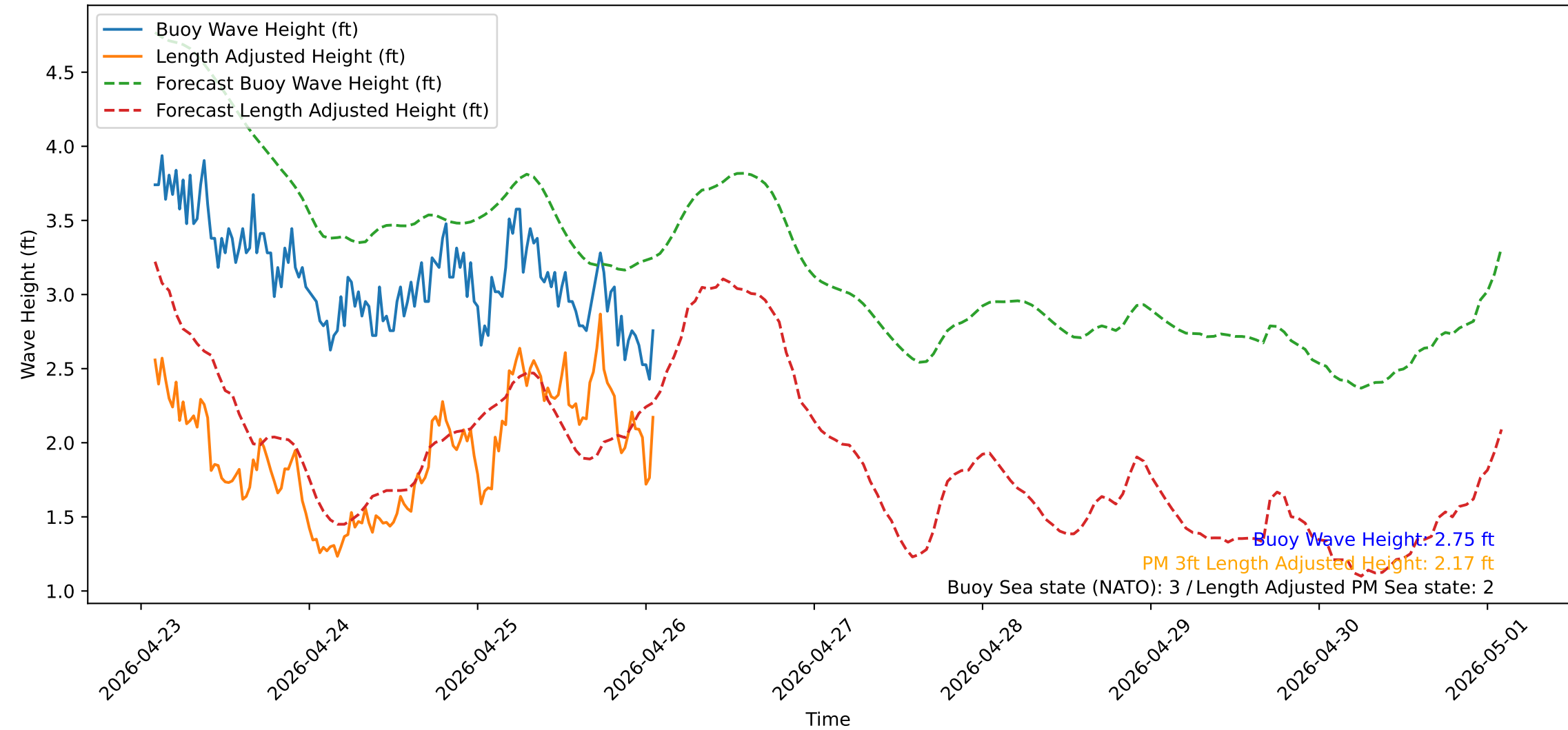
Wave Heights over Time for Green Beach at 2026-04-26 01:51:14
