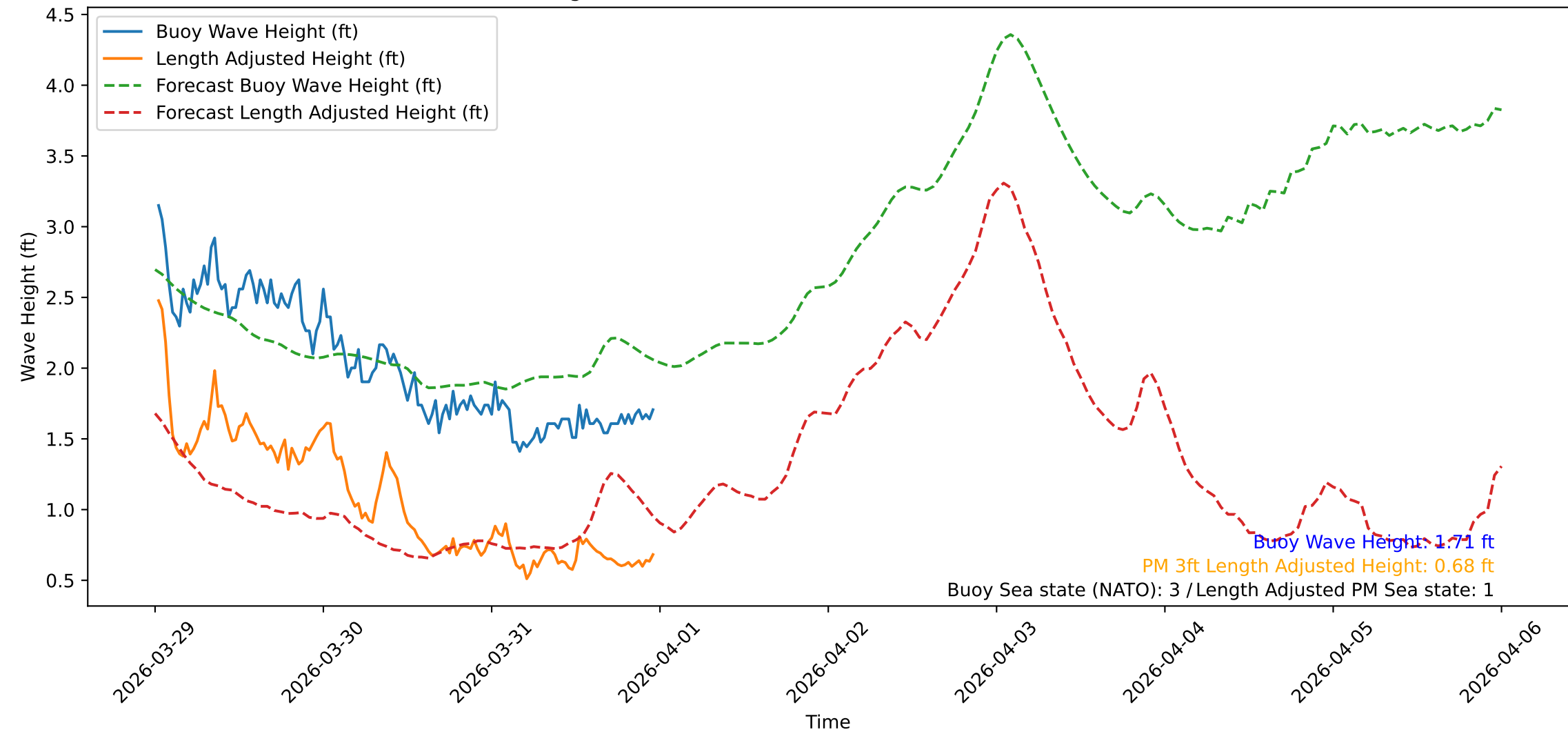
Wave Heights over Time for Green Beach at 2026-04-01 00:21:09
