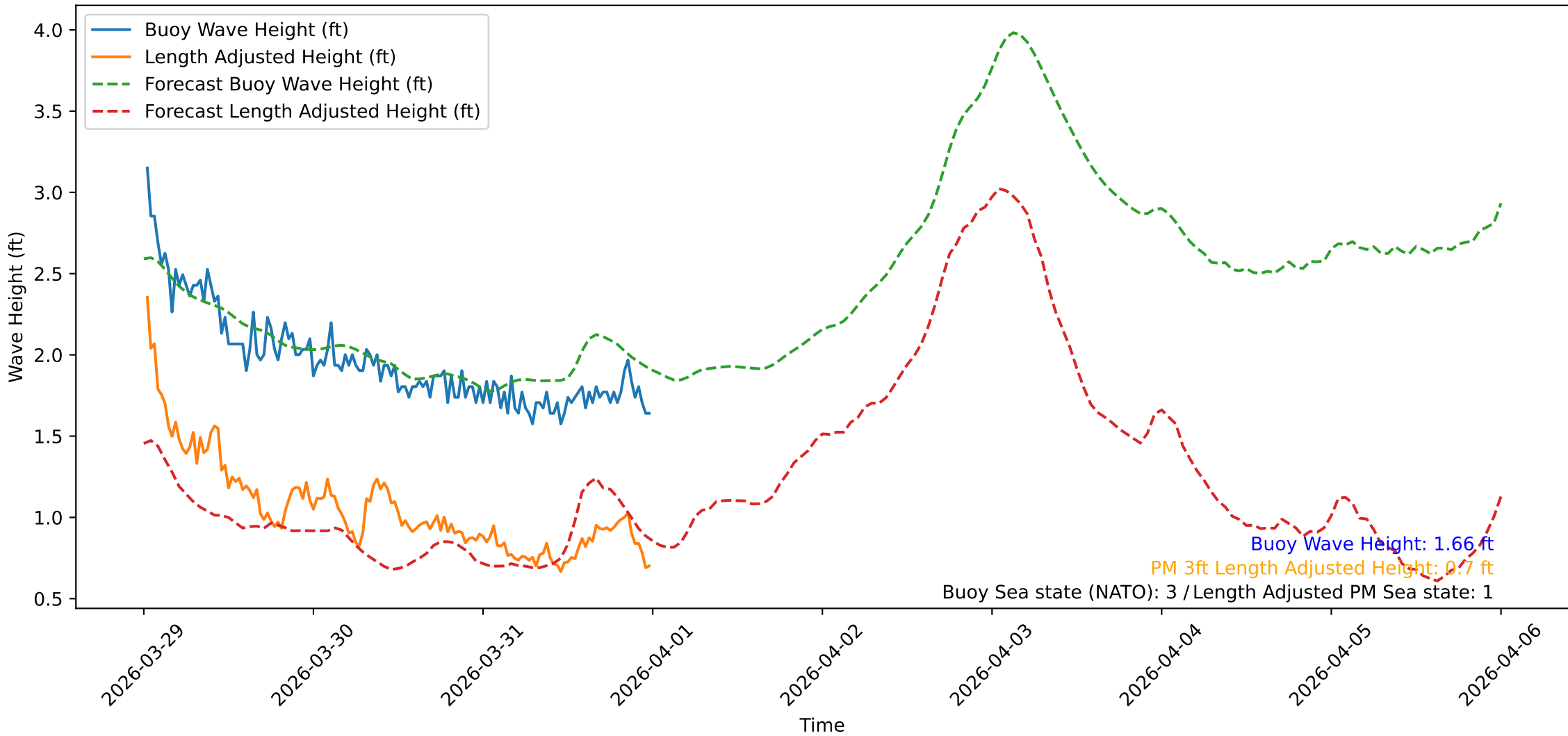
Wave Heights over Time for Oceanside Harbor at 2026-04-01 00:20:31
