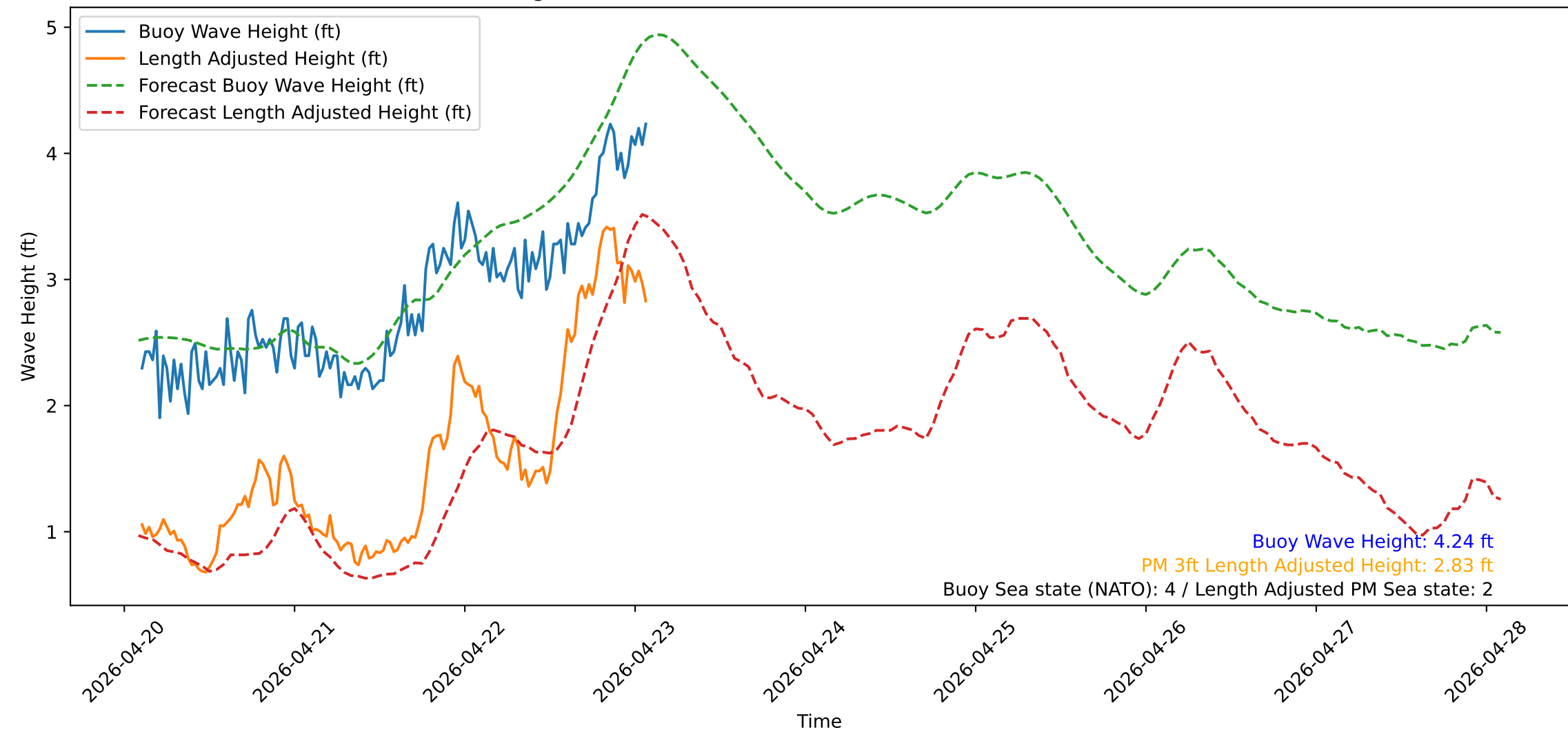
Wave Heights over Time for Oceanside Harbor at 2026-04-23 02:20:31
