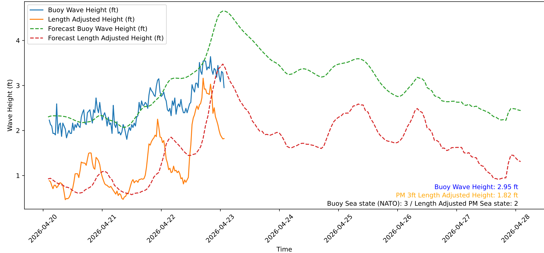
Wave Heights over Time for Red Beach at 2026-04-23 02:20:51
