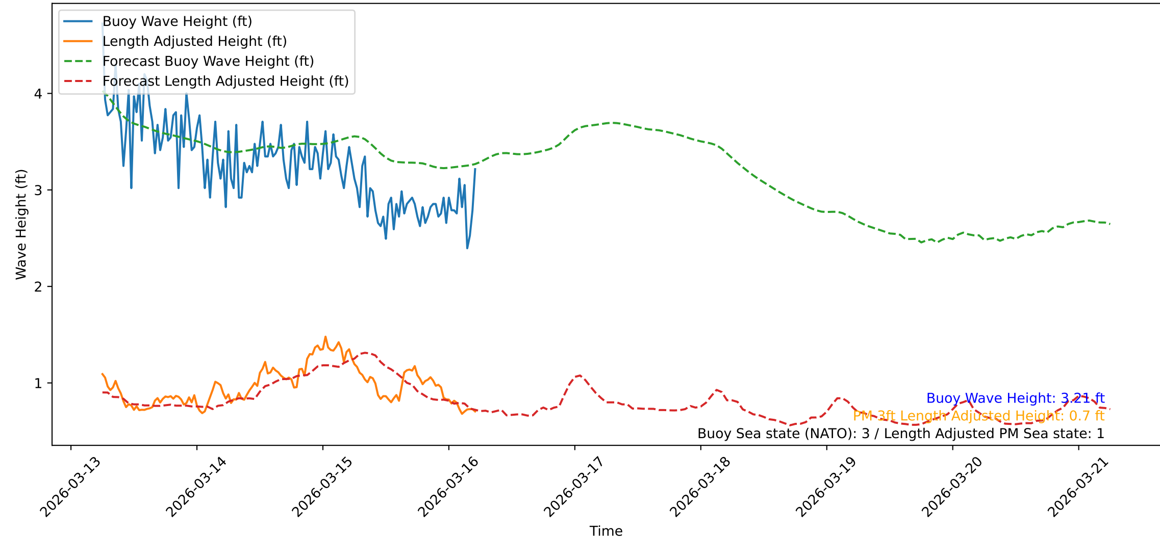
Wave Heights over Time for Oceanside Harbor at 2026-03-16 05:50:43
