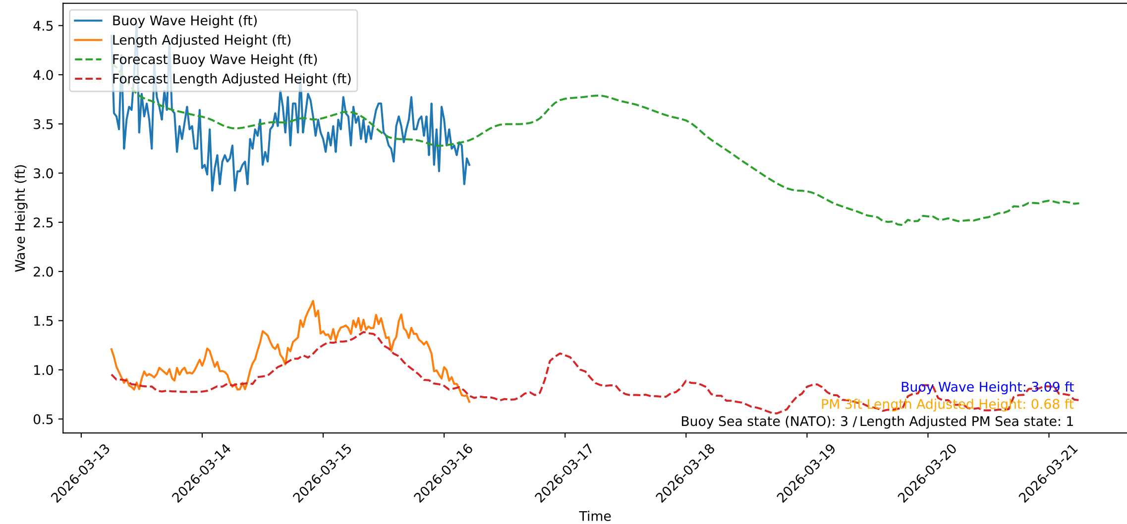
Wave Heights over Time for Green Beach at 2026-03-16 05:52:10
