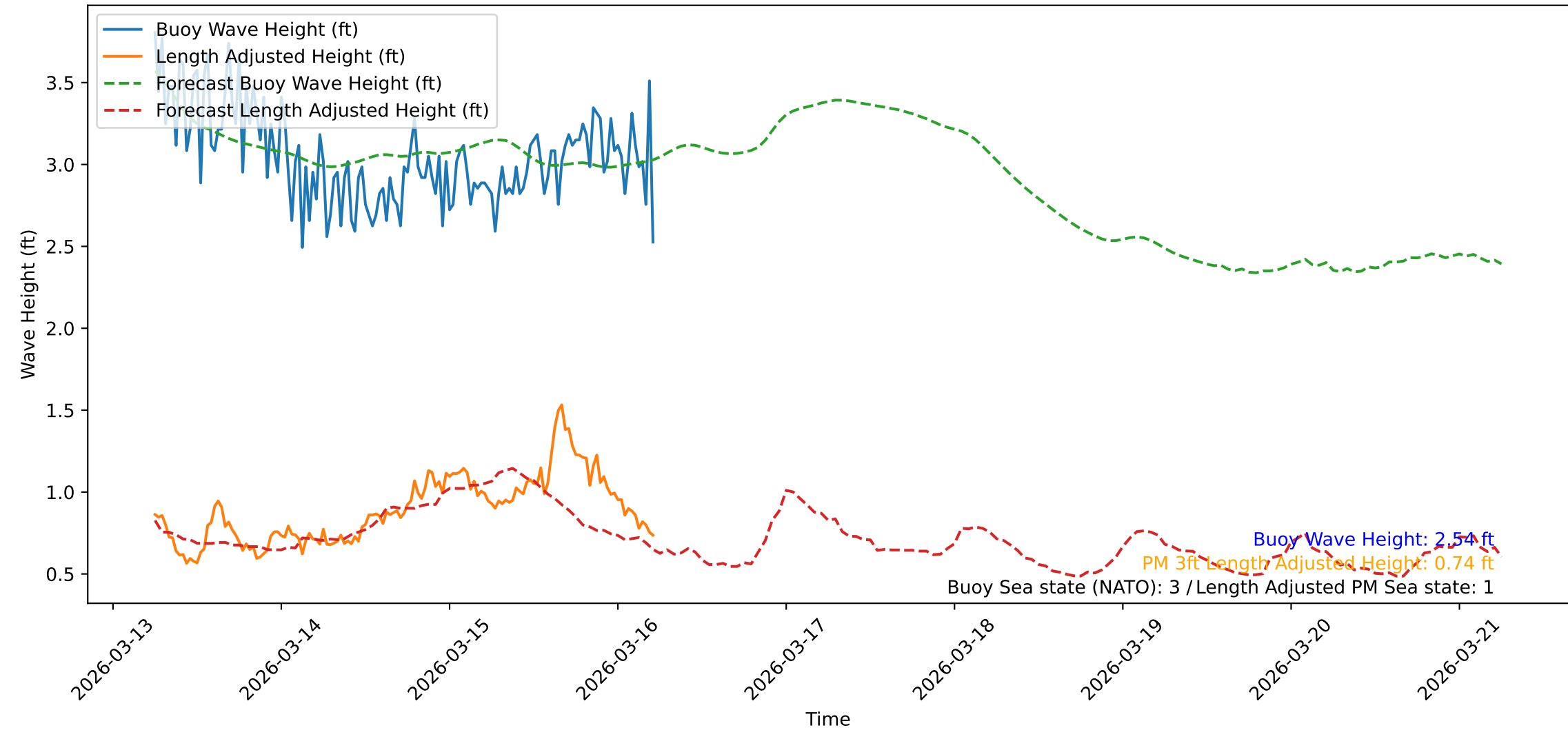
Wave Heights over Time for Red Beach at 2026-03-16 05:51:24
