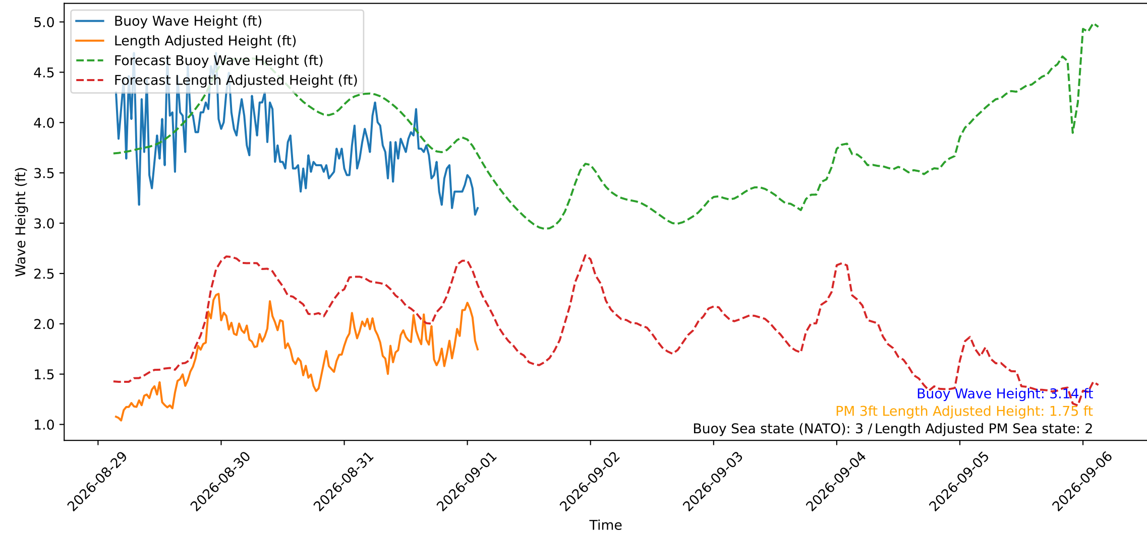
Wave Heights over Time for Red Beach at 2026-09-01 03:00:50
