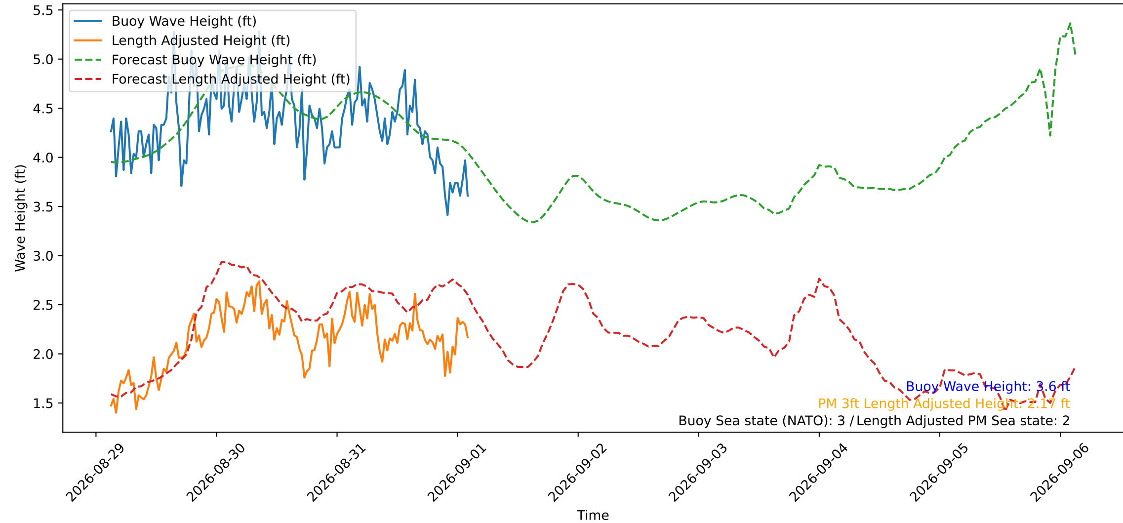
Wave Heights over Time for Oceanside Harbor at 2026-09-01 03:00:30
