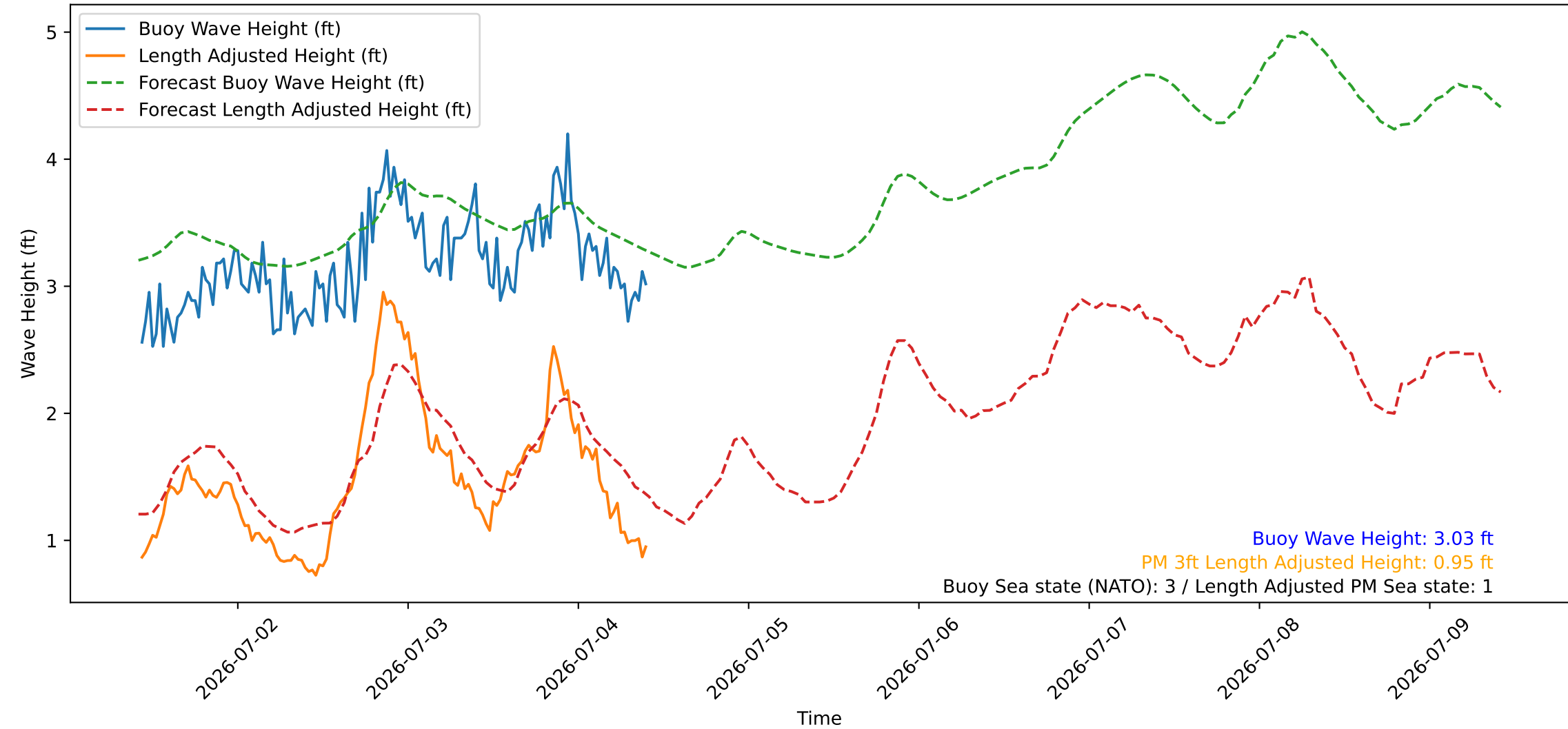
Wave Heights over Time for Green Beach at 2026-07-04 10:21:08
