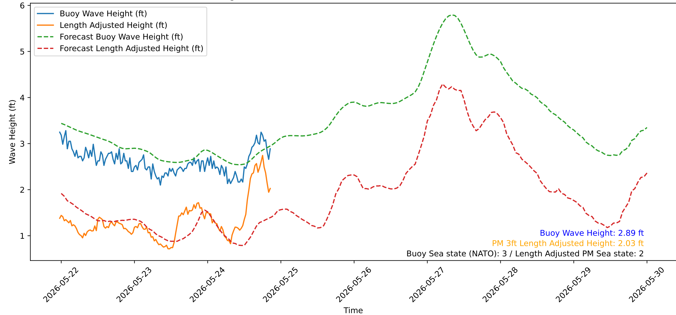
Wave Heights over Time for Oceanside Harbor at 2026-05-24 23:40:31
