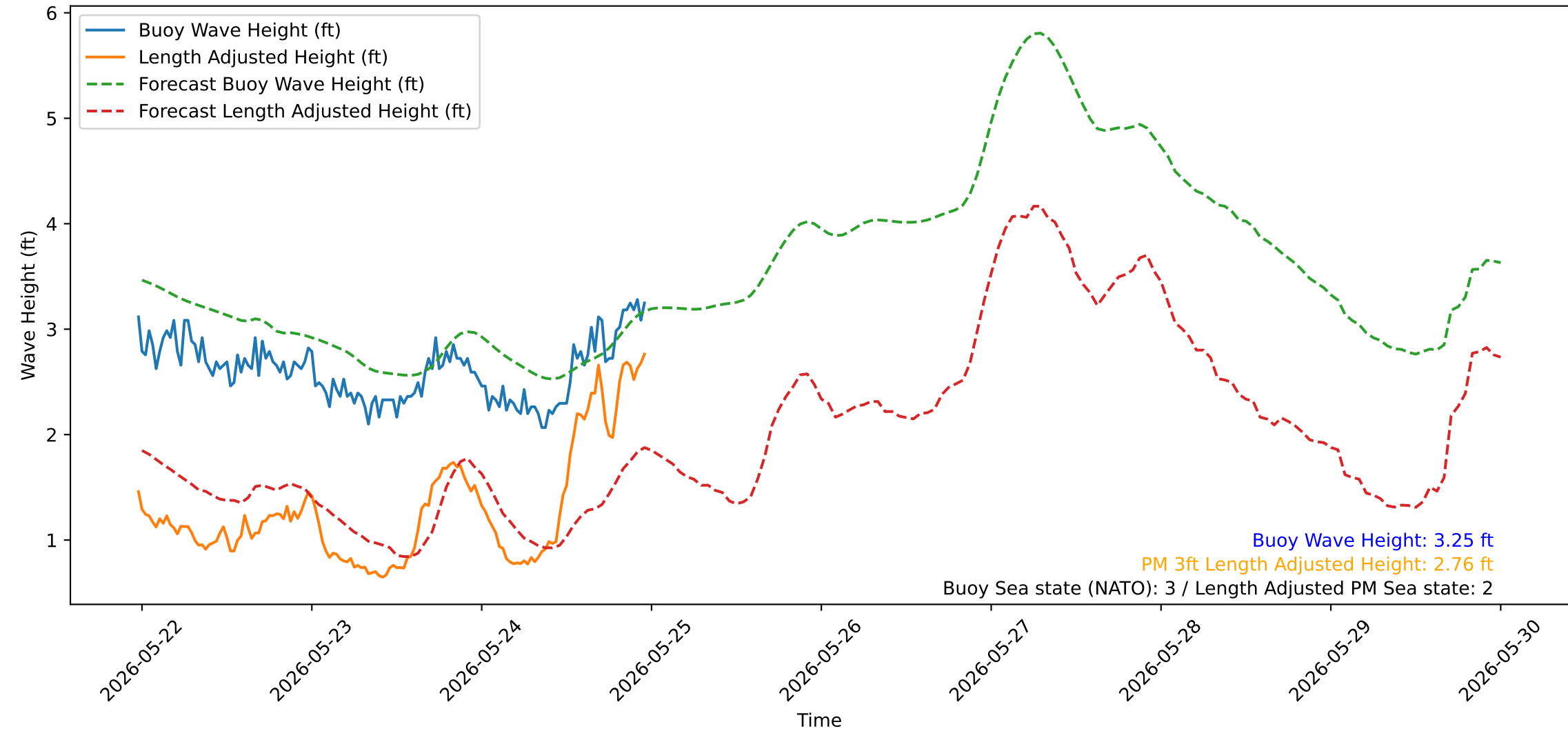
Wave Heights over Time for Green Beach at 2026-05-24 23:41:13
