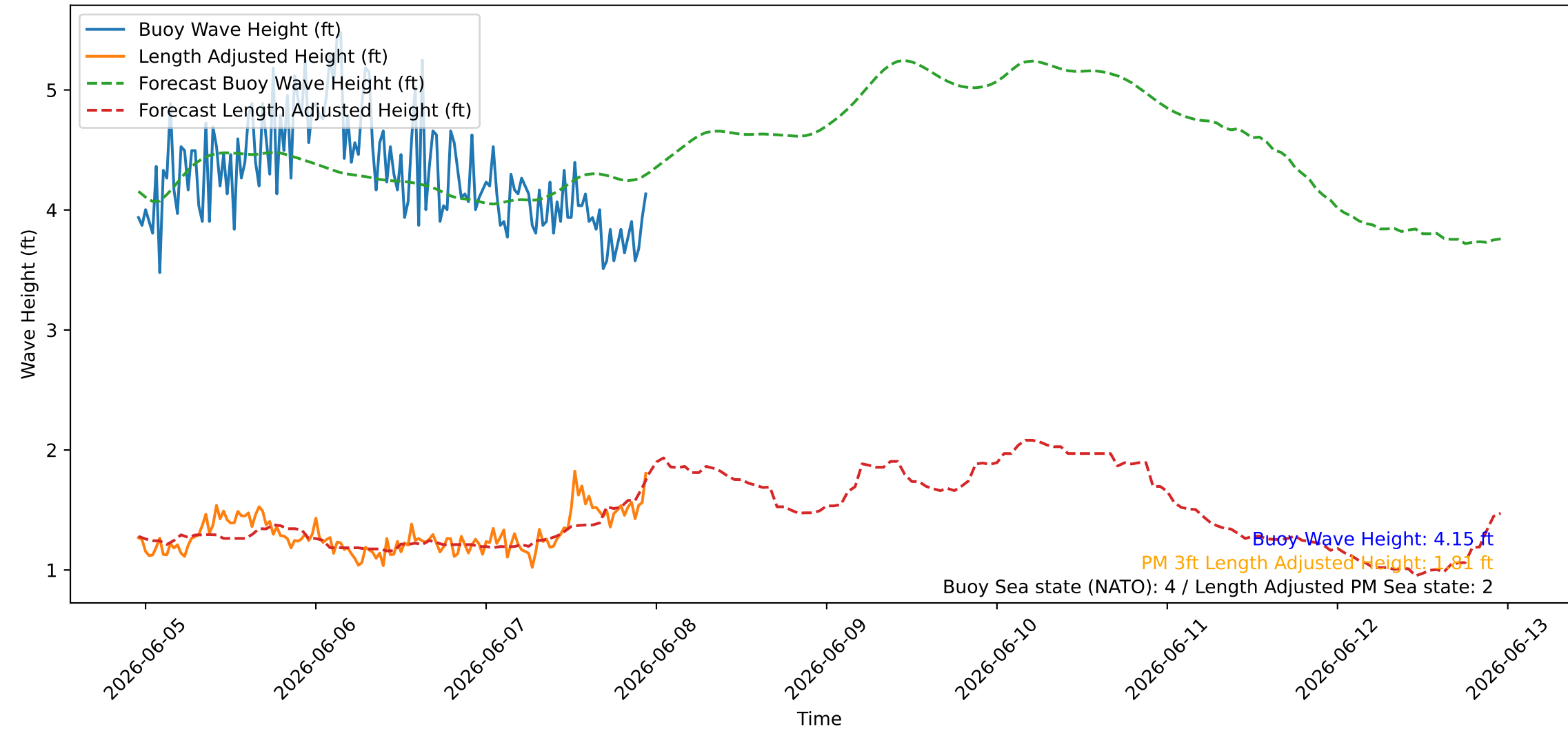
Wave Heights over Time for Oceanside Harbor at 2026-06-07 23:10:27
