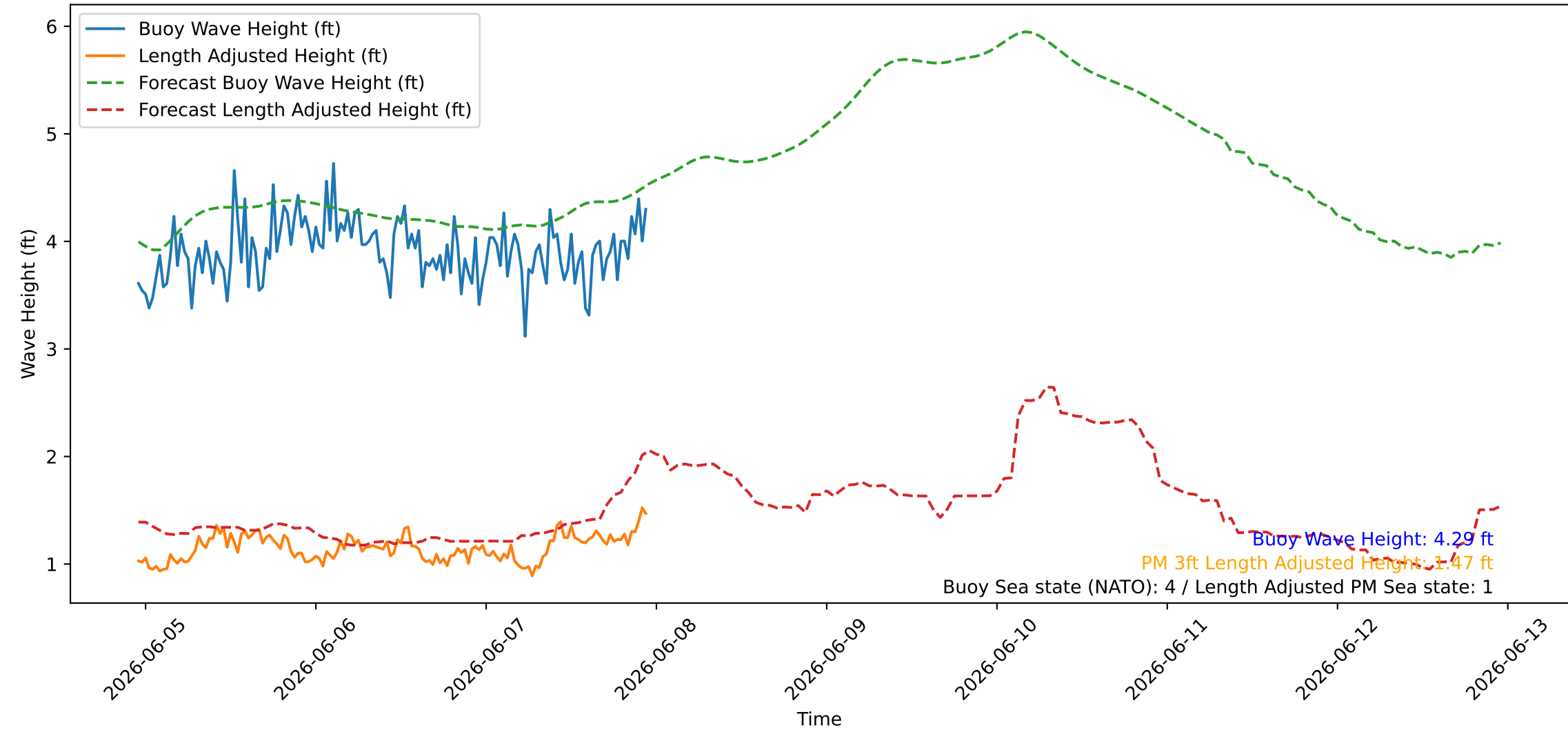
Wave Heights over Time for Green Beach at 2026-06-07 23:11:08
