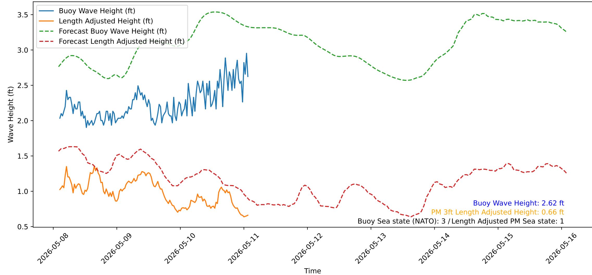
Wave Heights over Time for Red Beach at 2026-05-11 02:20:51
