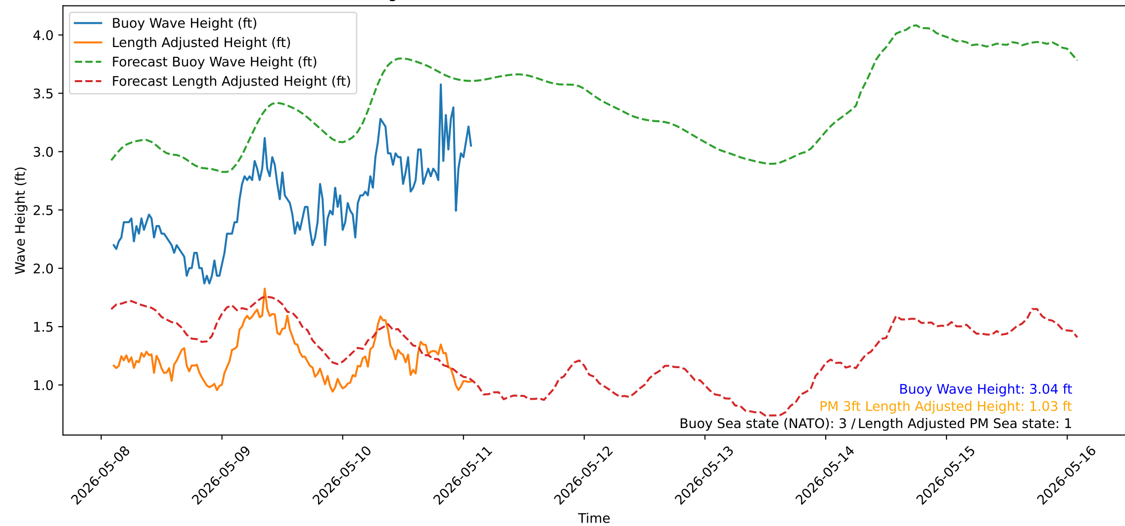
Wave Heights over Time for Oceanside Harbor at 2026-05-11 02:20:30
