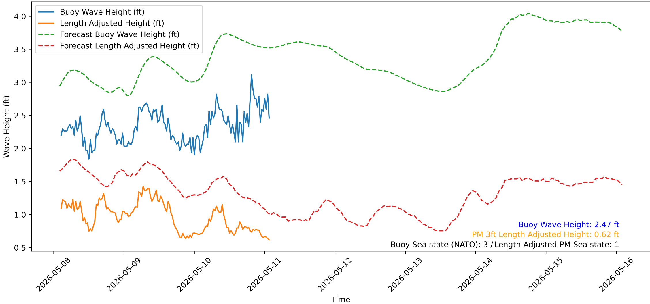
Wave Heights over Time for Green Beach at 2026-05-11 02:21:13
