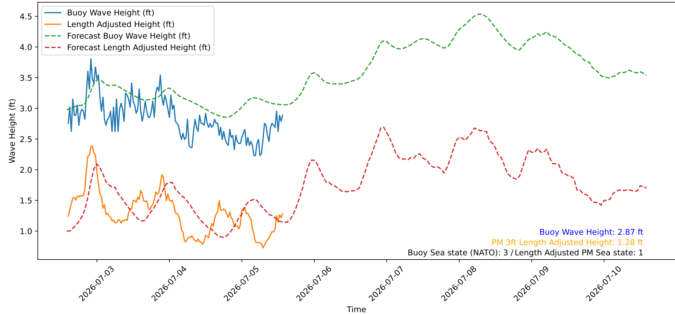
Wave Heights over Time for Red Beach at 2026-07-05 14:10:46
