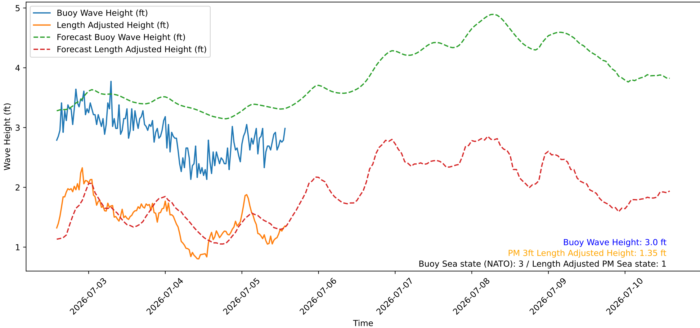
Wave Heights over Time for Oceanside Harbor at 2026-07-05 14:10:26
