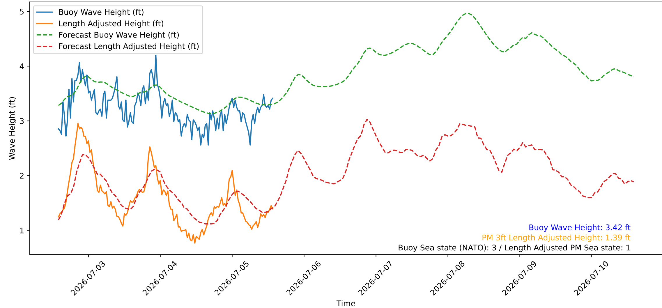
Wave Heights over Time for Green Beach at 2026-07-05 14:11:09
