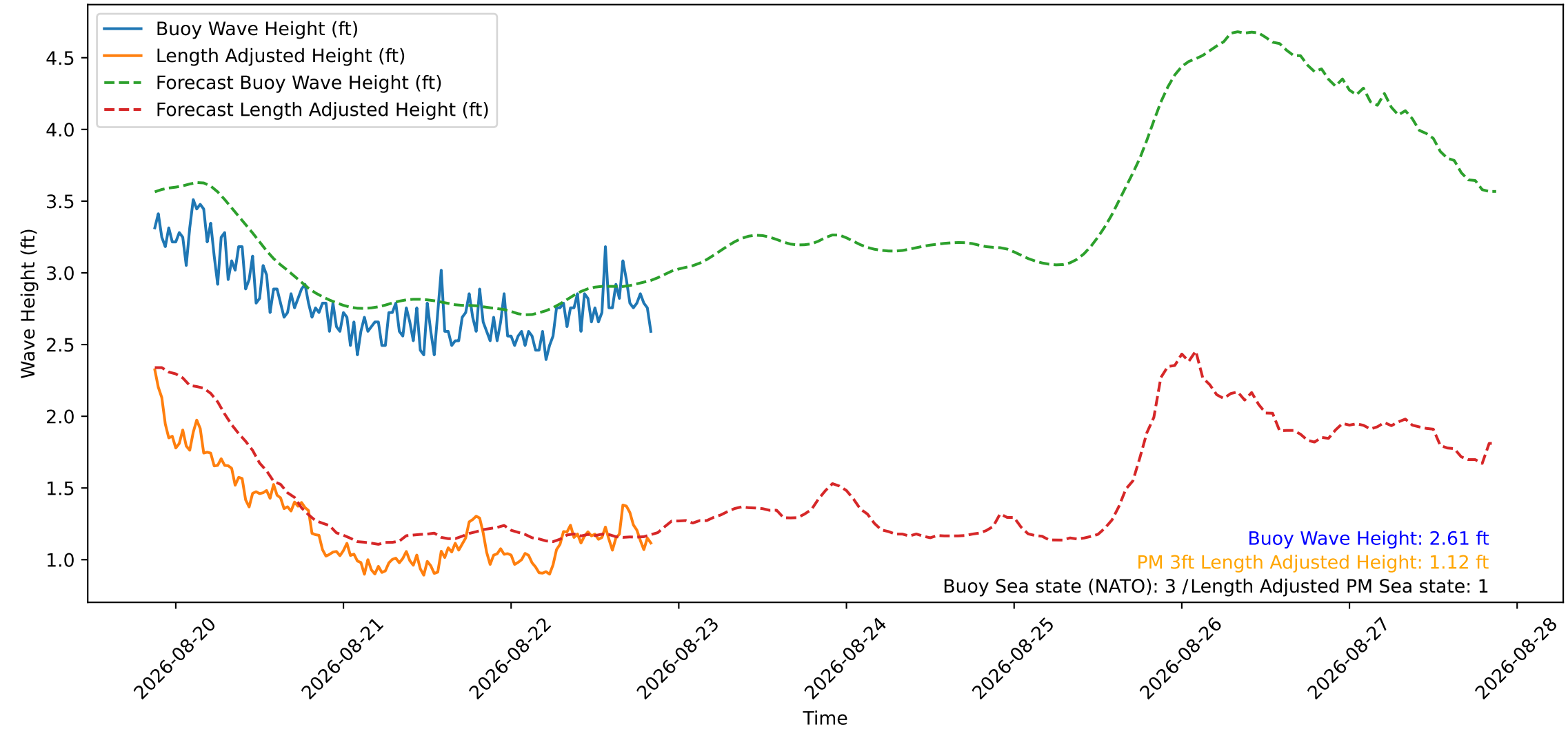
Wave Heights over Time for Green Beach at 2026-08-22 20:41:12
