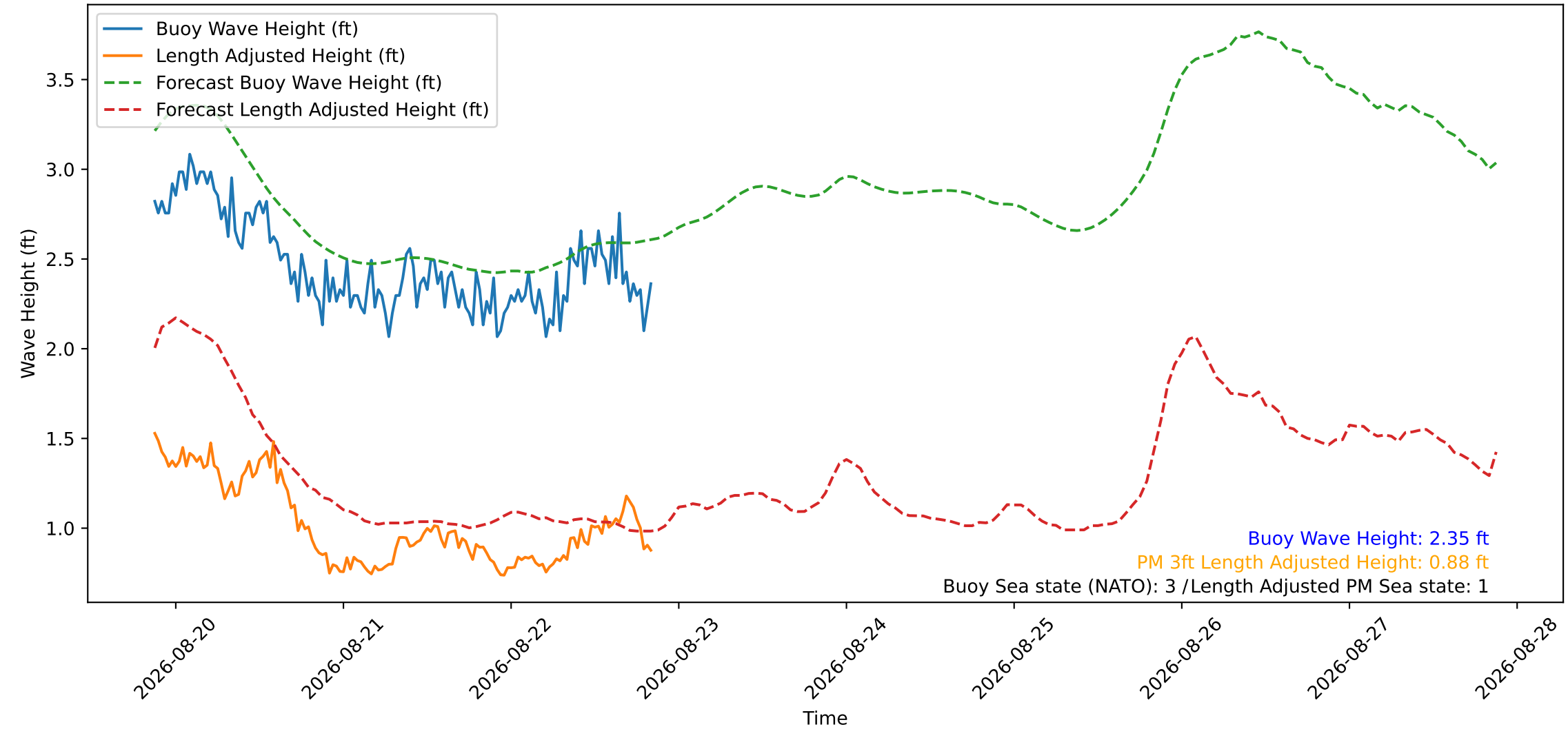
Wave Heights over Time for Red Beach at 2026-08-22 20:40:49
