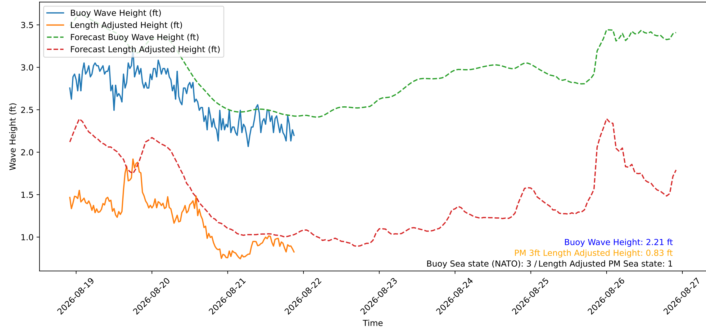
Wave Heights over Time for Red Beach at 2026-08-21 21:40:49
