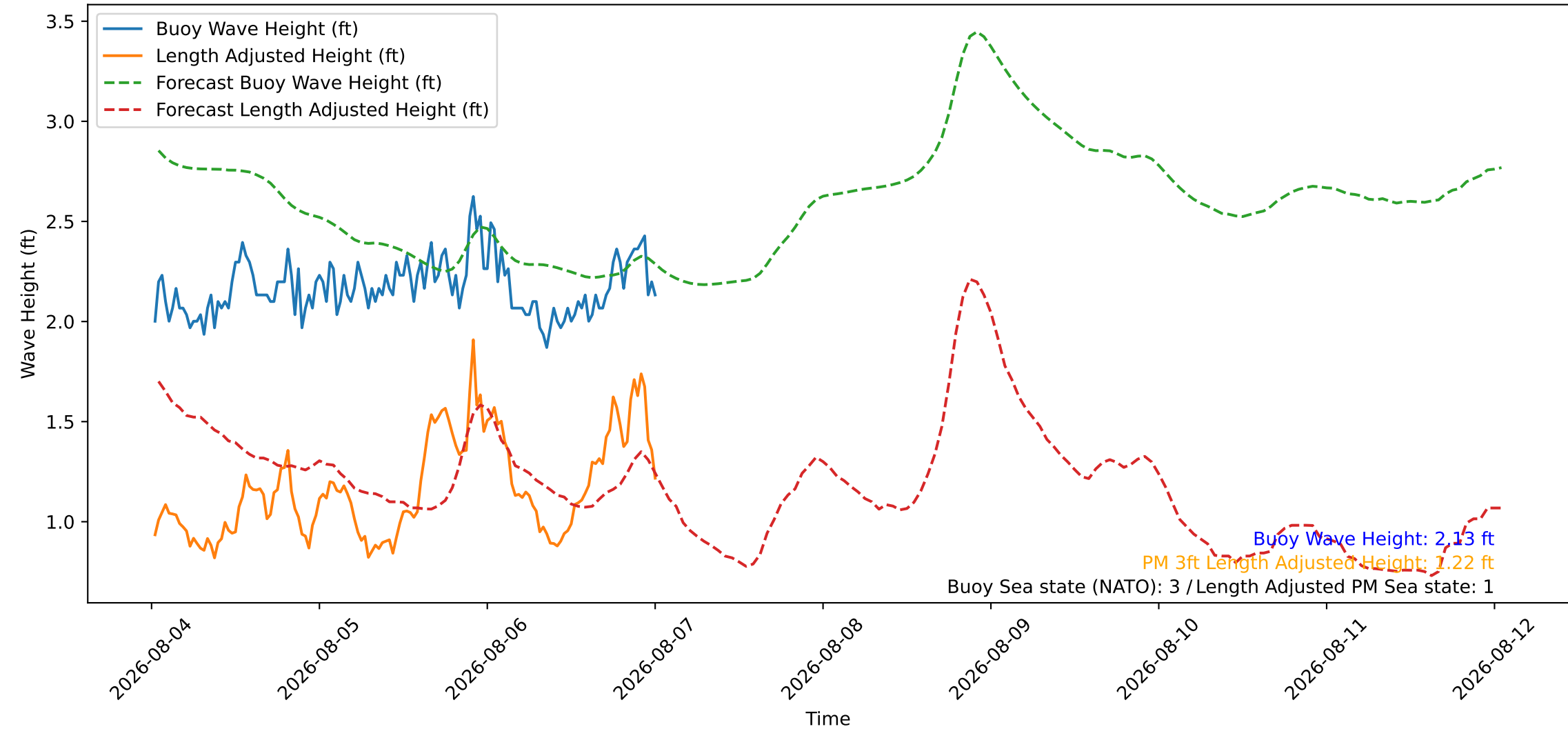
Wave Heights over Time for Green Beach at 2026-08-07 00:41:07
