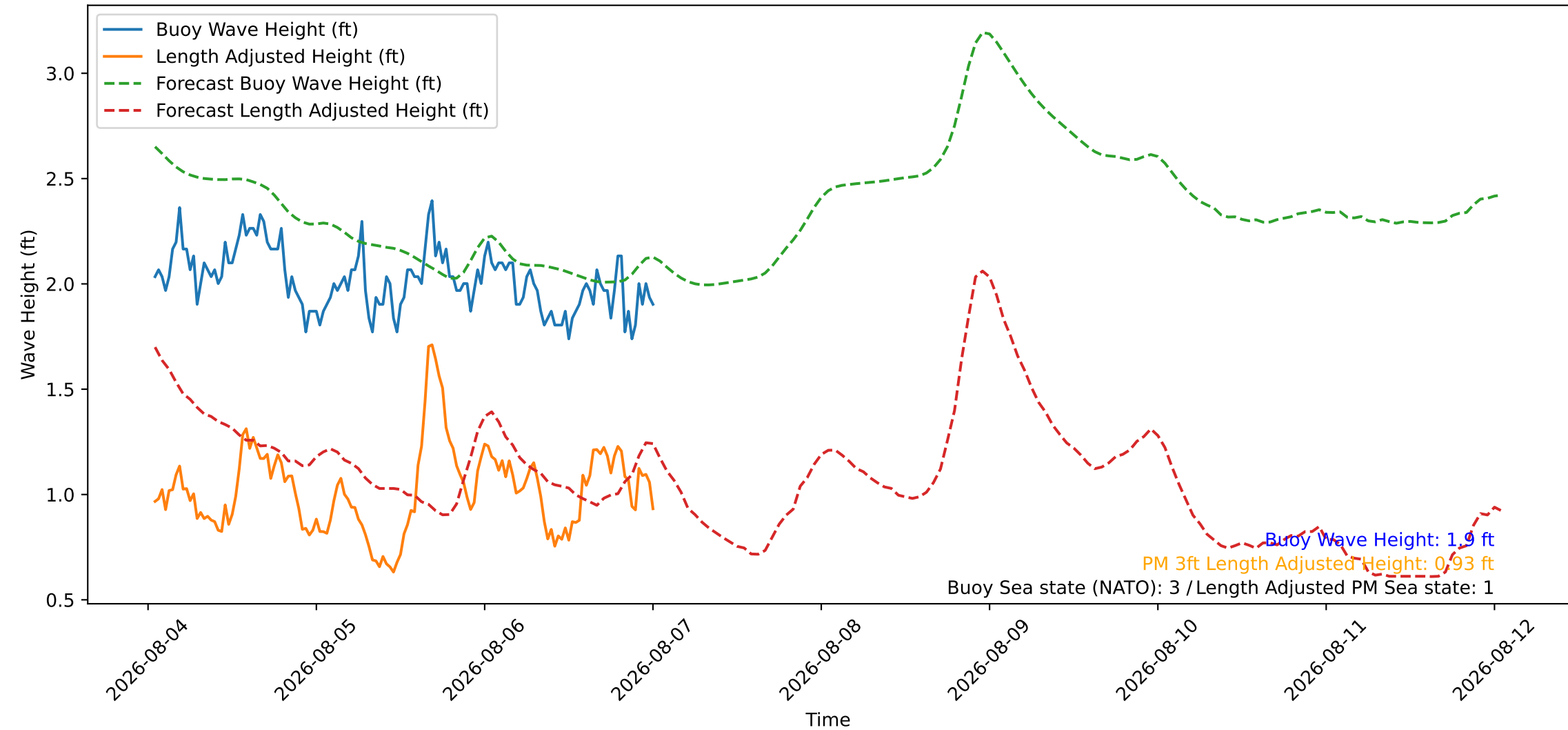
Wave Heights over Time for Red Beach at 2026-08-07 00:40:45
