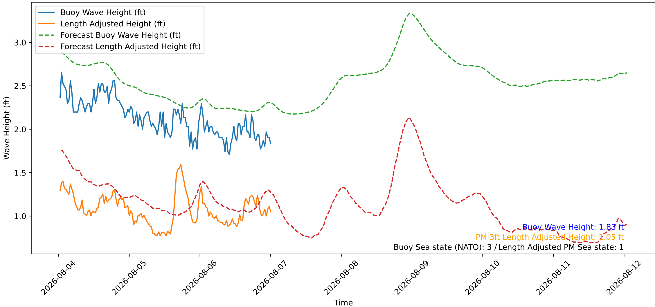
Wave Heights over Time for Oceanside Harbor at 2026-08-07 00:40:26
