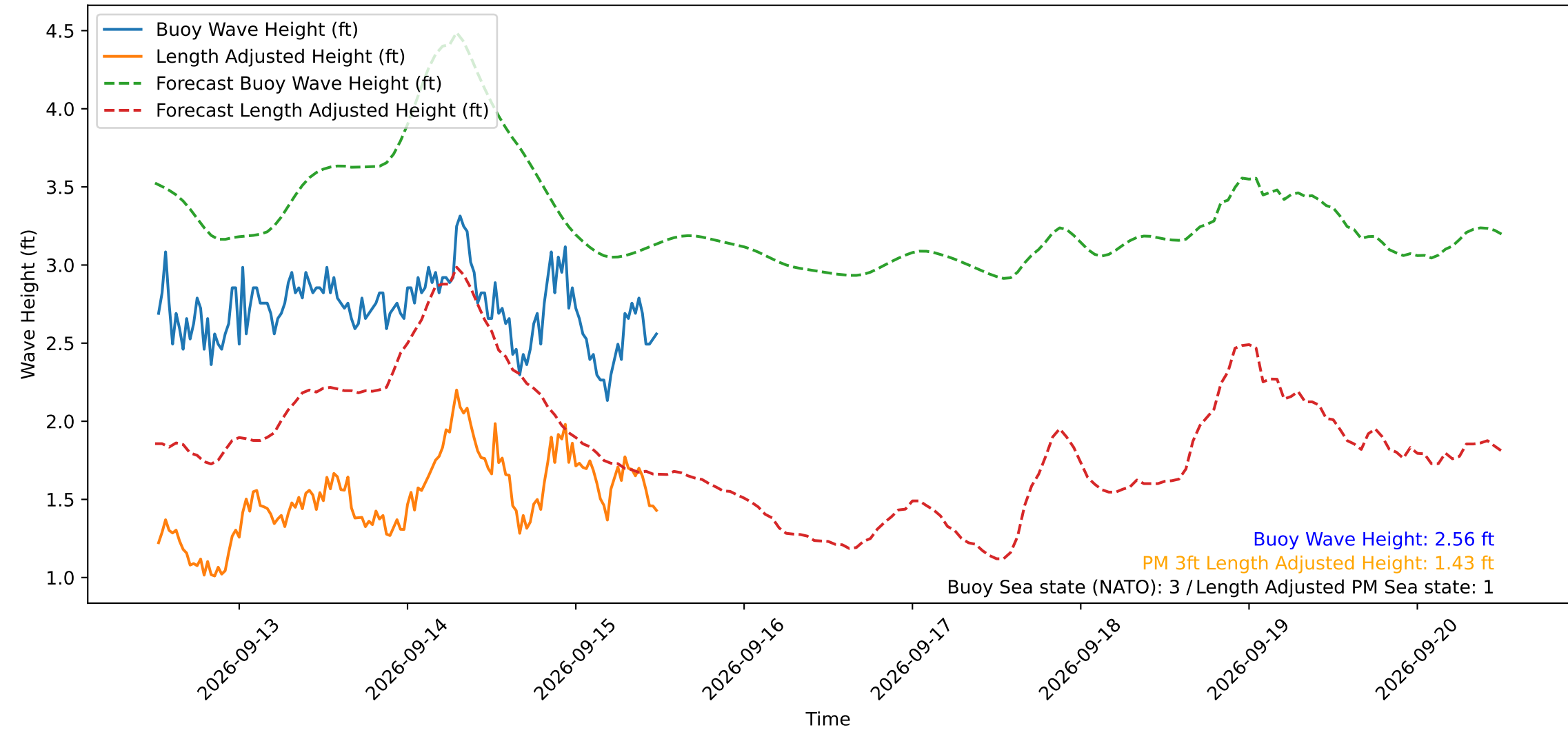
Wave Heights over Time for Green Beach at 2026-09-15 12:11:12
