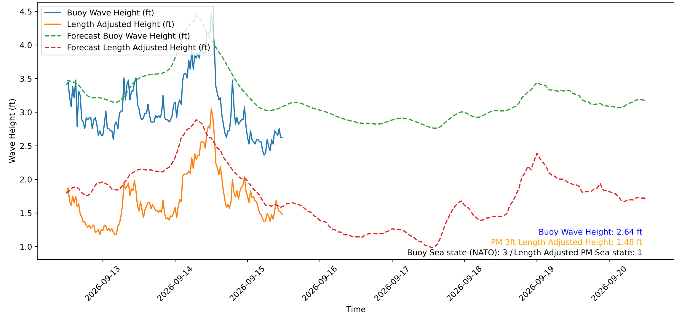
Wave Heights over Time for Oceanside Harbor at 2026-09-15 12:10:30
