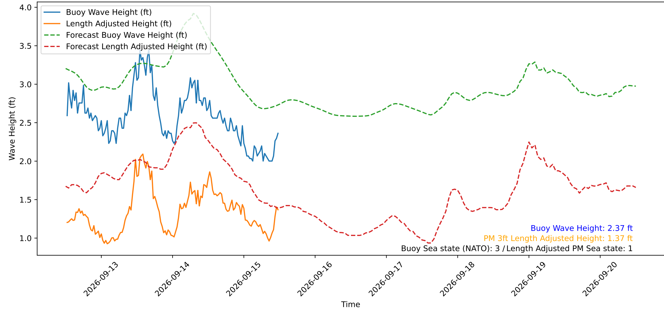
Wave Heights over Time for Red Beach at 2026-09-15 12:10:50
