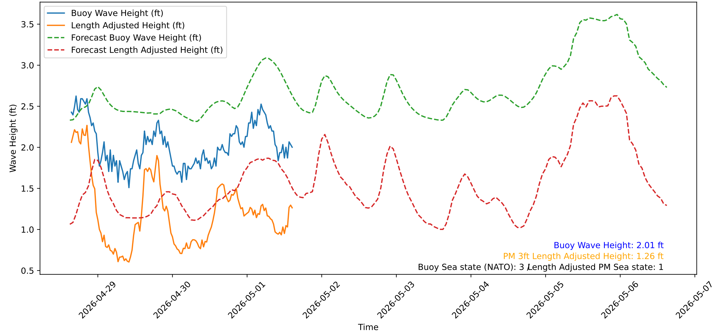
Wave Heights over Time for Red Beach at 2026-05-01 15:10:51
