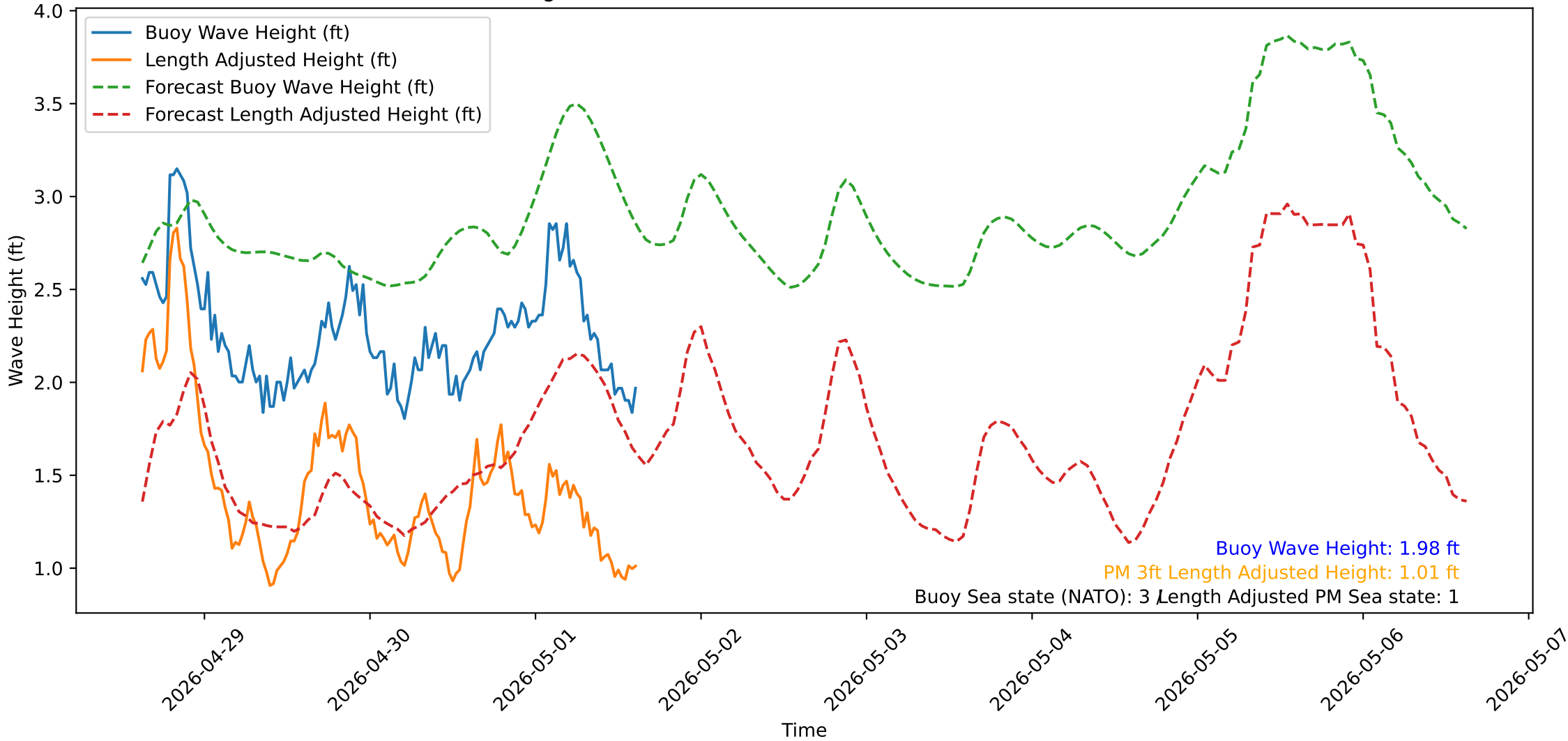
Wave Heights over Time for Green Beach at 2026-05-01 15:11:14
