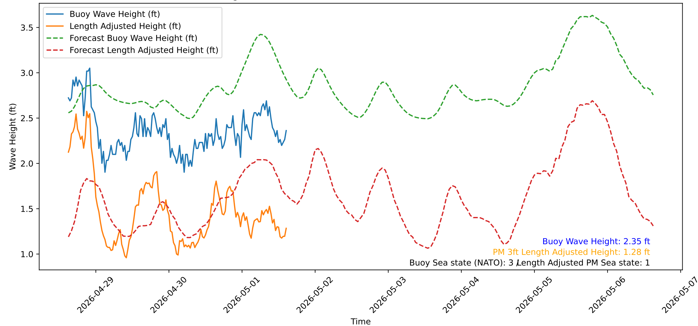
Wave Heights over Time for Oceanside Harbor at 2026-05-01 15:10:31
