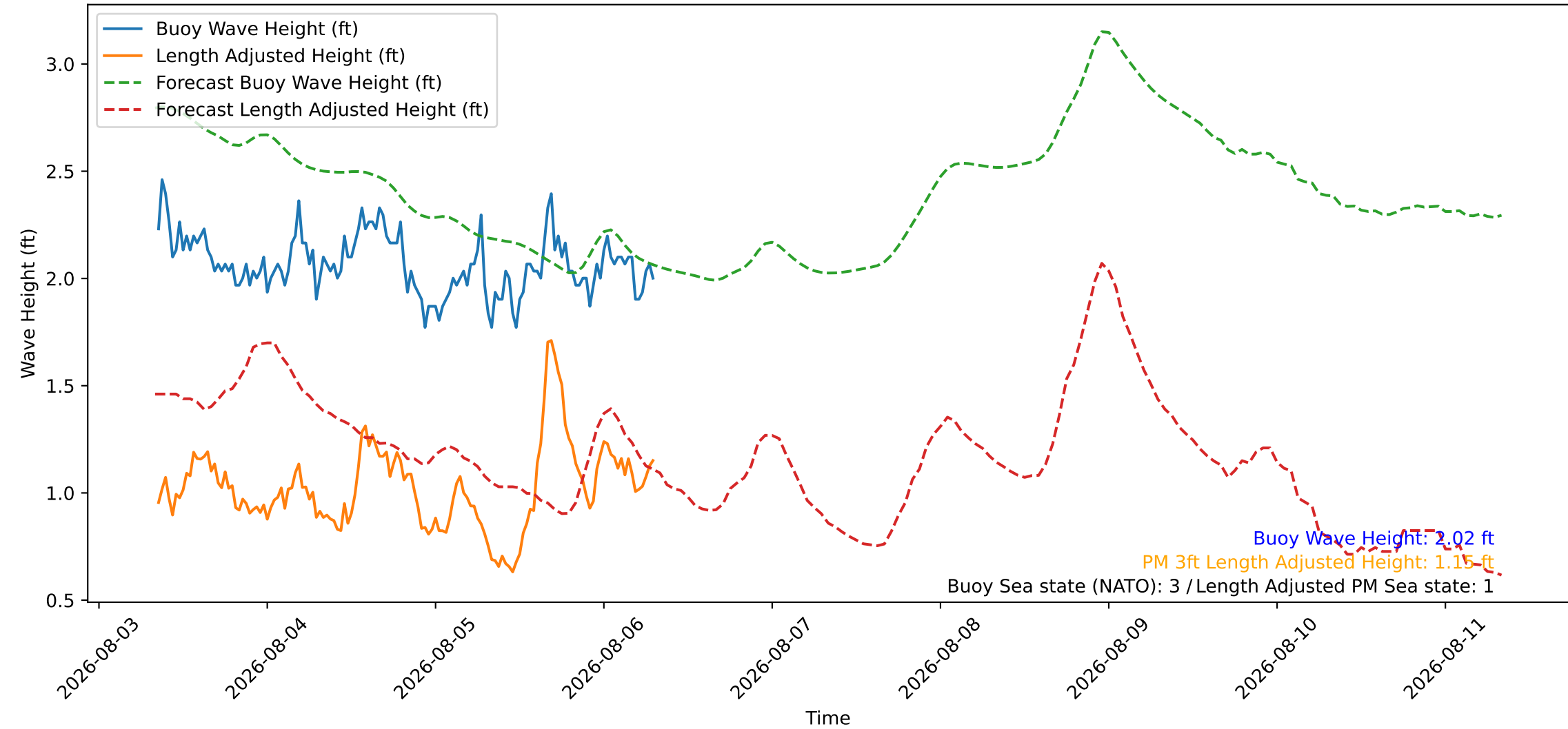
Wave Heights over Time for Red Beach at 2026-08-06 08:00:45
