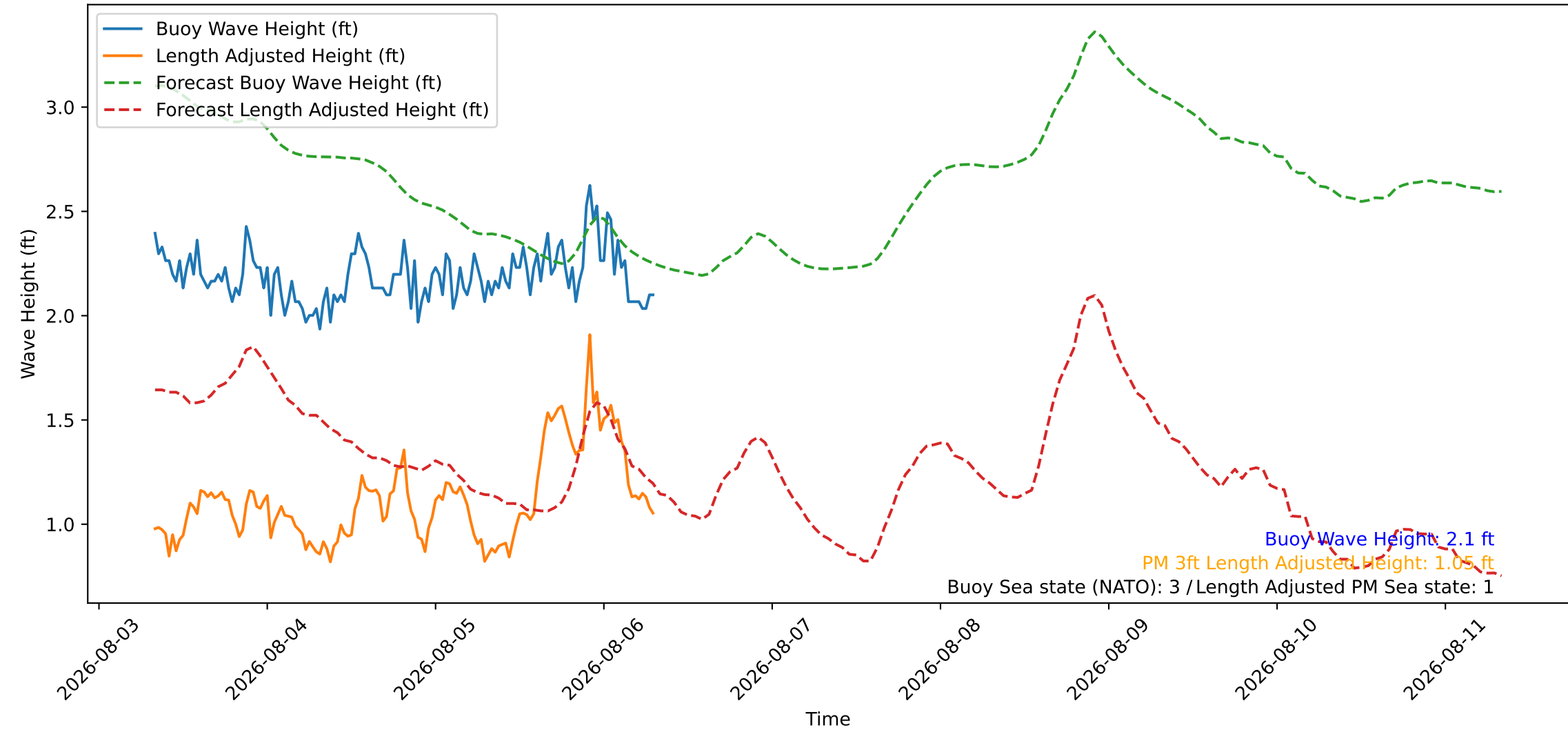
Wave Heights over Time for Green Beach at 2026-08-06 08:01:07
