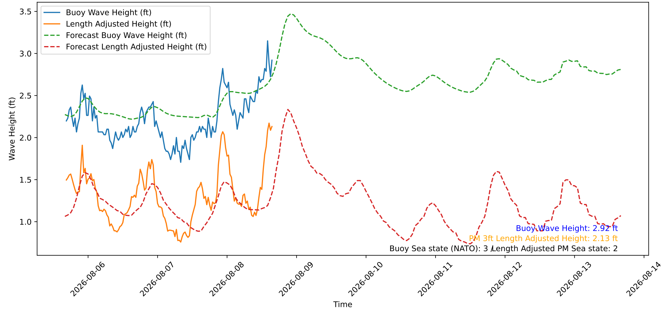
Wave Heights over Time for Green Beach at 2026-08-08 16:21:10
