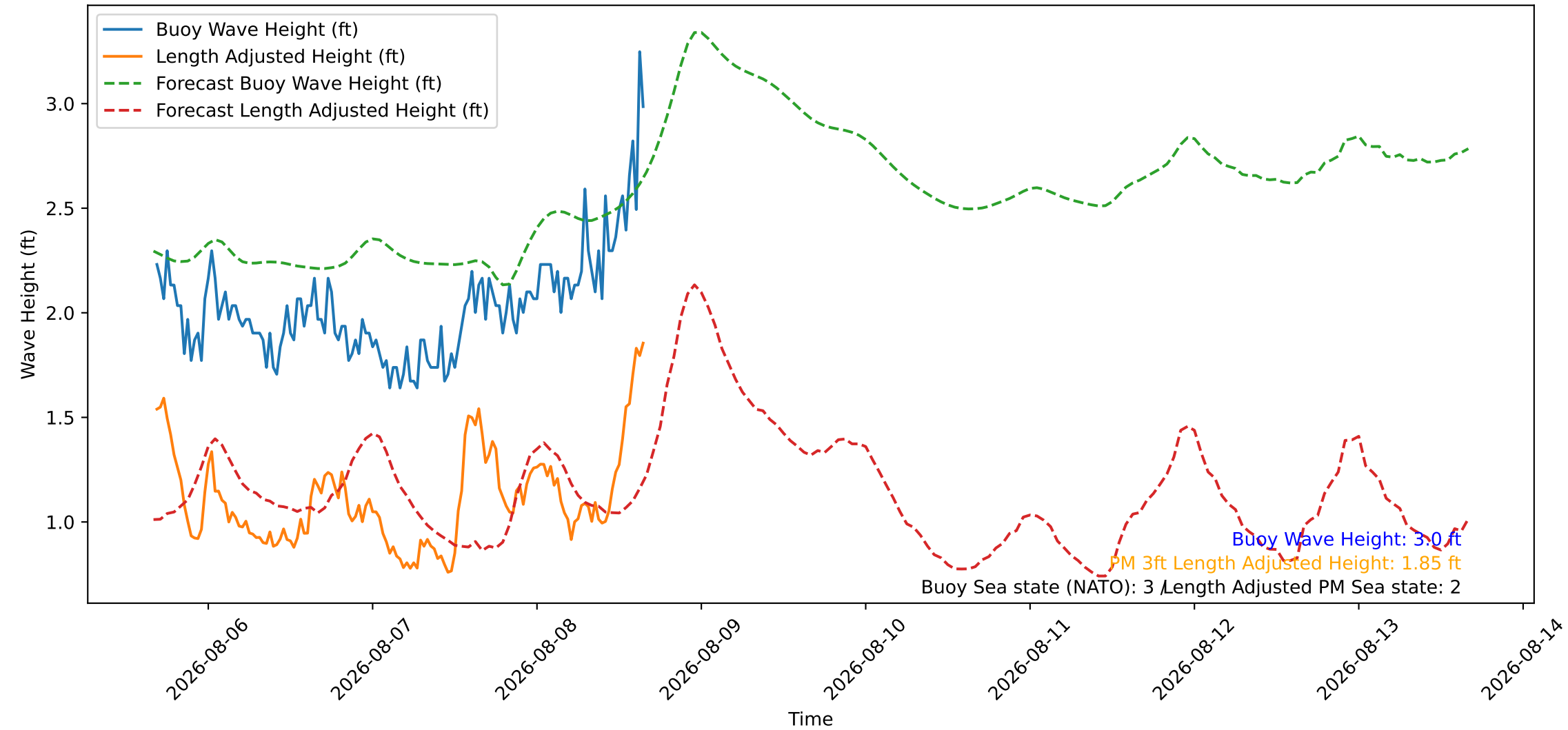
Wave Heights over Time for Oceanside Harbor at 2026-08-08 16:20:26
