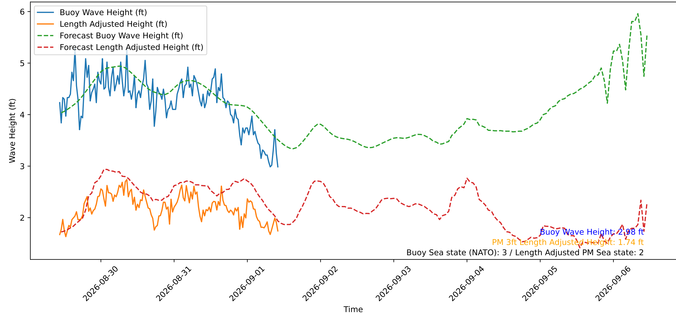
Wave Heights over Time for Oceanside Harbor at 2026-09-01 10:40:29
