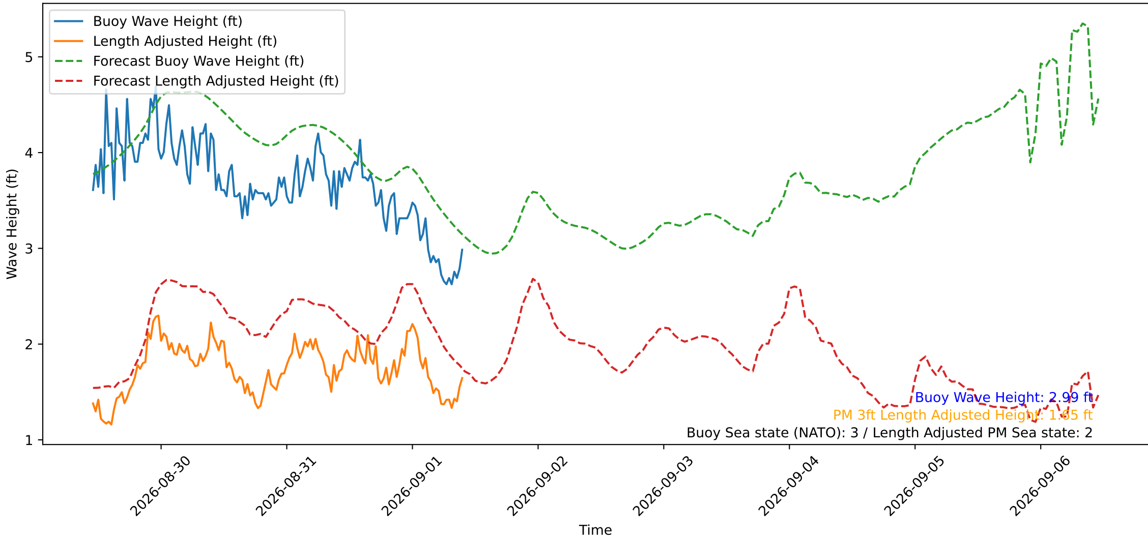
Wave Heights over Time for Red Beach at 2026-09-01 10:40:49
