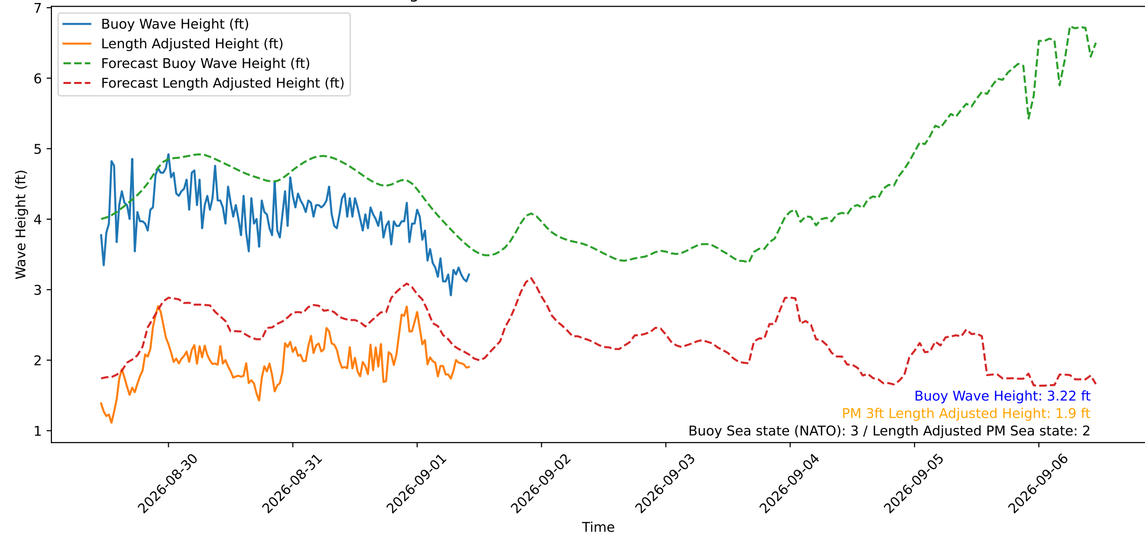
Wave Heights over Time for Green Beach at 2026-09-01 10:41:11
